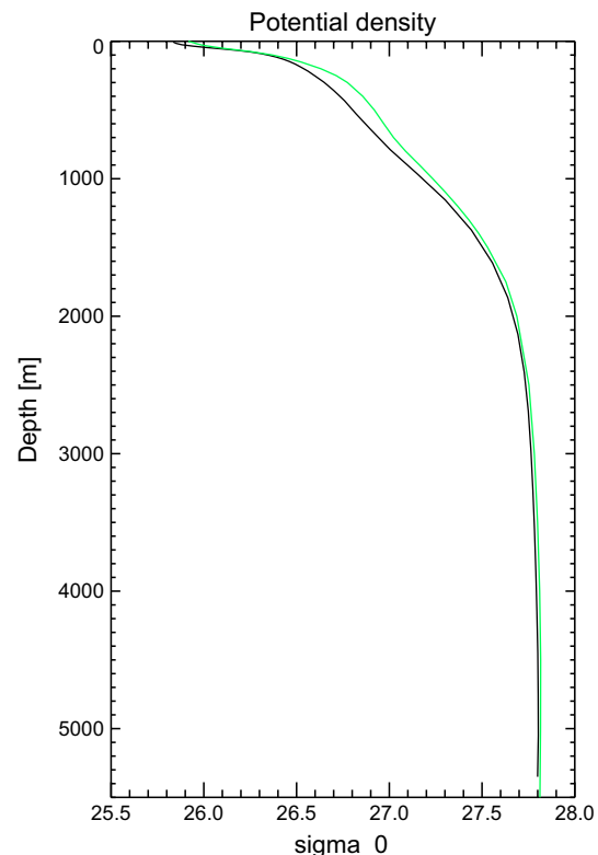
Fig. 1 Globally averaged density profile from the World Ocean Atlas 2009 (black, Locarnini et al. 2006) and the HiGEM control run (green, 20-year average)
