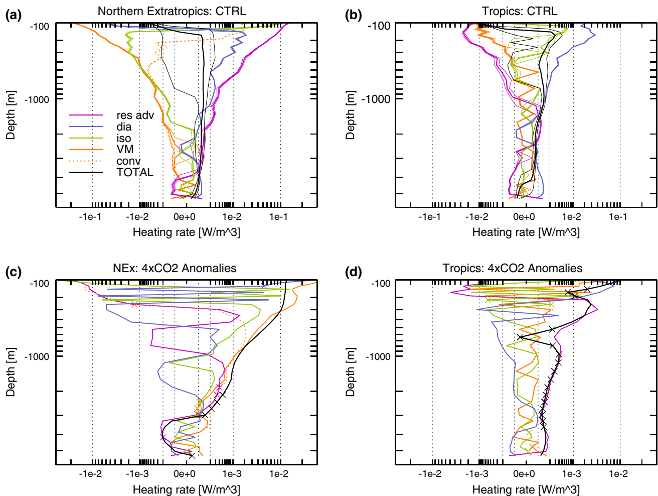
Fig. 5 Horizontally averaged temperature tendency diagnostics for a the control run in the Northern Extratropics region, b the control runs in the Tropics region, and the 4xCO 2 anomalies in c the Northern Extratropics and d the Tropics region. Both axes are stretched according to a power law to visualize both the large values in the mixed layer and the small values at depth. The dotted vertical lines denote orders of magnitude. Note the varying scales on the x-axis.
