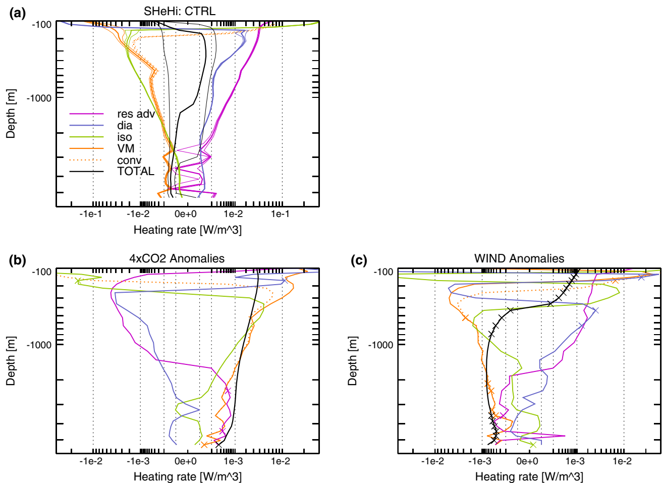
Fig. 7 Horizontally averaged temperature tendency diagnostics for the Southern Hemisphere high latitudes for a the control run, b the 4xCO 2 anomalies and c the WIND anomalies. Otherwise as Fig. 5
