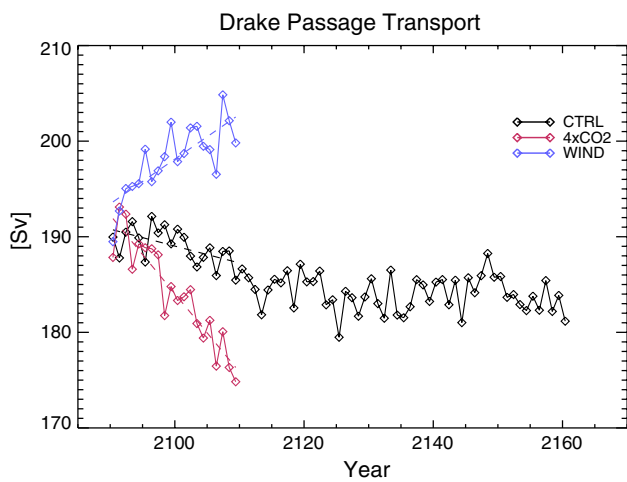
Fig. 10 Drake Passage transport in Sverdrup ( 1 \text{ Sv} = 10^6 \text{ m}^3 \text{ s}^{-1} ) in the three HiGEM1.2 runs. Dashed lines show trend estimates over 20 years
