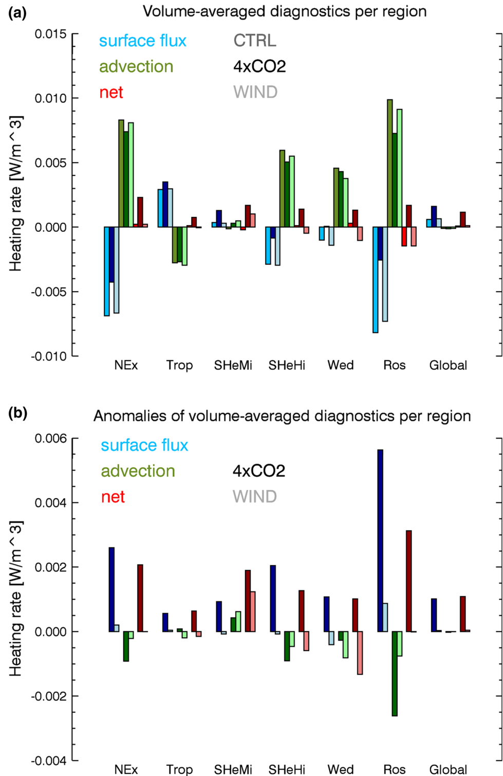
Fig. 9 Overview plot for the most relevant heat uptake processes in the regions of interest discussed in the text. The regions are defined in Sect. 4. In a each region has three groups of three bars. Each group is colour coded according to the process it represents. In each group, the main colour comes in three hues, where the first bar is for CTRL, the second for 4xCO 2 and the third for WIND. Each single bar gives the heating rate for a specific region, process and run. Panel b shows anomalies of the perturbation runs. Therefore, in each group, the main colour comes in two hues, where the first bar is for 4xCO 2 ( dark hue ) and the second for WIND ( light hue )
