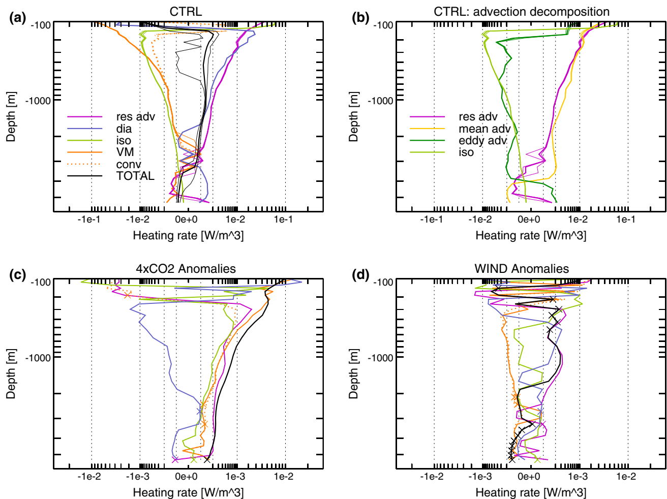
Fig. 3 The temperature tendency diagnostics as a function of depth in HiGEM1.2. Bold lines show a 70-year average from the control run and 20-year averages from the perturbation runs. The thin lines indicate a \pm 1 standard deviation interval for the control run (CTRL). They are shown for the components as well as the total, but are hardly discernible since the standard deviation is relatively small in all of the cases. Both axes are stretched according to a power law to visualize both the large values in the mixed layer and the small values at depth. Dotted black vertical lines mark orders of magnitudes. a CTRL, b
