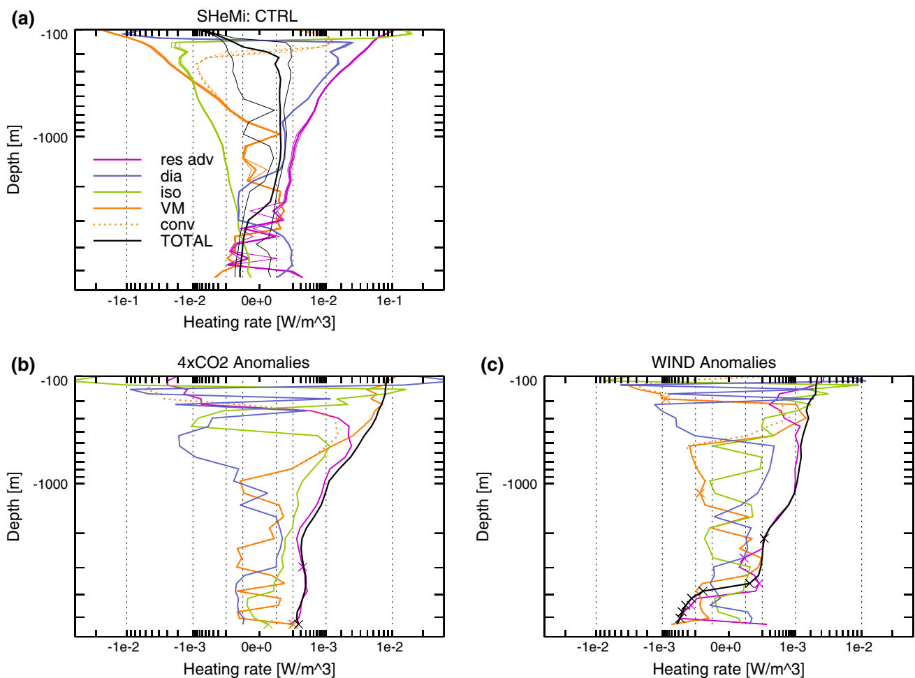
Fig. 6 Horizontally averaged temperature tendency diagnostics for the Southern Hemisphere mid-latitudes for a the control run, b the 4xCO 2 anomalies and c the WIND anomalies. Otherwise as Fig. 5
