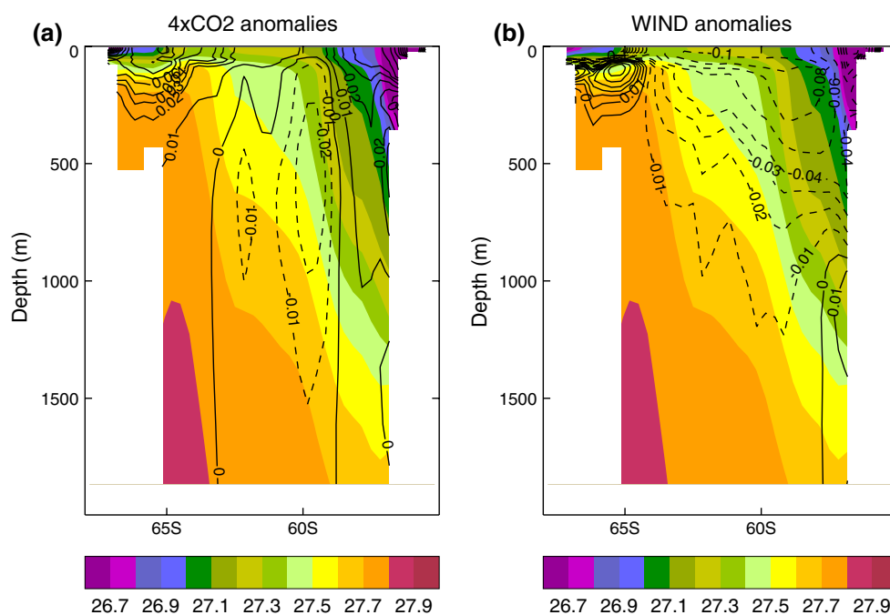
Fig. 12 Zonal average of potential density (shaded, in \sigma_2 units) and its anomaly (contours) in the Drake Passage region. a Anomalies of 4xCO 2 , b anomalies of WIND. Solid contours indicate positive den-
