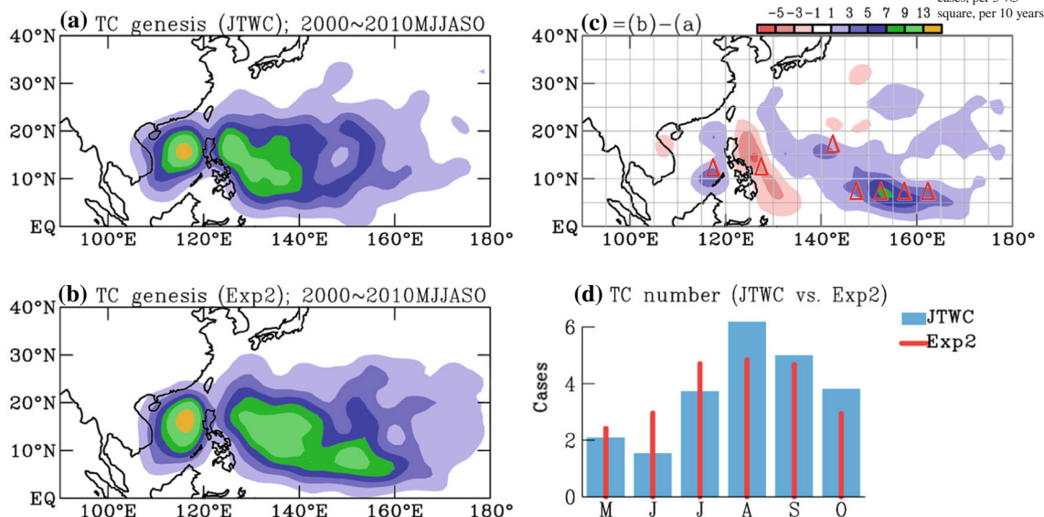
Fig. 3 As in Fig. 1, except for the comparison between the variations of TC genesis derived from the JTWC and the ensemble of Exp2 (i.e. the RegCM3 driven by CFS2 hindcast data; see Sect. 2) during 2000–2010, May–October
