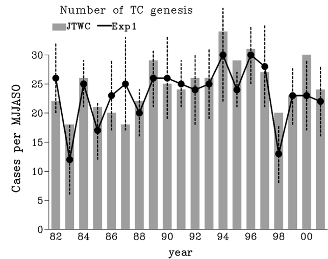
Fig. 2 Year-to-year variations of the MJJASO (May–October) TC genesis numbers over the WNP basin derived from the JTWC data (grey bar) and the outputs of Exp1 during 1982–2001 (solid line represents the ensemble mean). The spread between the ensemble members are shown by the dashed lines
