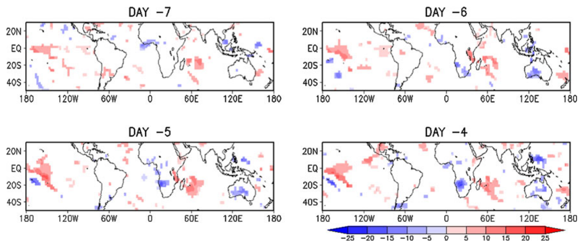
Fig. 5 Composites anomaly of outgoing longwave radiation ( Wm^{-2} , significant at the 90 % level using a student's t test)
