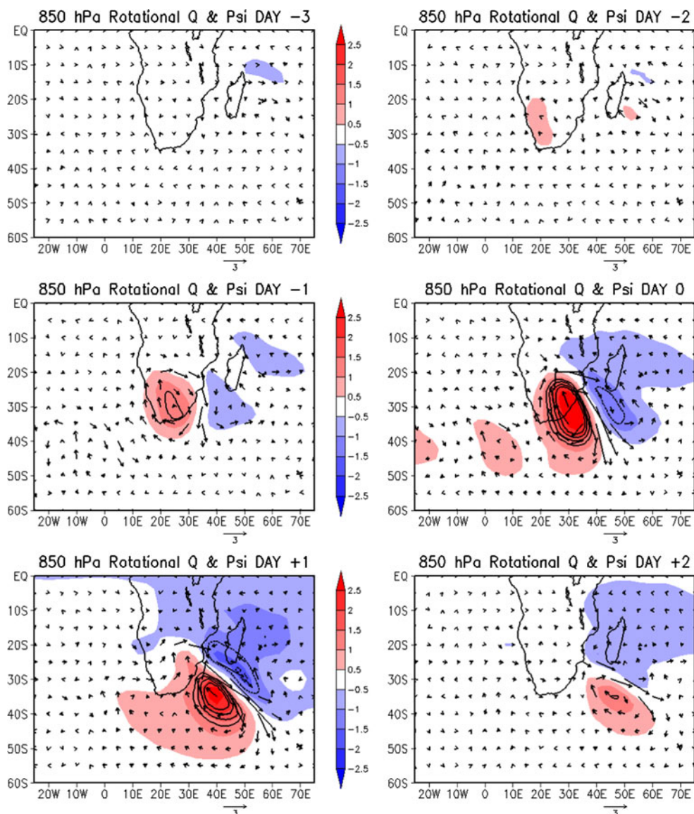
Fig. 12 Composite anomalies of 850 hPa streamfunction (shaded, significant at the 95 % level using t test are contoured, units: 1 \times 10^6 \text{ m}^2 \text{ s}^{-1} ) and rotational component of moisture transport (vectors, units: \text{gm m}^{-1} \text{ s}^{-1} )
