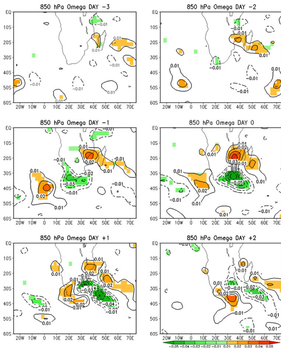
Fig. 11 Composites anomalies of 850 hPa Omega ( \text{Pa s}^{-1} , shaded values are significant at the 95 % level using a student's t test)
