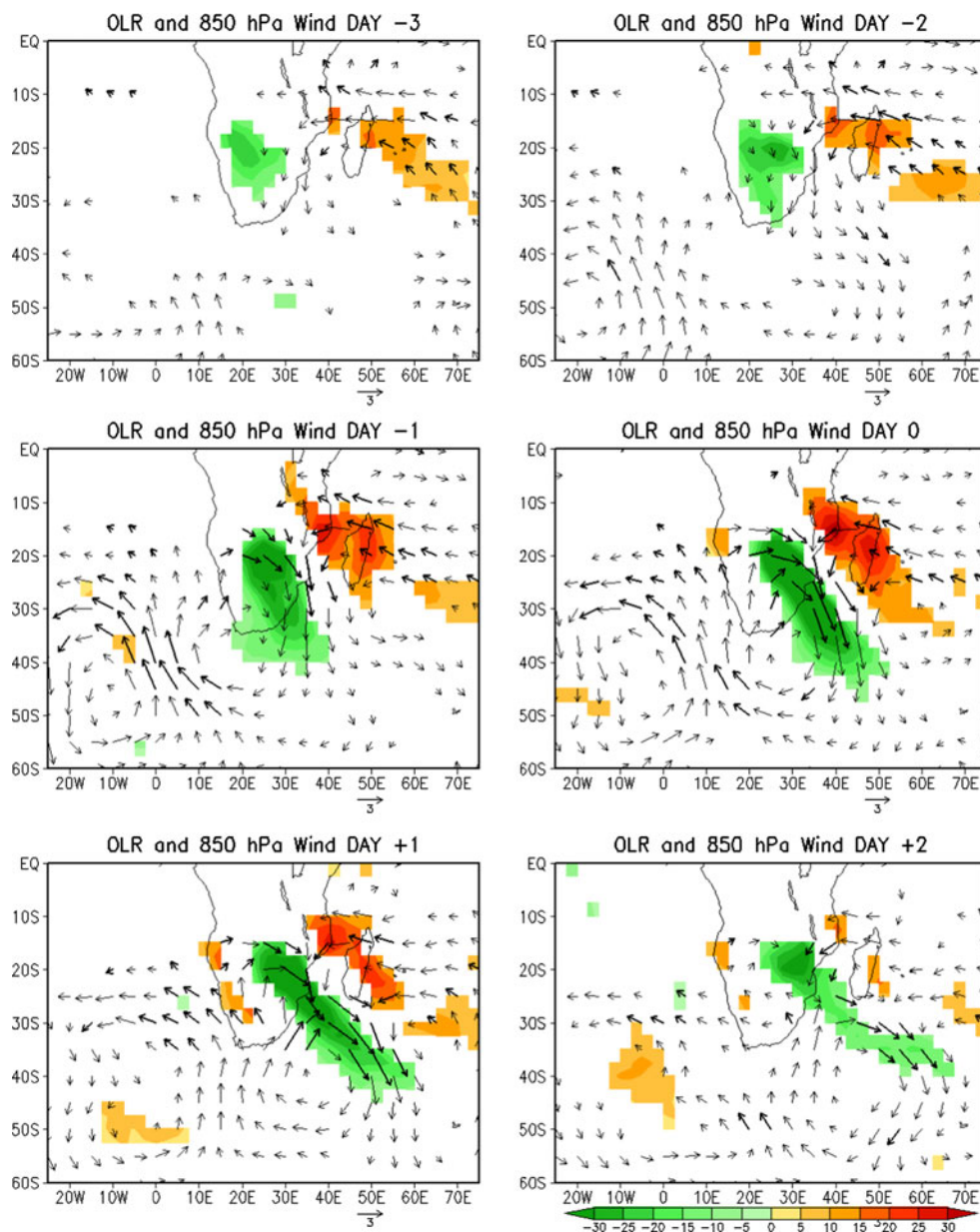
Fig. 9 Composites anomalies of OLR ( Wm^{-2} , shown values are significant at 95 % using a student's t test) and wind vectors ( m s^{-1} , thick arrows are significant at the 90 % level using a student's t test)
