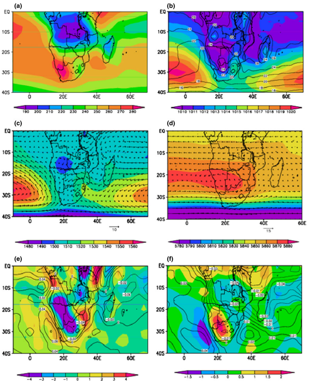
Fig. 1 December–January–February (DJF) climatology of a outgoing longwave radiation ( \text{Wm}^{-2} ), b sea level pressure (shaded, hPa) and surface temperature (contour, degree C), c 850 hPa geopotential
