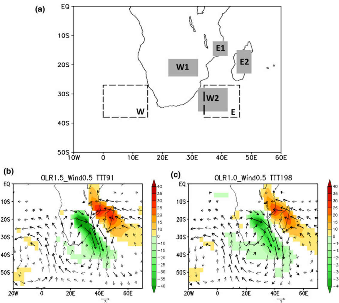
Fig. 2 a Various regions chosen for identifying the index. Filled rectangle boxes (E1, E2, W1 and W2) are used for OLR and dashed rectangular boxes (W and E) are used for wind. b Composite structure
