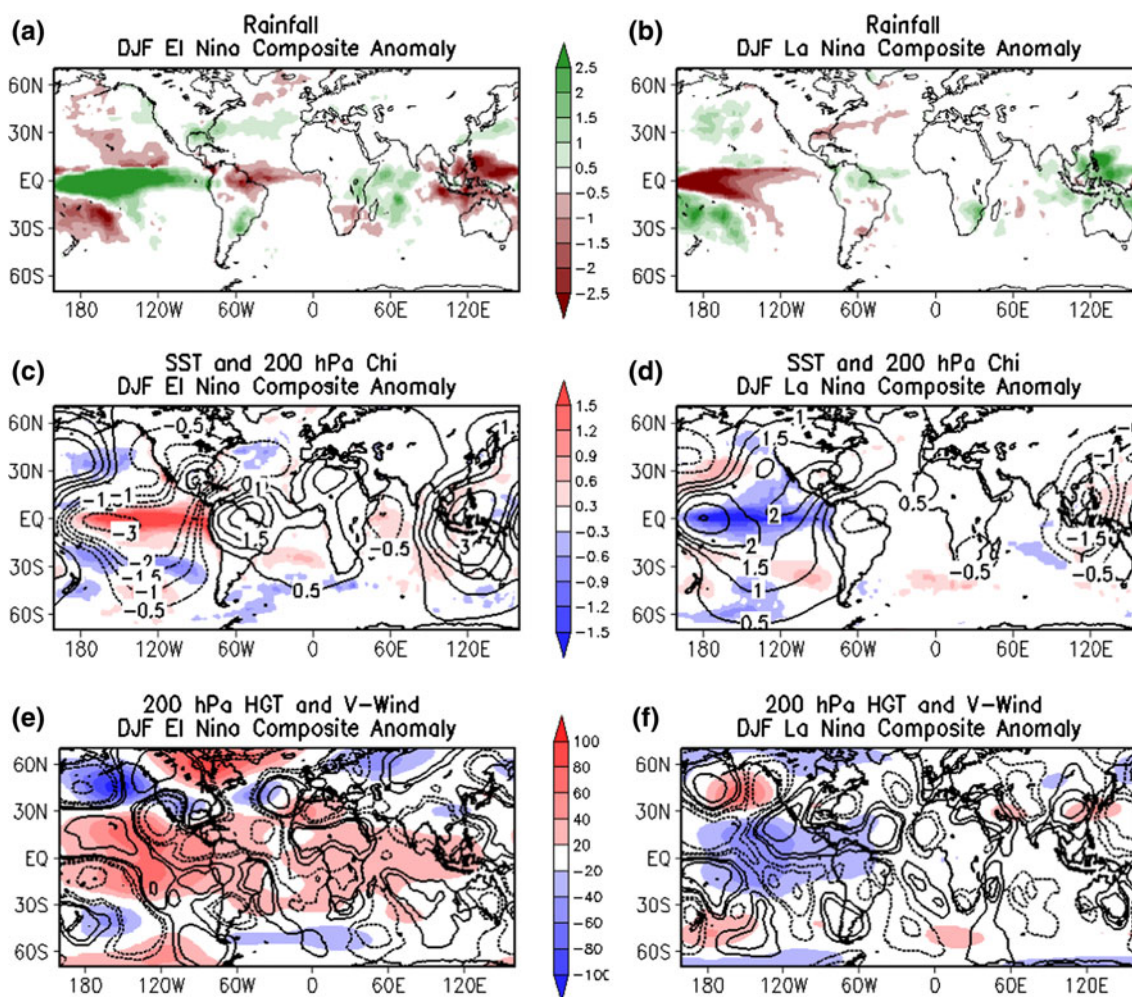
Fig. 16 DJF composite anomalies of rainfall (mm/day) (a, b), sea surface temperature (K, shaded) and 200 hPa velocity potential ( 10^6 \text{ m}^2 \text{ s}^{-1} , contour) (c, d), 200 hPa geopotential height (m, shaded)
