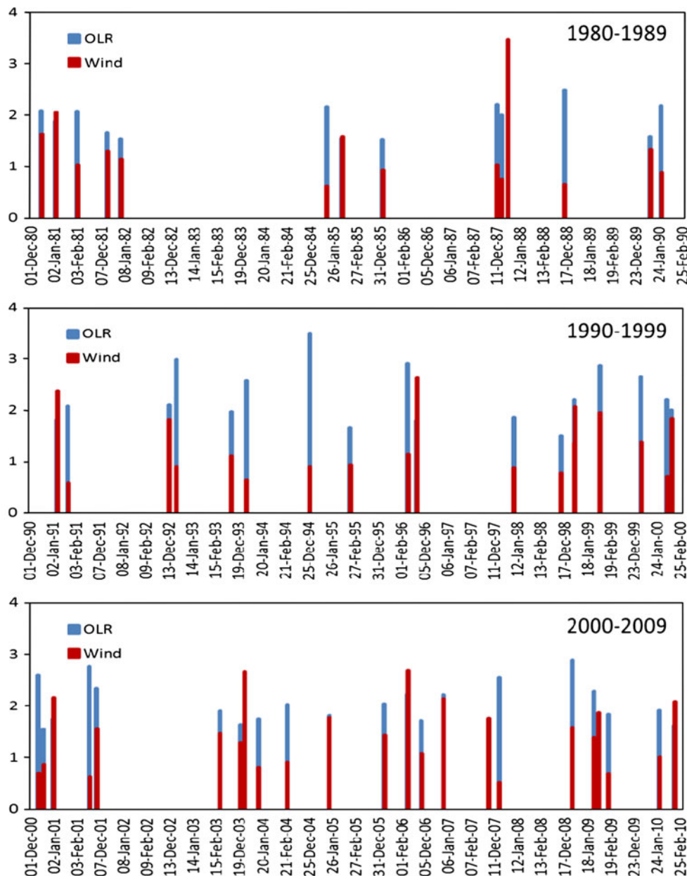
Fig. 4 Standardized anomaly of OLR and winds for the 55 strong TTT events during the period 1980–2009 (the anomalies for remaining days are suppressed for the clarity of those 55 events)
