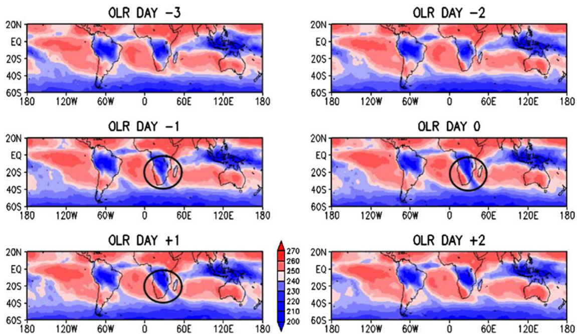
Fig. 15 Composites of outgoing longwave radiation ( \text{Wm}^{-2} )
