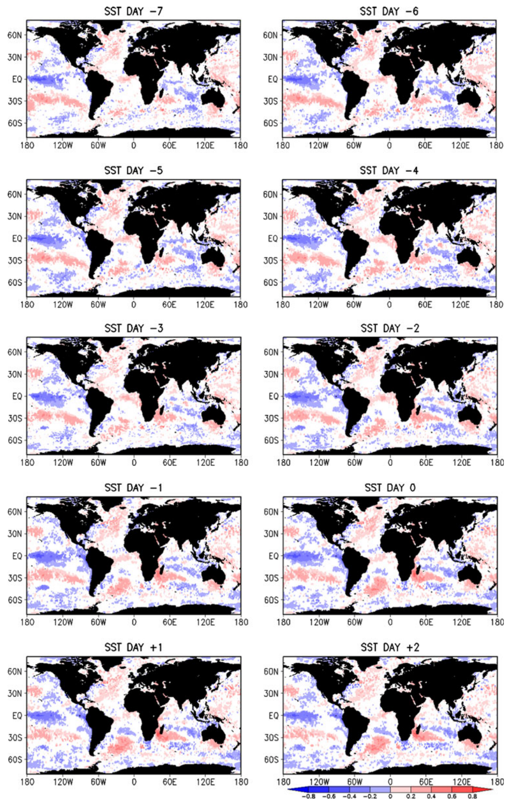
Fig. 8 Composites anomalies of sea surface temperature (K). Shown values are significant at the 90 % level using a student's t test
