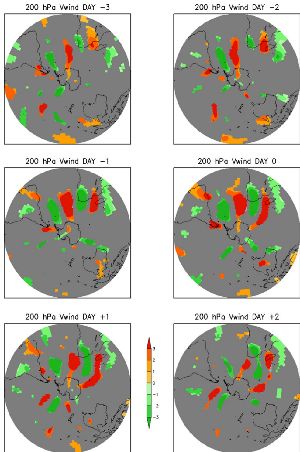
Fig. 14 Composite anomalies of 200 hPa meridional winds ( \text{m s}^{-1} , shown values are significant at the 90 % level using a student's t test)
