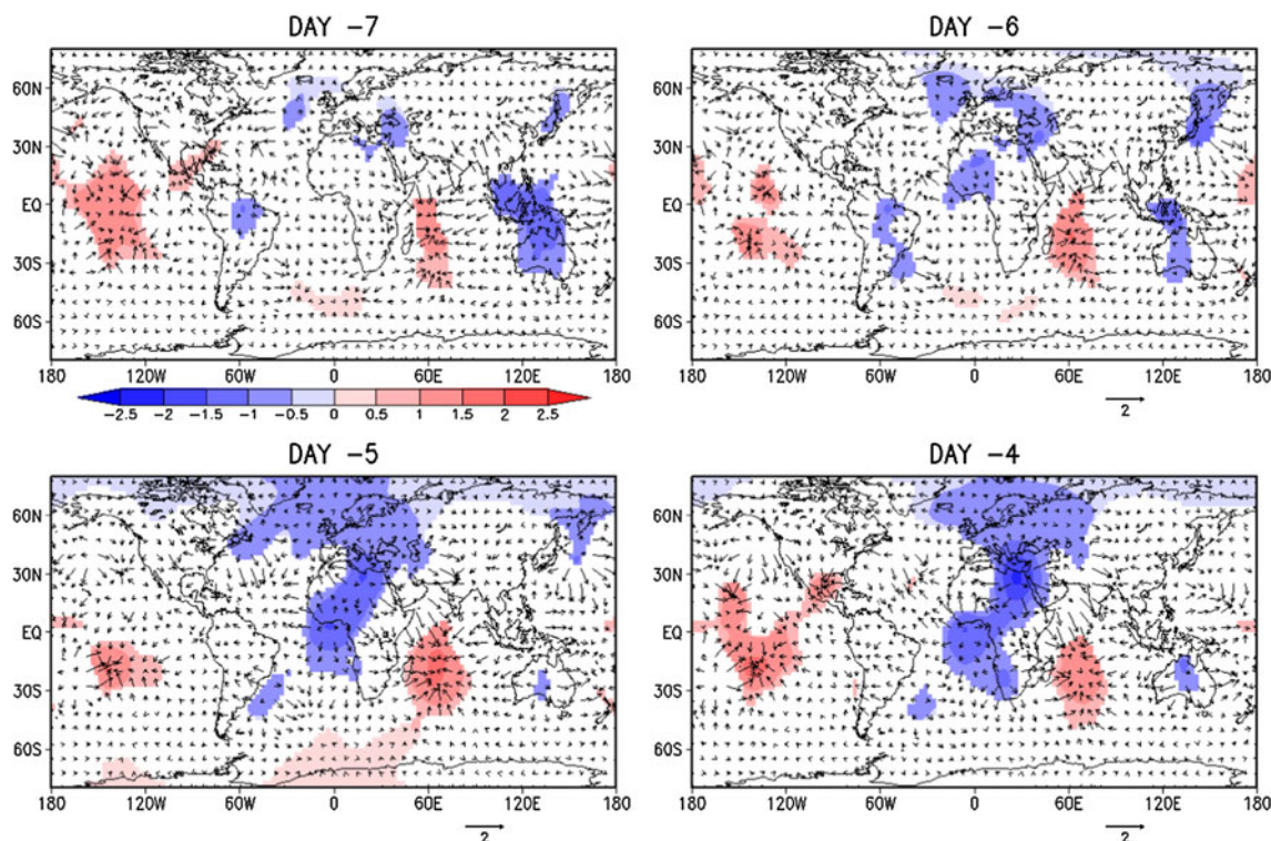
Fig. 6 Composite anomalies of 200 hPa velocity potential ( shaded ). Values are significant at the 90 % level using a student's t test and the units are 1 \times 10^6 \text{ m}^2 \text{ s}^{-1} . Divergent component of the winds (vectors, units: \text{m s}^{-1} ) are overlaid
