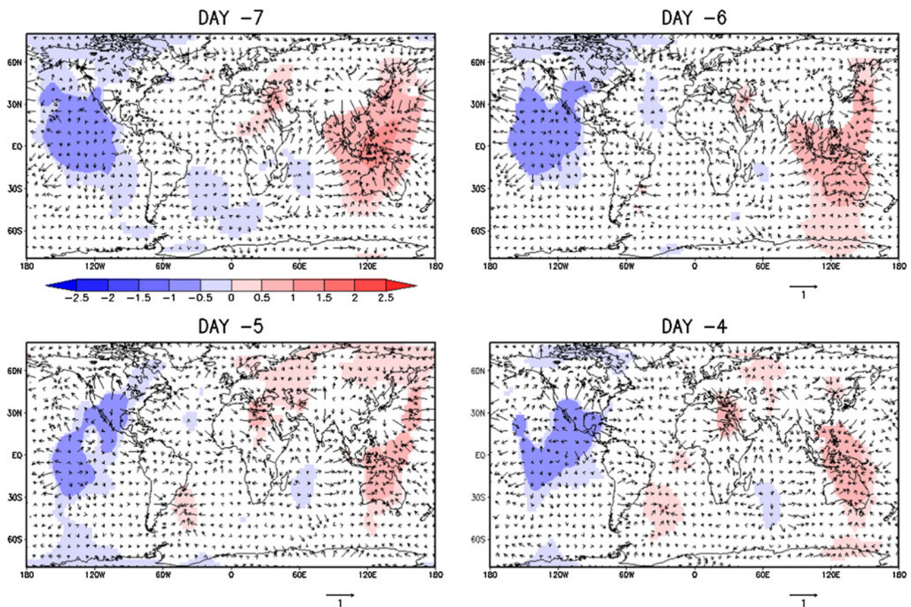
Fig. 7 Composite anomalies of 850 hPa velocity potential ( shaded ). Values are significant at the 90 % level using a student's t test and the units are 1 \times 10^6 \text{ m}^2 \text{ s}^{-1} . Divergent component of the winds (vectors, units: \text{m s}^{-1} ) are overlaid
