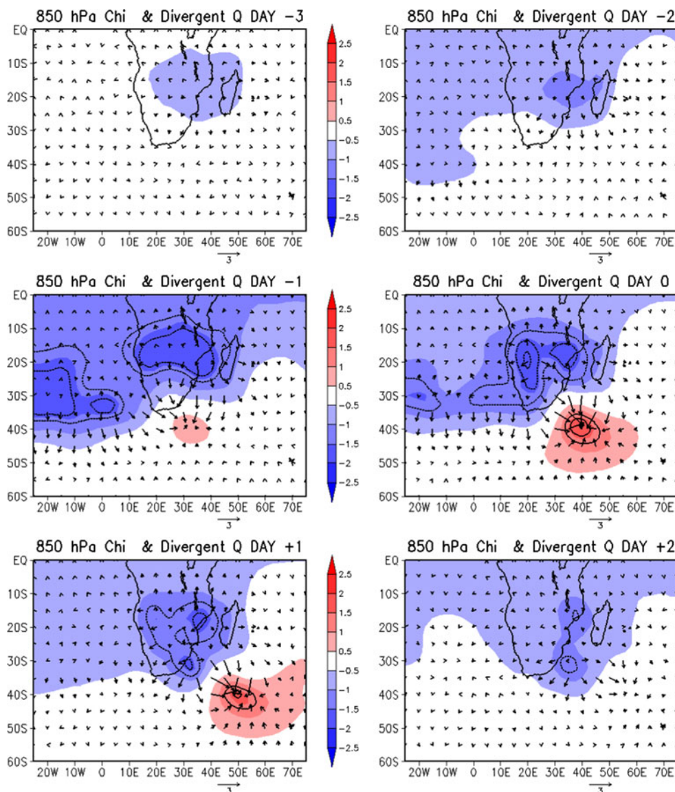
Fig. 13 Composite anomalies of 850 hPa velocity potential (shaded, significant at the 95 % level using t test is contoured, units: 1 \times 10^6 \text{ m}^2 \text{ s}^{-1} ) and divergent component of moisture transport (vectors, units: \text{gm m}^{-1} \text{ s}^{-1} )
