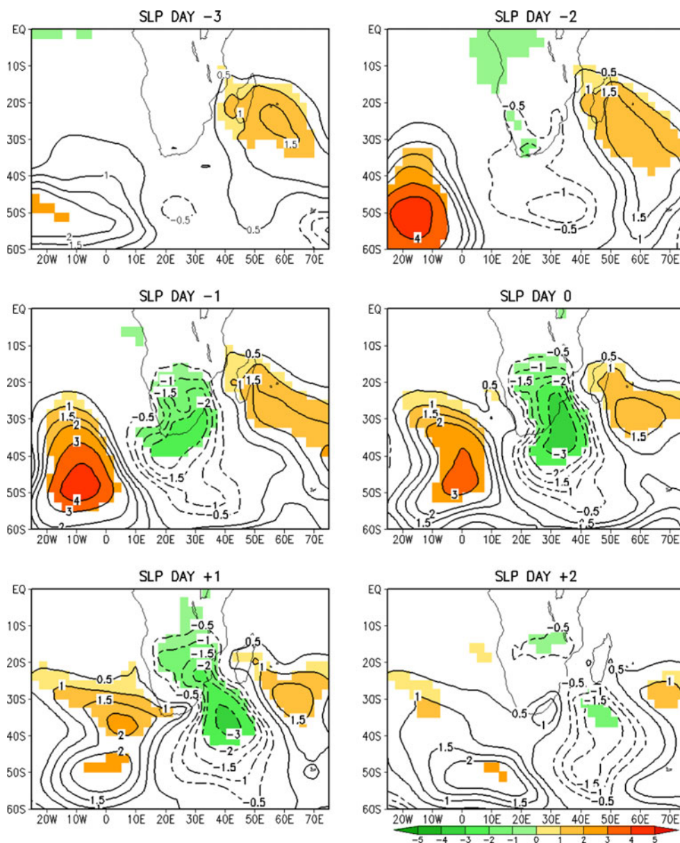
Fig. 10 Composites anomalies of sea level pressure (hPa, shaded values are significant at the 95 % level using a student's t test)
