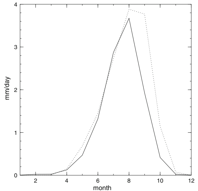
Fig. 1 Annual cycle of precipitation averaged over the west Sahel (mm/day). The west Sahel index is computed over the region from 15^{\circ}W to 10^{\circ}E and from 12^{\circ}N to 20^{\circ}N . The solid curve shows the observed seasonal cycle and the dotted curve the simulated seasonal cycle by ECHAM5. The observation is based on the CRU data-set and the simulated is based on our control integration. For better comparison the seasonal cycle for the observations is computed over the period 1979–1995
