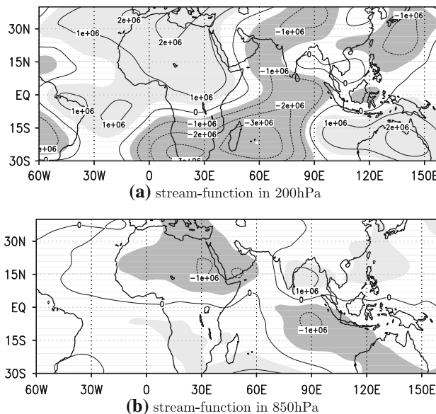
Fig. 11 The summer JAS 200hPa and 850hPa stream-function anomaly patterns ( m^2/s ) for the Indian Ocean experiment. Shown are the simulated anomalies relative to the control integration forced by climatological SSTs. Light shading indicates anomalies exceeding 5 \times 10^5 and dark shading represents anomalies lower than -5 \times 10^5
