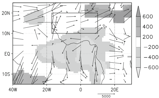
Fig. 10 Response in simulated vertically integrated specific humidity (precipitable water) in kg/m^2 and vertically integrated humidity flux in mg/(skg) for the Atlantic experiment. Shown are anomalies relative to the control integration forced by climatological SSTs. Only significant changes in precipitable water at the 95% significance level according to a two-tailed t test are shaded. The vectors show the response in the vertically integrated humidity flux
