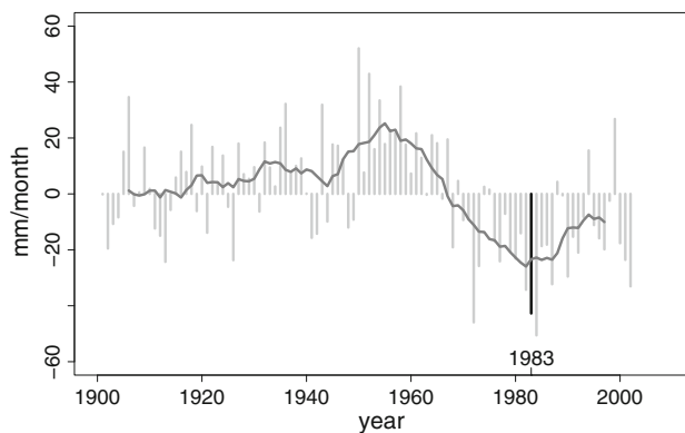
Fig. 3 observed summer (JAS) rainfall anomaly over the western Sahel (see text for details) based on the CRU data-set (mm/month). Grey bars indicate seasonal means, the line the 11-year running mean of the summer rainfall and the black bar indicates the rainfall anomaly in the year 1983
