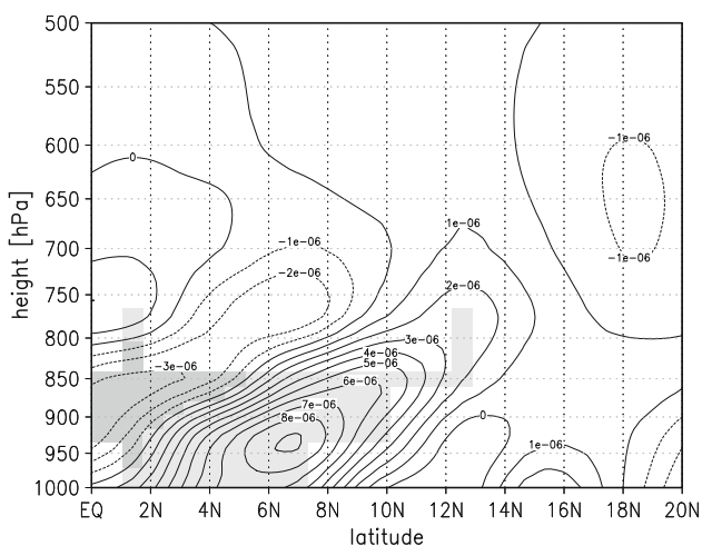
Fig. 9 Height-latitude cross-section of the response in simulated horizontal moisture divergence averaged from 15°W to 10°E for the Atlantic experiment [g/(kg s)]. Shown are anomalies relative to the control integration forced by climatological SSTs. Only significant changes in horizontal moisture divergence at the 95% significance level according to a two-tailed t test are shaded. Dashed contours represent negative values of the horizontal moisture divergence and solid lines positive: dashed curves mean moisture convergence and solid moisture divergence
