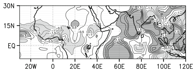
Fig. 4 Observed JAS precipitation anomaly during 1983 relative to the climatological mean (1979–1996), based on the CMAP data-set (mm/day)
