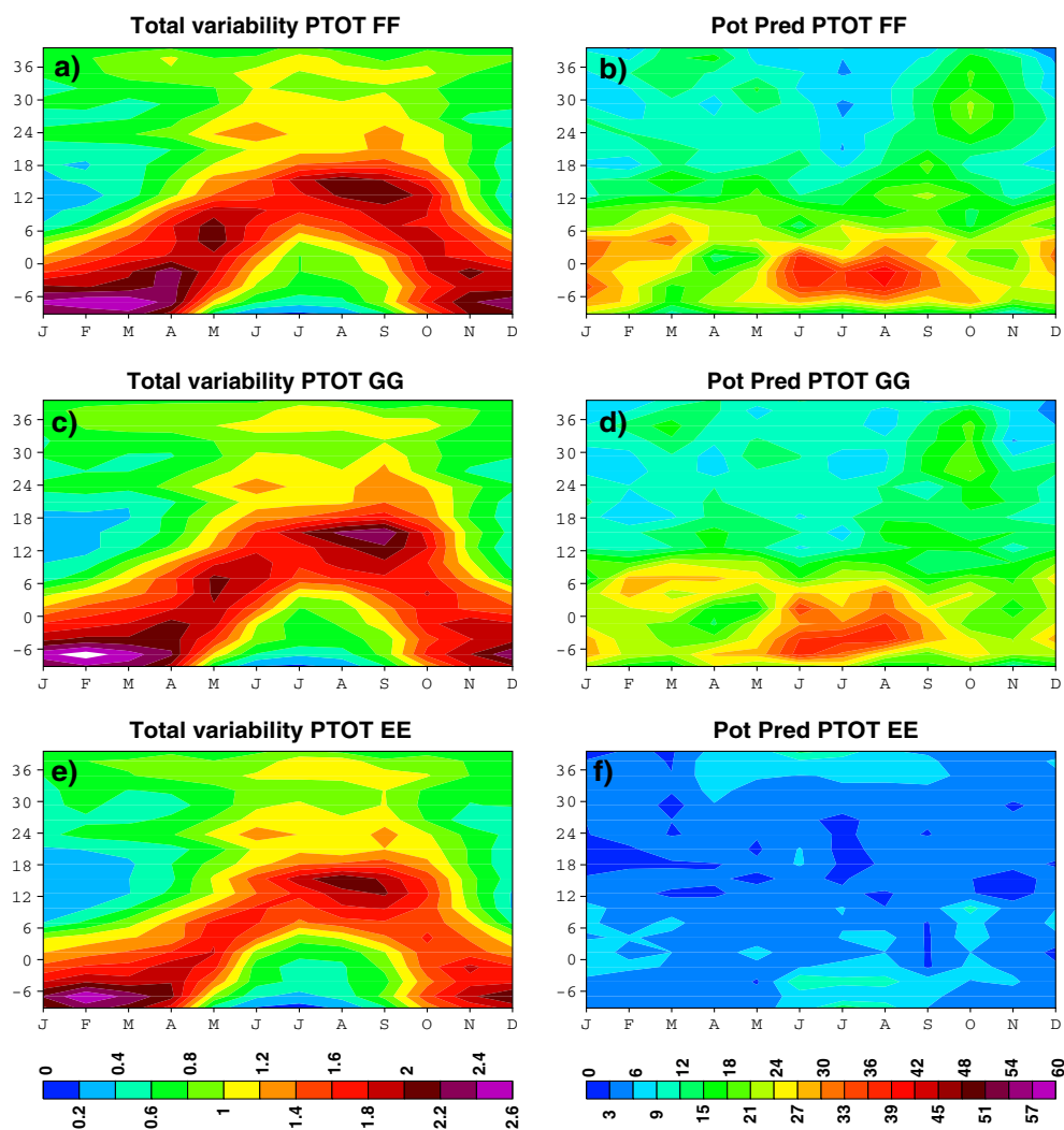
Fig. 10 Same as Fig. 9, but for precipitation
