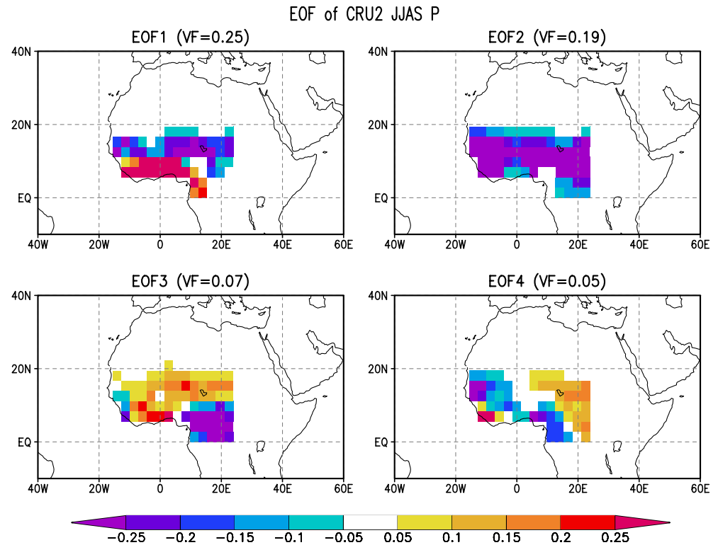
Fig. 3 Leading spatial patterns ( EOFs ) of filtered JJAS precipitation anomalies over West Africa based on the CRU2 climatology over the 1911–1992 period. VF is the fraction of variance explained by each EOF
