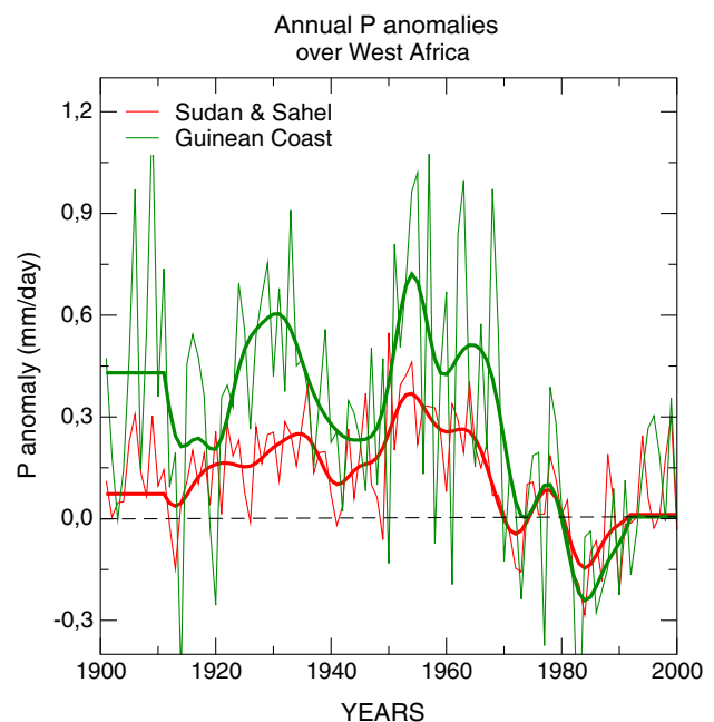
Fig. 1 CRU2 annual anomalies of Sudan-Sahel ( in red ) and Guinean Coast ( in green ) rainfall indices (see text for the definition) relative to the 1971–2000 climatology. Thick lines represent low-pass filtered anomalies using a digital filter with a 10-year frequency cutoff
