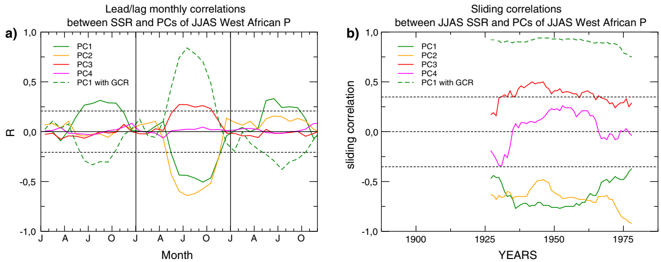
Fig. 5 a Lead–lag correlations of the leading PCs of JJAS West African rainfall in year 0 with monthly anomalies in SSR (as well as GCR for the first PC ) from year –1 to year +1. Note that the monthly timeseries have been filtered with a 5-month moving average to smooth the correlations that have been estimated over the 1911–1992 period. b Thirty-one years sliding correla-
