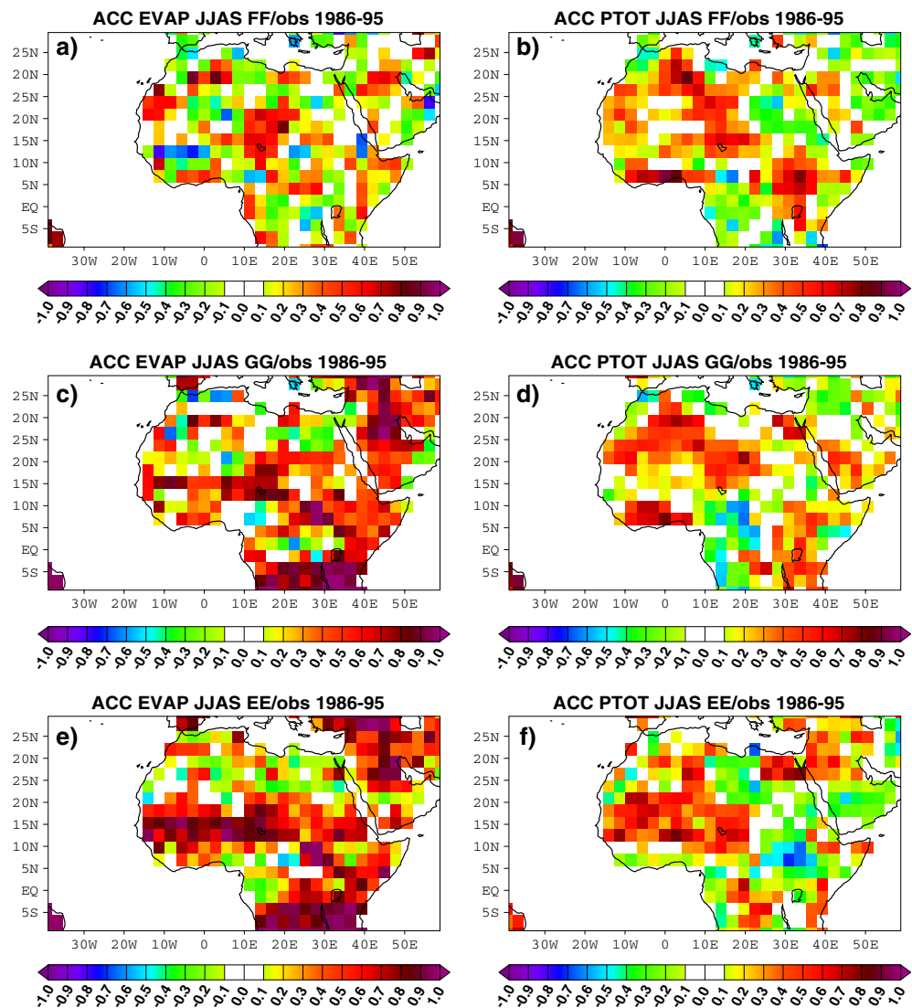
Fig. 11 Regional maps of temporal anomaly correlation coefficients ( ACC ) between simulated and analysed (GSWP2) or observed (CRU2) JJAS anomalies over the 1986–1995 period for surface evaporation ( left panels ) and precipitation ( right panels ), respectively
