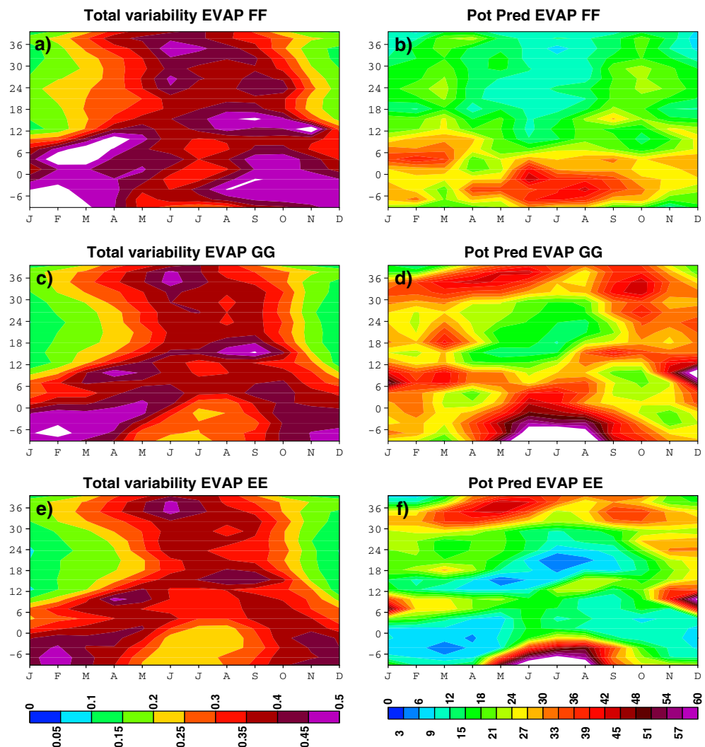
Fig. 9 Annual cycle of zonal mean (20°W–25°E) total variability (left panels in mm/day) and potential predictability (right panels in %) of surface evaporation over West Africa (land grid points only) between 10°S and 40°N
