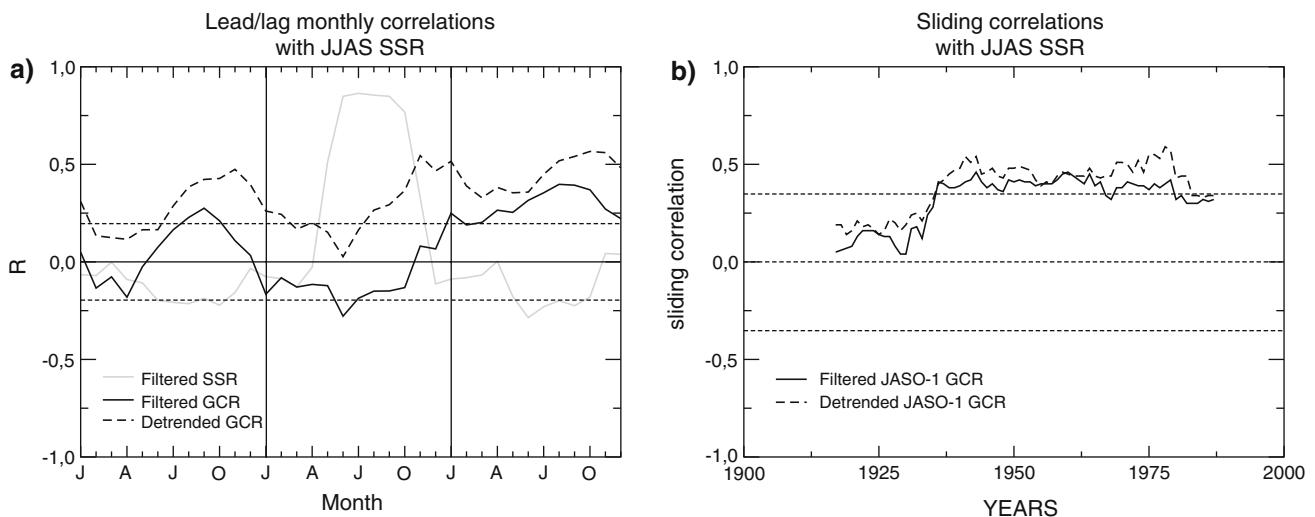
Fig. 7 a Lead–lag correlations between JJAS SSR in year 0 and monthly GCR anomalies from year -1 to year +1 (also shown are the auto-correlations with the filtered SSR timeseries). Note that the monthly timeseries have been filtered with a 5-month moving average to smooth the correlations that have been estimated
