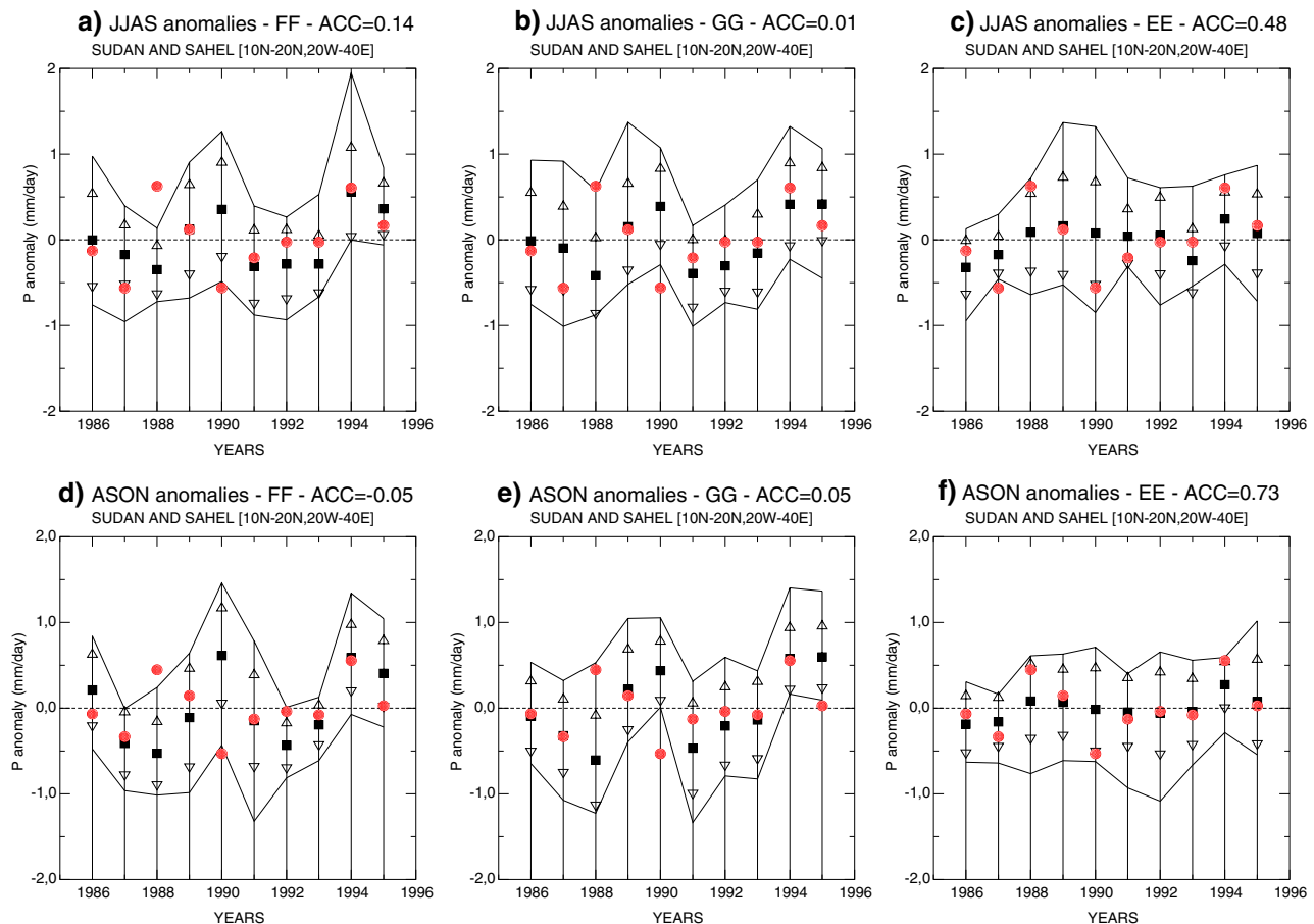
Fig. 13 Same as in Fig. 12, but for precipitation (SSR)
