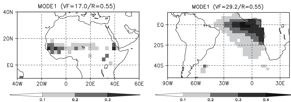
Fig. 15 First mode of a maximum covariability analysis applied to JASO southern tropical Atlantic SSTs in year 0 and JJAS West African rainfall in year +1 (filtered data over the 1911–1992 period). Left : JJAS rainfall heterogeneous vector (mm/day). Right : JASO SST homogeneous vector (K). This first pair of
