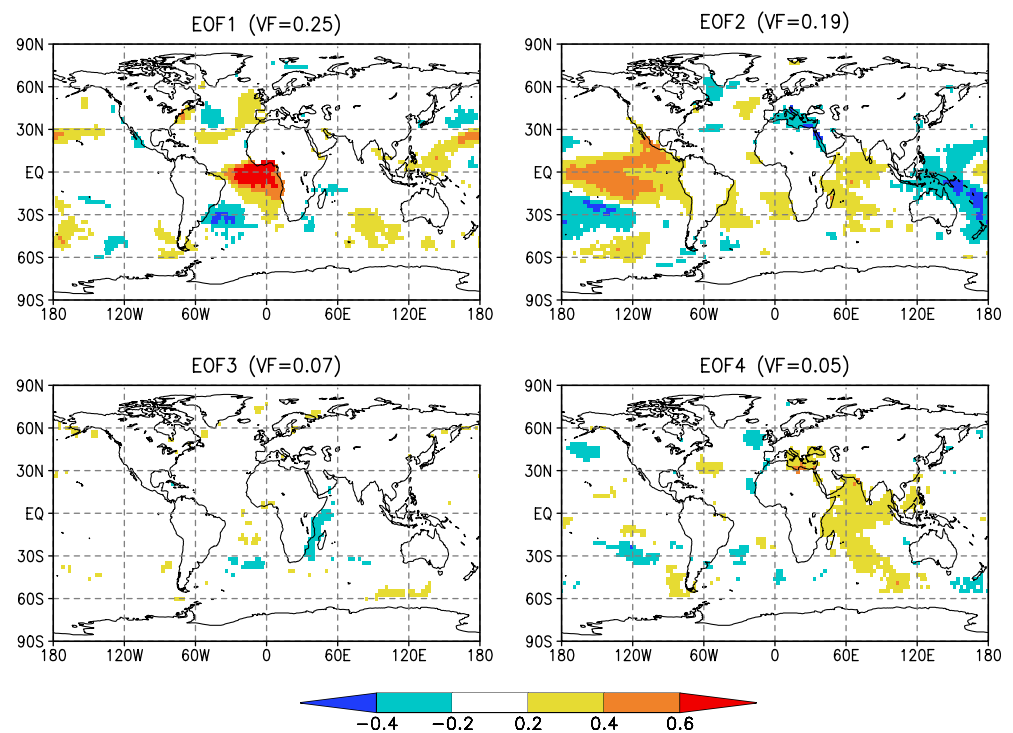
Fig. 4 Global correlation maps between the leading PCs of JJAS West African rainfall and JJAS grid-cell SST anomalies (detrended and filtered) from the HadSST.1 climatology. The correlations are estimated over the 1911–1992 period. VF is the fraction of variance explained by each EOF
