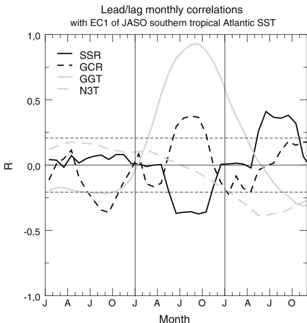
Fig. 16 Lead–lag correlations of the first EC of JASO southern tropical Atlantic SSTs from the MCA shown in Fig. 15 with monthly anomalies in SSR and GCR ( in black ), as well as with monthly SST anomalies ( in grey ) over the Guinean Gulf ( 5^{\circ}\text{S} – 5^{\circ}\text{N}/30^{\circ}\text{W} – 10^{\circ}\text{E} ) and the Niño-3 domain ( 5^{\circ}\text{S} – 5^{\circ}\text{N}/30^{\circ}\text{W} – 10^{\circ}\text{E} ). Note that the monthly timeseries have been filtered with a 5-month moving average to smooth the correlations that have been estimated over the 1911–1992 period. The 5% significance level of correlations is indicated by dashed horizontal lines
