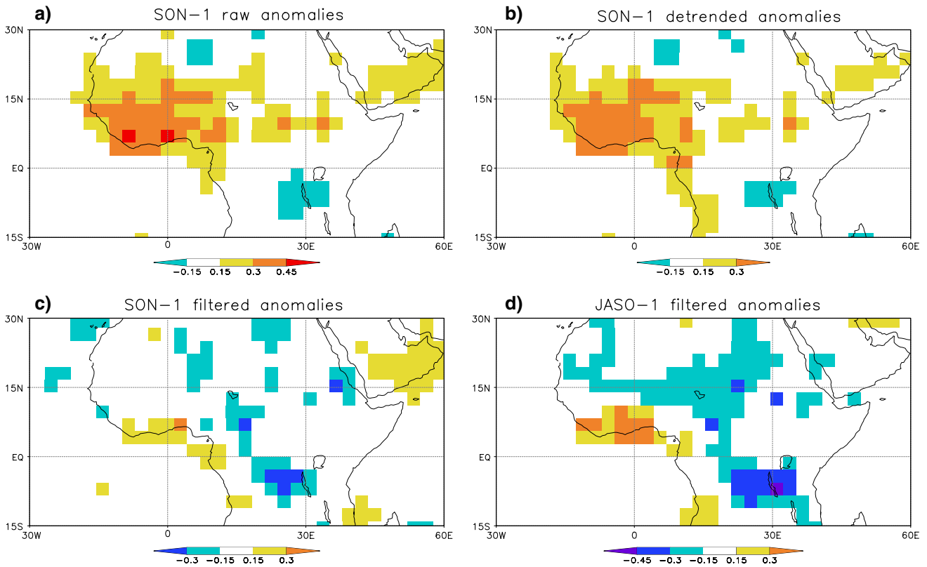
Fig. 6 Regional correlation maps between JJAS SSR in year 0 and SON ( a–c ) or JASO ( d ) grid-cell precipitation anomalies in year –1: a raw anomalies, b detrended anomalies, c , d high-pass
