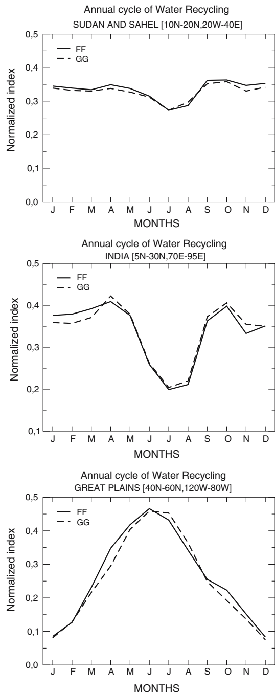
Fig. 14 Annual cycle of regional water vapour recycling ratio (see the text for details) in the FF and GG experiments over three regions, including sub-Saharan Africa ( top panel ), highlighted as “hot spots” in the GLACE intercomparison project
