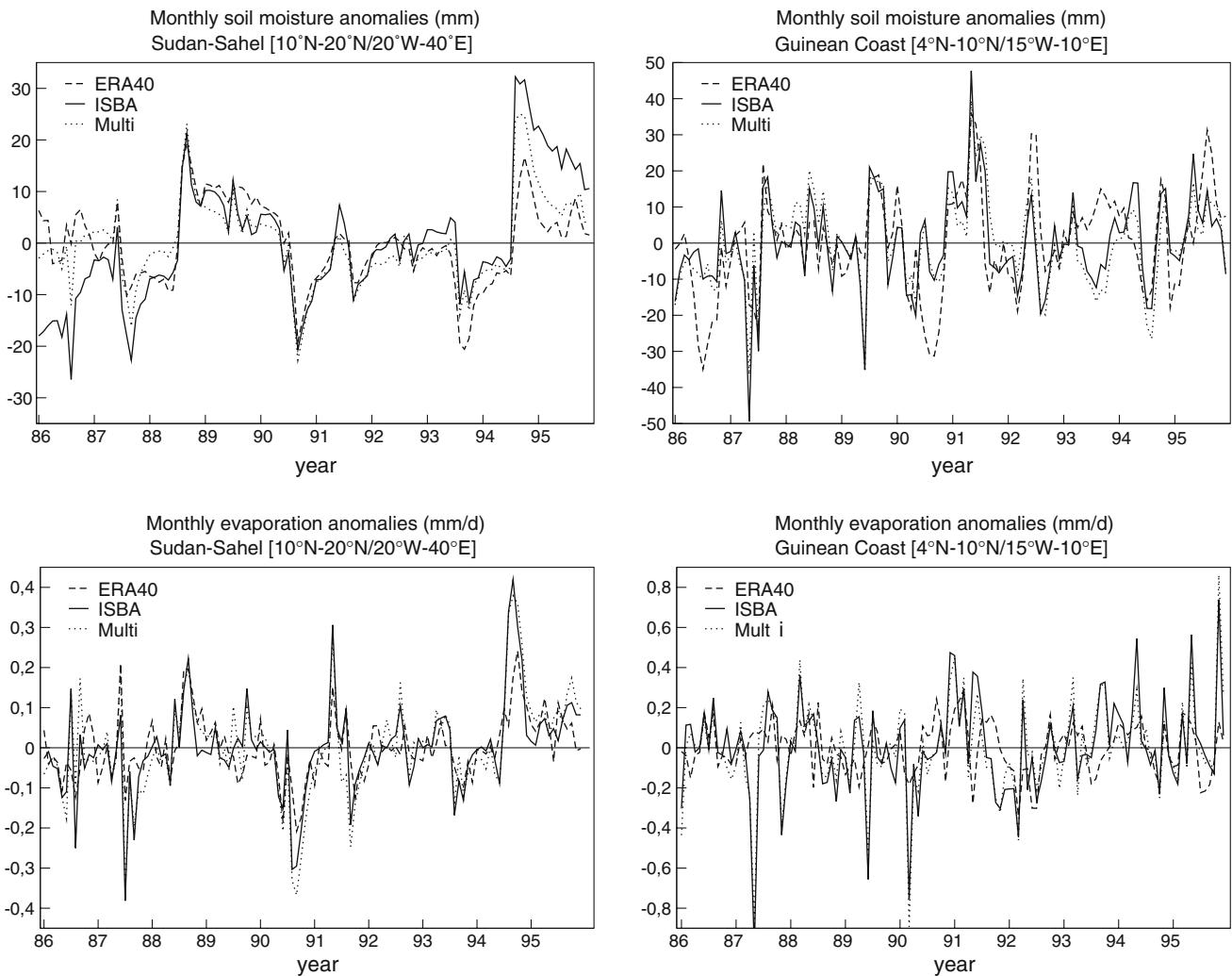
Fig. 2 Monthly anomalies of SM ( upper panels ) and surface evaporation ( lower panels ) relative to the 1986–1995 climatology over sub-Saharan Africa ( left panels ) and the Guinean Coast
