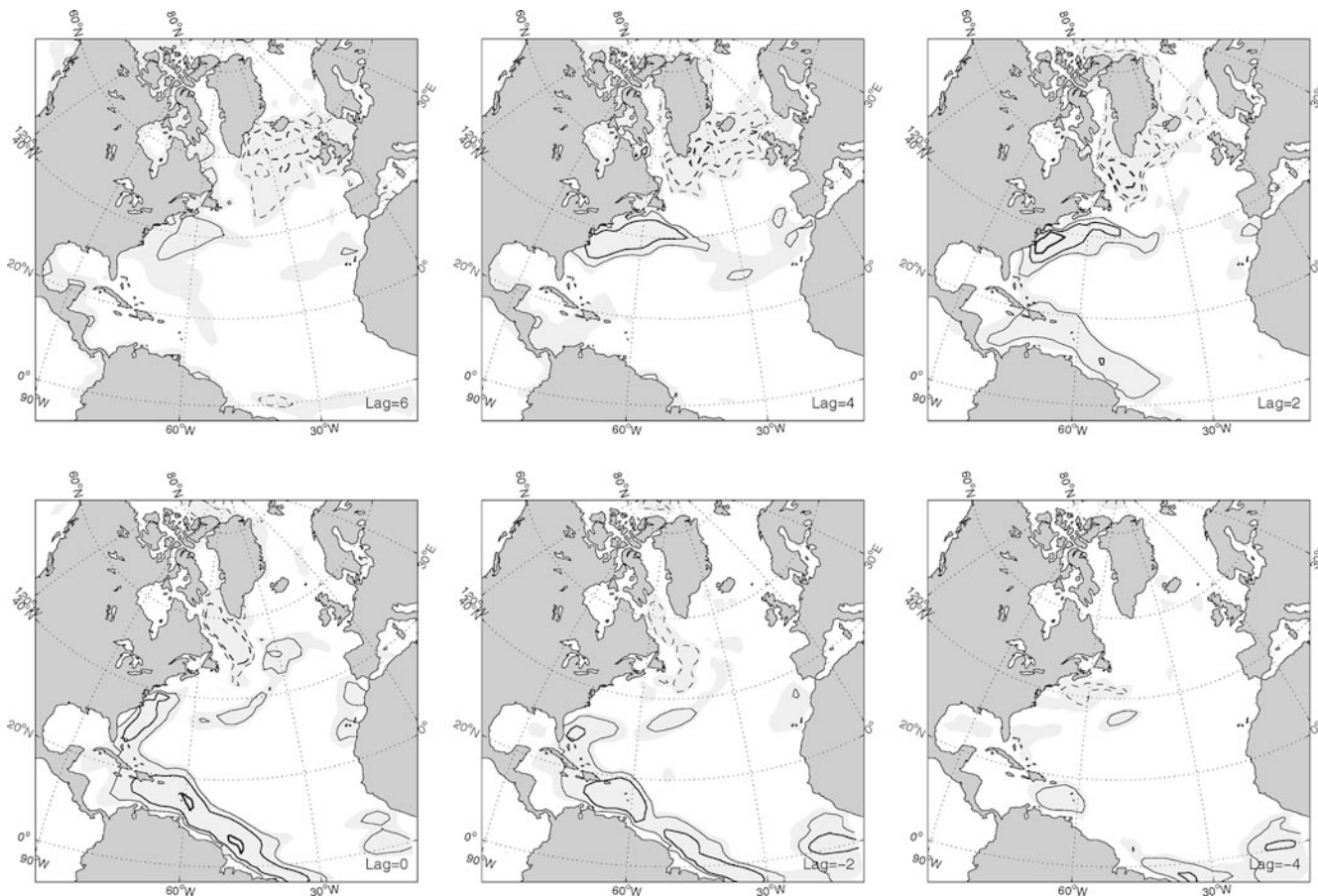
Fig. 15 Lag correlations between the barotropic stream function and PC1 of AMOC in the BCM experiment. Filtering, contouring and significance as for Fig. 9
