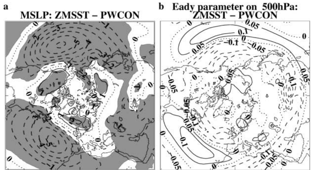
Fig. 8 Differences of ZMSST minus PWCON. ZMSST is a 120 m average of monthly mean data and PWCON is as for Fig. 1. a Mean sea level pressure differences for ZMSST minus PWCON with isobars at 1 hPa intervals. Regions where the changes are 95% significant using a 2-tailed t -test are shaded. b Eady parameter on 500 hPa calculated using data on 600 hPa, 500 hPa and 400 hPa with contours at 0.05 day -1 intervals
