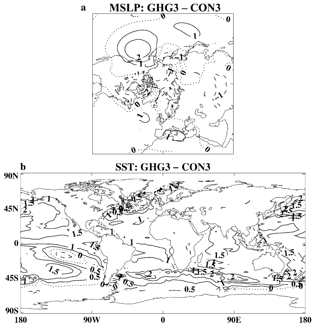
Fig. 9 Difference of GHG3 (30 y (2010-2040) average of monthly mean data for December, January, February) minus CON3 (100 y average of monthly mean data for December, January, February). a Mean sea level pressure with isobars at 1 hPa intervals. b Sea surface temperature with contours at 0.5 K intervals
