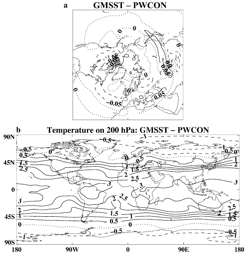
Fig. 6 Differences of GMSST minus PWCON. GMSST is a 120 m average of monthly mean data and PWCON is as for Fig. 1. a Eady parameter on 500 hPa calculated using data on 600 hPa, 500 hPa and 400 hPa with contours at 0.05 day -1 intervals. b Temperature on 200 hPa with contours at 0.5 K intervals
