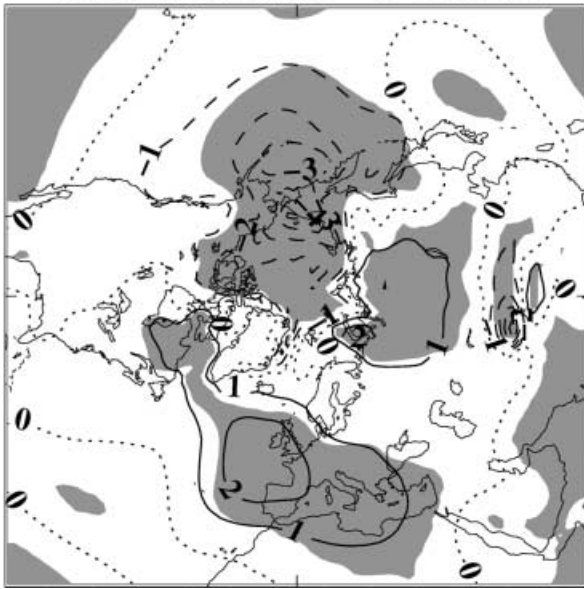
Fig. 5 Mean sea level pressure differences for GMSST minus PWCON with isobars at 1 hPa intervals. Regions where the changes are 95% significant using a 2-tailed t -test are shaded. GMSST is a 120 m average of monthly mean data and PWCON is as for Fig. 1
