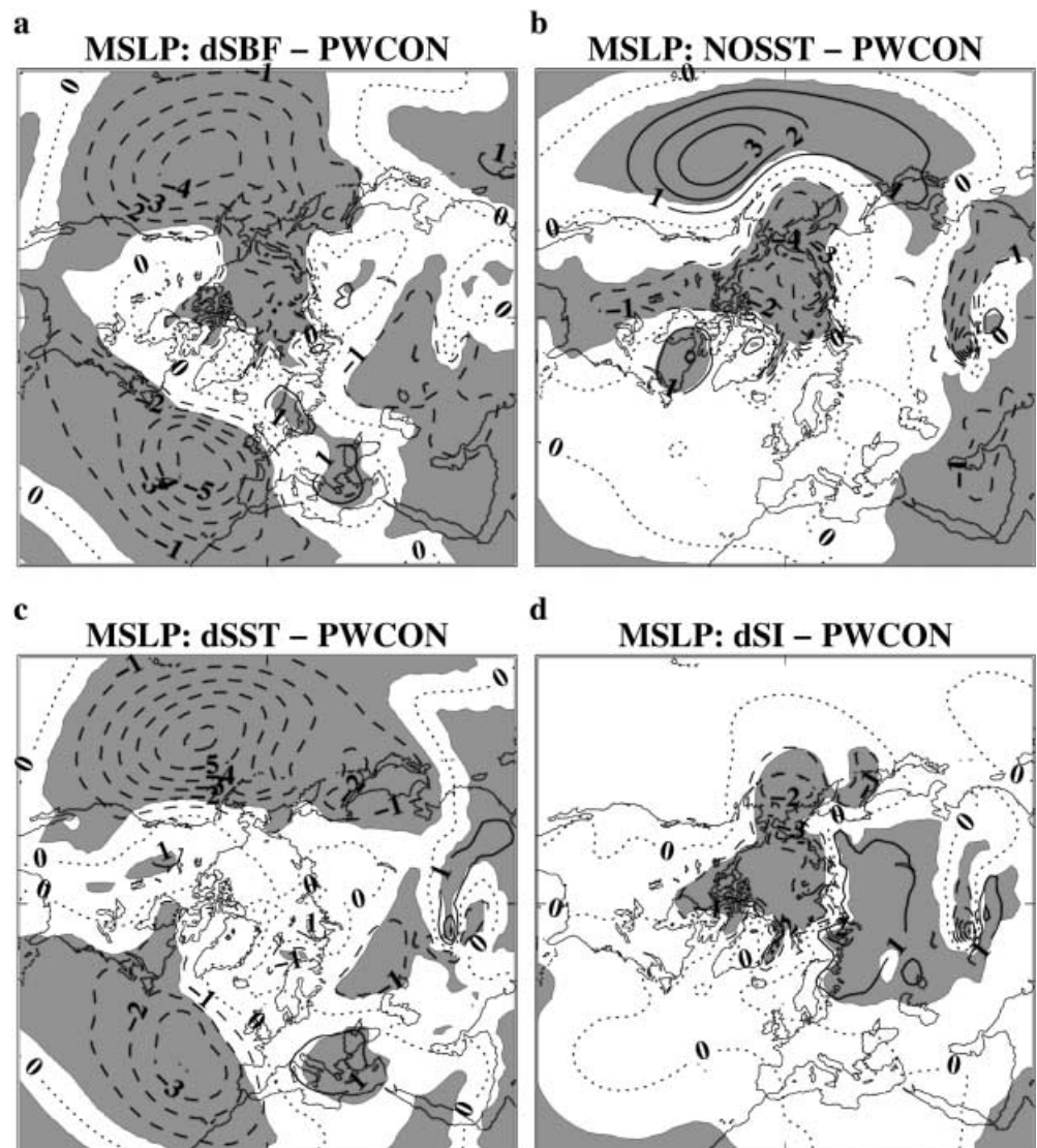
Fig. 4 Mean sea level pressure differences with isobars at 1 hPa intervals. Regions where the changes are 95% significant using a 2-tailed t -test are shaded. Anomaly experiments are 120 m averages of monthly mean data and PWCON is as for Fig. 1. a dSBF minus PWCON; b NOSST minus PWCON; c dSST minus PWCON; and d dSI minus PWCON
