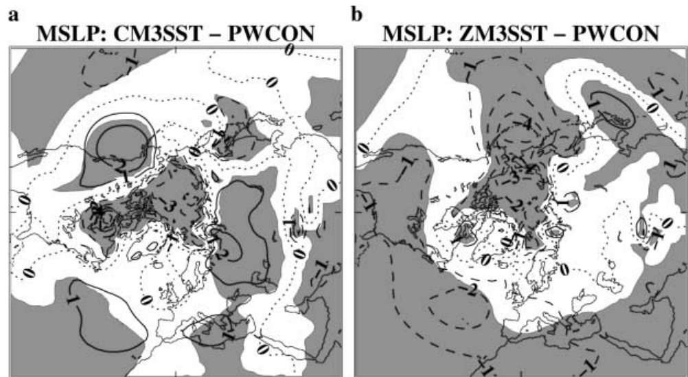
Fig. 10 Mean sea level pressure differences with isobars at 1 hPa intervals. Regions where the changes are 95% significant using a 2-tailed t -test are shaded. Anomaly experiments are 120 m averages of monthly mean data and PWCON is as for Fig. 1. a CM3SST minus PWCON and b ZM3SST minus PWCON
