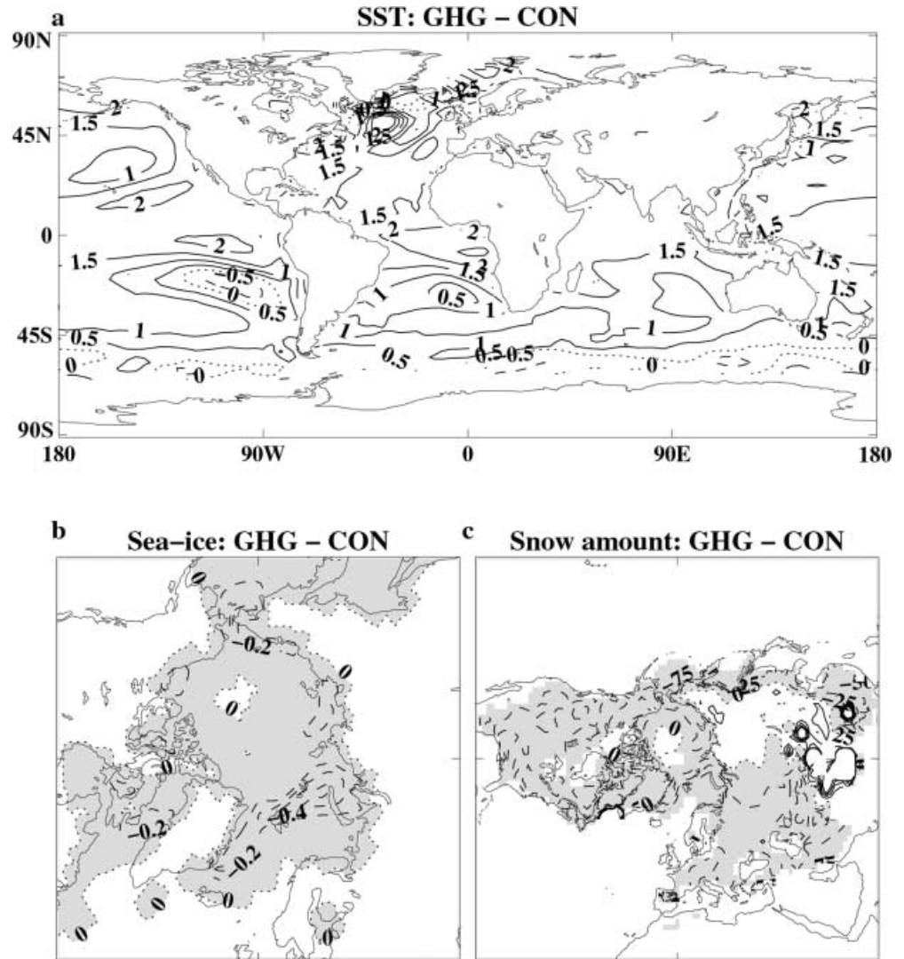
Fig. 2 Difference of the GHG (30 y (2006-2036) average of DJF seasonal mean data) minus CON (120 y average of DJF seasonal mean data). a Sea surface temperature with contours at 0.5 K intervals. b Sea-ice fraction with contours at 0.2 intervals, negative changes are shaded. c Percentage change in snow amount with contours at 25% intervals, negative changes are shaded
