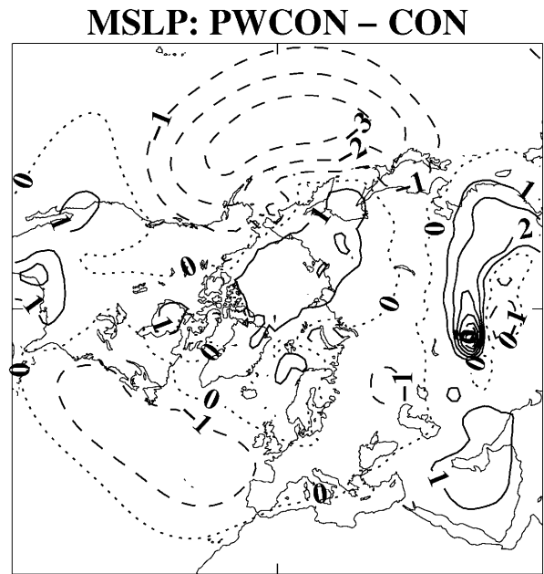
Fig. 1 Mean sea level pressure difference of PWCON (360 m average of monthly mean data) minus CON (120 y average of monthly mean data for December, January, February). Isobars are at 1 hPa intervals. Positive contours are solid, the zero contour is dotted and negative contours are dashed
