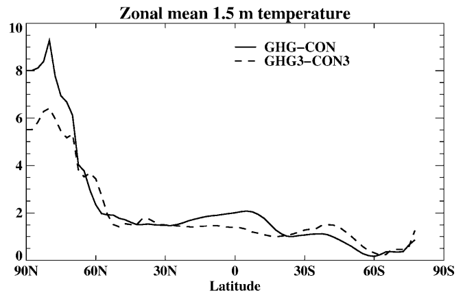
Fig. 7 Zonal mean of 1.5 m temperature changes over open sea and sea-ice points for: GHG (30 y (2006-2036) average) minus CON (120 y average) (solid line); and GHG3 (30 y (2010-2040) average) minus CON3 (100 y average) (dashed line). Calculated using long term means of monthly mean data for December, January, February
