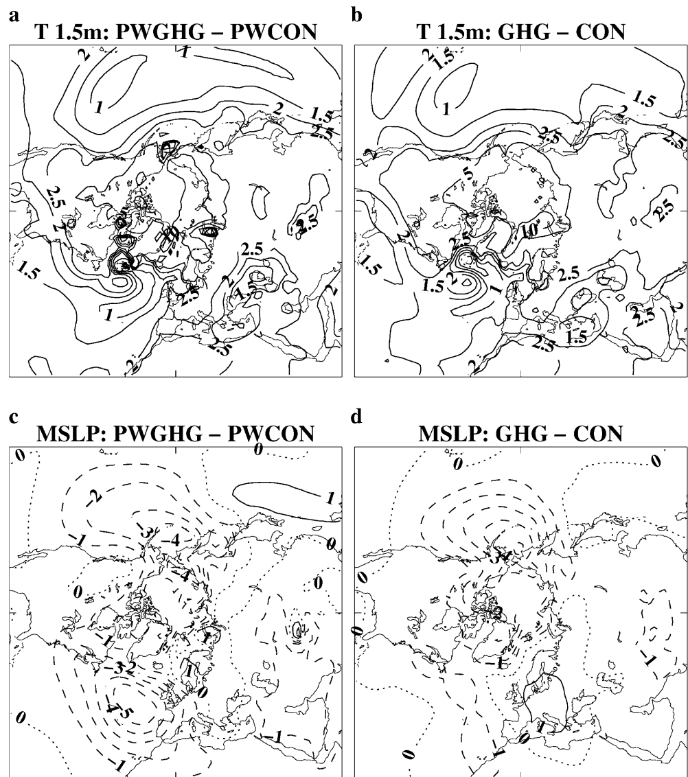
Fig. 3 a and b 1.5 m temperature with contours at 0.5 K intervals to 2.5 K then at 5 K and 10 K. c and d mean sea level pressure differences with isobars at 1 hPa intervals. a and c PWGHG (120 m average of monthly mean data) minus PWCON (as for Fig. 1). b and d GHG (30 y (2006-2036) average of monthly mean data for December, January, February) minus CON (as for Fig. 1)
