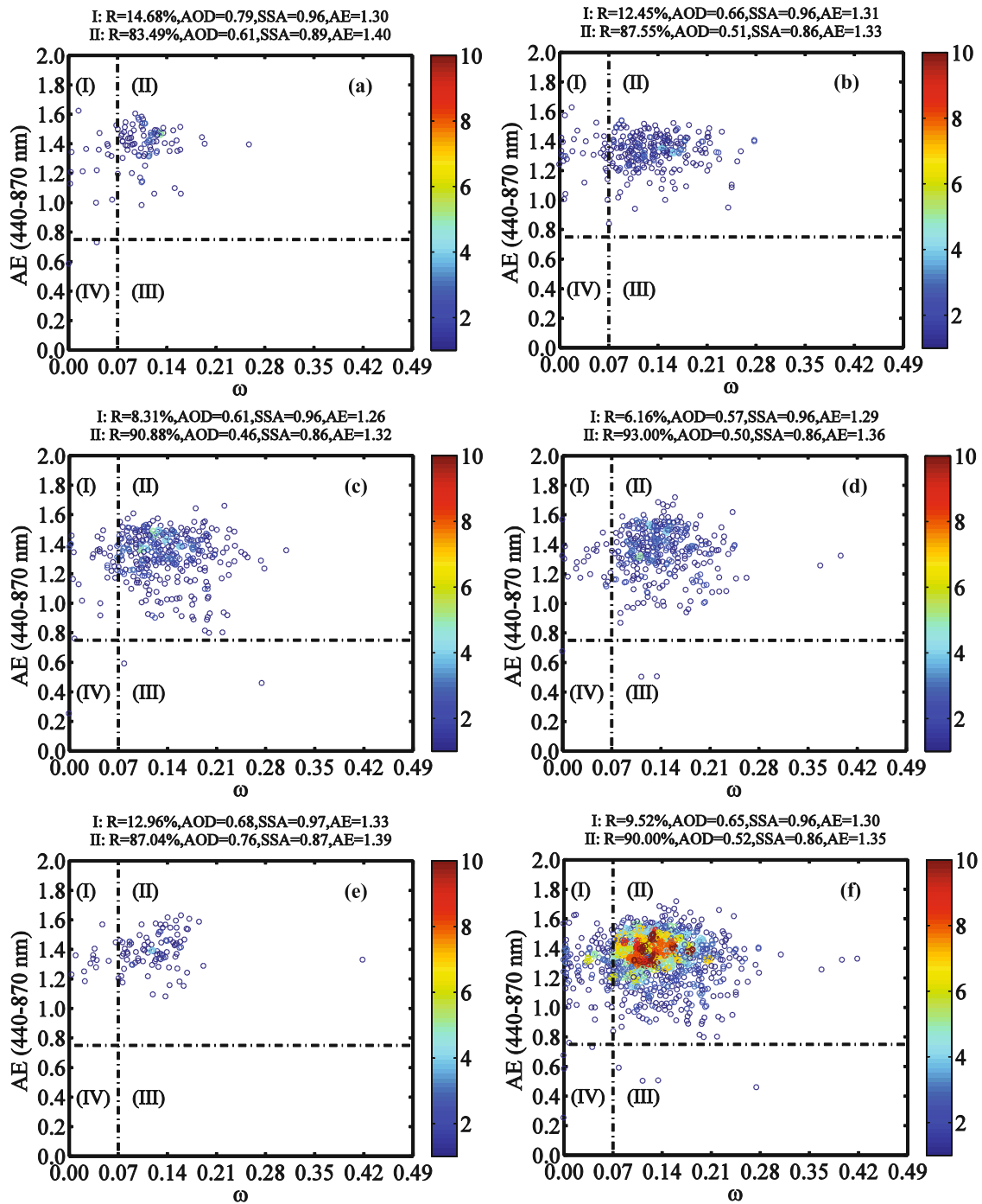
Fig. 6. Classification of the mean physicochemical properties of aerosols into four regions using AE (440–870 nm) and \omega at 440 nm. The color scale represents the relative density of points. Panels (a–f) correspond to October, November, December, January, February, and all data, respectively, in the years 2006–12. R is the proportion of particle amount.
