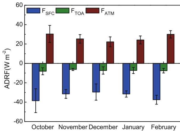
Fig. 8. Monthly mean diurnal ADRF at the surface ( F_{SFC} ), at the top of the atmosphere ( F_{TOA} ), and within the atmosphere ( F_{ATM} ). Error bars represent standard deviations.
