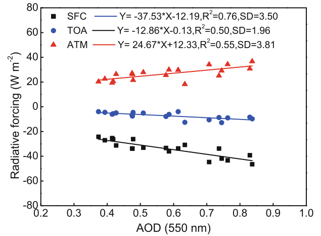
Fig. 9. Diurnal ADRF at the surface (SFC, black), at the top of the atmosphere (TOA, blue), and within the atmosphere (ATM, red) as a function of AOD at 550 nm over the PRD region. Best-fit lines through the points are shown and linear regression functions and statistics (coefficient of determination, R^2 , and standard deviation, SD) are given.
