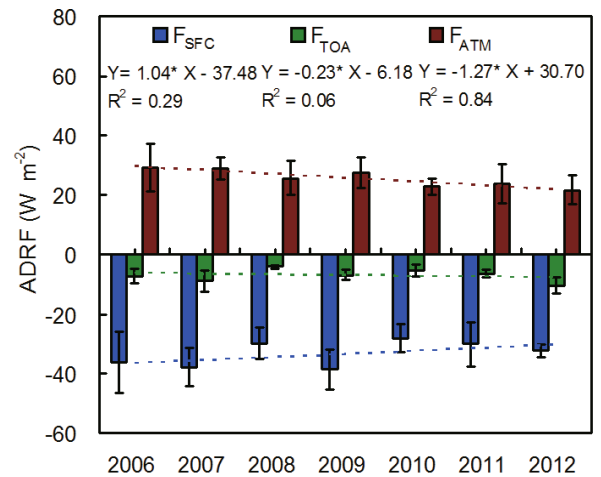
Fig. 10. Interannual trends in diurnal ADRF during the dry season (October to February) in the PRD region. Dashed red, green, and blue lines represent linear-fit lines for ADRF within the atmosphere (ATM), at the top of the atmosphere (TOA), and at the surface (SFC), respectively. Vertical bars represent one standard deviation computed from the monthly mean forcing.
