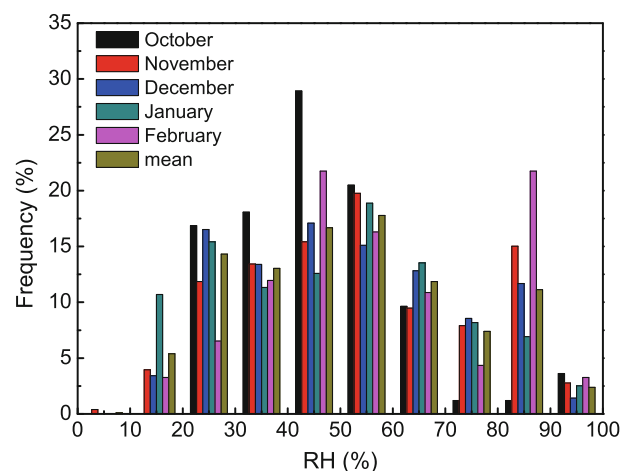
Fig. 4. Frequency distributions of RH. The frequency in each month was calculated using 10 RH bins ranging from 5% to 95%.
