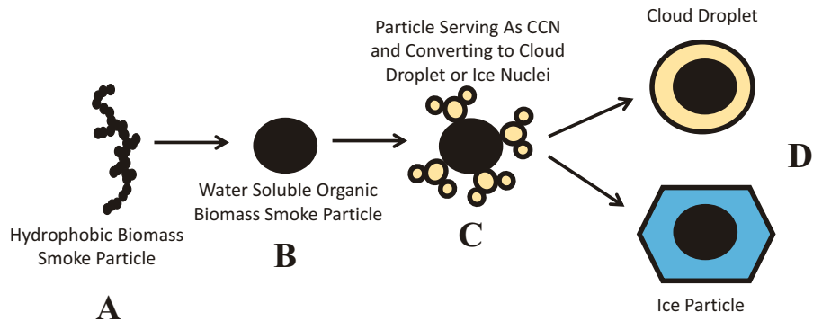
Fig. 5. Conceptual model of a biomass burning smoke particle becoming a cloud droplet (A–C). The hydrophobic smoke particle (A) are aged and oxidized by sunlight and/or gas-phase radicals to a more water-soluble form (B) and becomes a CCN. Net condensation (hygroscopic growth) occurs around the smoke particle (C) to create cloud droplets or ice particles (D) depending on the updraft strength in the cloud (i.e., strong updrafts can lift CCN above the freezing level).
