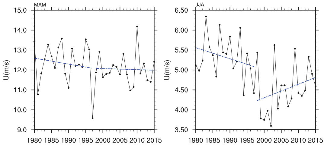
Fig. 5. Temporal evolution (solid curves in black) and LVTs (dashed lines in blue) of the 500-hPa zonal wind in spring and summer averaged over (25°–45°N, 80°–120°E). Units: m s -1 .
