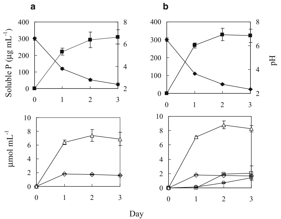
Fig. 1 Relationships between pH, organic acid production and solubilization of calcium phosphate by Aspergillus spp. (a) Aspergillus sp. 1B; (b) Aspergillus sp. 6A., phosphate concentration, (—■—); pH, (—◆—); gluconic acid, (—△—); malic acid, (—◇—); oxalic acid, (—□—); citric acid, (—○—)
