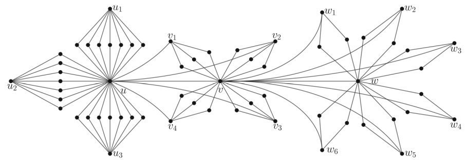
Fig. 2 The graph \mathcal{H}_8
