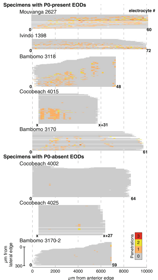
Fig. 7 Heterogeneous and homogeneous electric organ morphology in P. kingsleyae . We show here variation in electric organ morphology from eight individuals, representing three major types of electric organs observed (mostly Pa , mostly NPp and mixed). Number of penetrations in individual section is indicated by color (gray 0, orange 1, yellow 2, red 3, white section missing/no data). For all plots, horizontal axis represents distance from the anterior edge of the electric organ, and the vertical axis represents distance from the lateral edge of the electric organ (top lateral). Mouvanga 2627 and Ivindo 1398 represent “typical” patterns of penetration in P0-present type Mormyrids. Pa type morphology is present in each electrocyte, characterized by a colored box in each column from anterior to posterior. In Bambomo (3170; 3118) and Cocobeach (4015) P0-present specimens the electric organ is heterogeneous (both Pa and NPp electrocyte morphology). P0-absent specimens (Bambomo 3170-2; Cocobeach 4002, 4025) exhibit comparatively homogeneous NPp morphology in the electric organ. Numbers of electrocytes are noted in bold on the ends of each plot; note the variability in the number of electrocytes between individuals. For Cocobeach 4025 and 4015 only a posterior portion each electric organ was available for analysis
