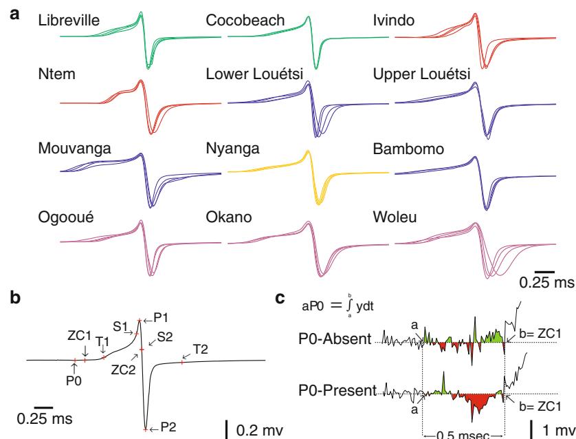
Fig. 2 EOD waveform analysis of P. kingsleyae . a Representative variation in EOD waveforms of P. kingsleyae from 12 localities ( n = 4 EODs for each locality). Waveforms vary principally in the duration and shape of initial P1 phase. b Nine landmarks were determined for each of 553 EOD recordings (indicated by red crosses). For each landmark, time and voltage relative to P1 were determined. See Table 2 for definitions of all landmarks used in this
