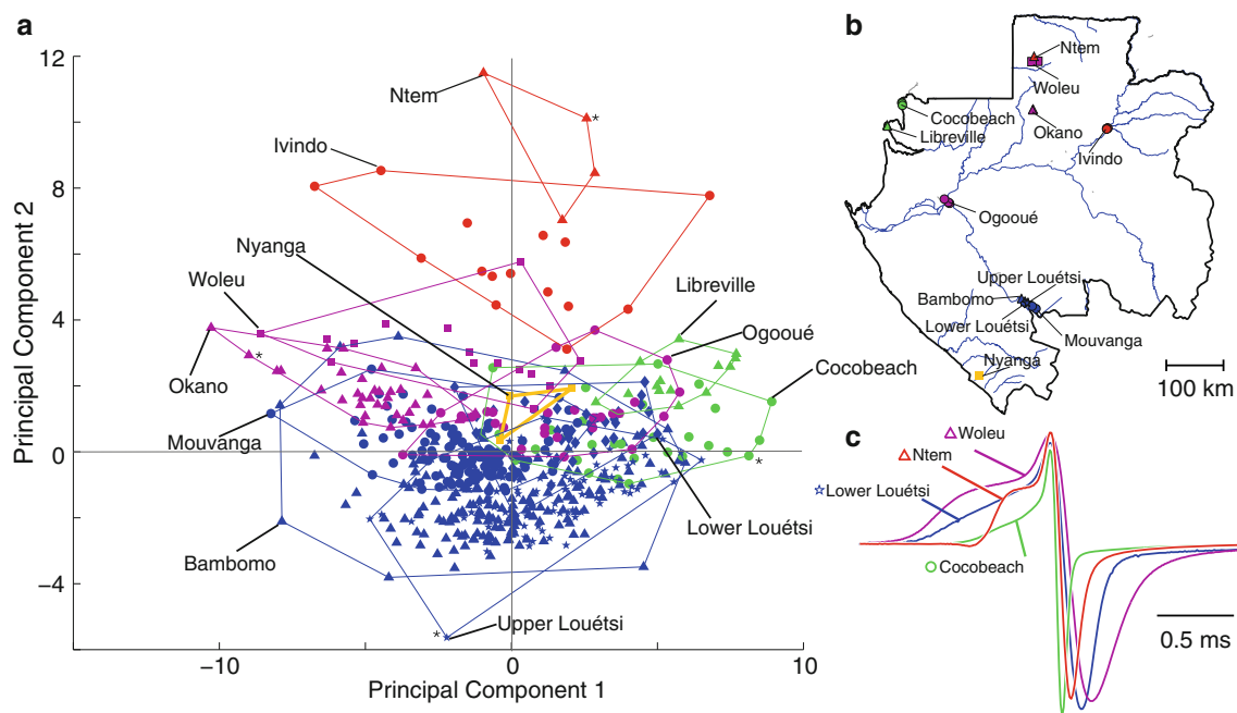
Fig. 3 Principal components analysis of EOD waveform variation for the P. kingsleyae dataset. a The first two principal components ( n = 553 ) describe variation across 21 variables. Each data point represented in principal component space has a representative shape and color corresponding to locality ( b ). Each locality is bounded by a minimum polygon (colored line, labeled with locality). Asterisk
