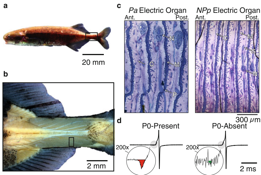
Fig. 1 Paramormyrops kingsleyae and its divergent signaling types. a P. kingsleyae from Biroundou Creek (see Table 1). b The electric organ of P. kingsleyae is located in the caudal peduncle. When skin and scales are removed, the electric organ is clearly visible as a striated structure flanked by two groups of muscles. c Two specimens are represented by sections of electric organs; P. kingsleyae that have either penetrating with anterior innervation ( Pa ) type electric organs or non-penetrating with posterior innervation ( Npp ) type electric organs. Anatomical features
