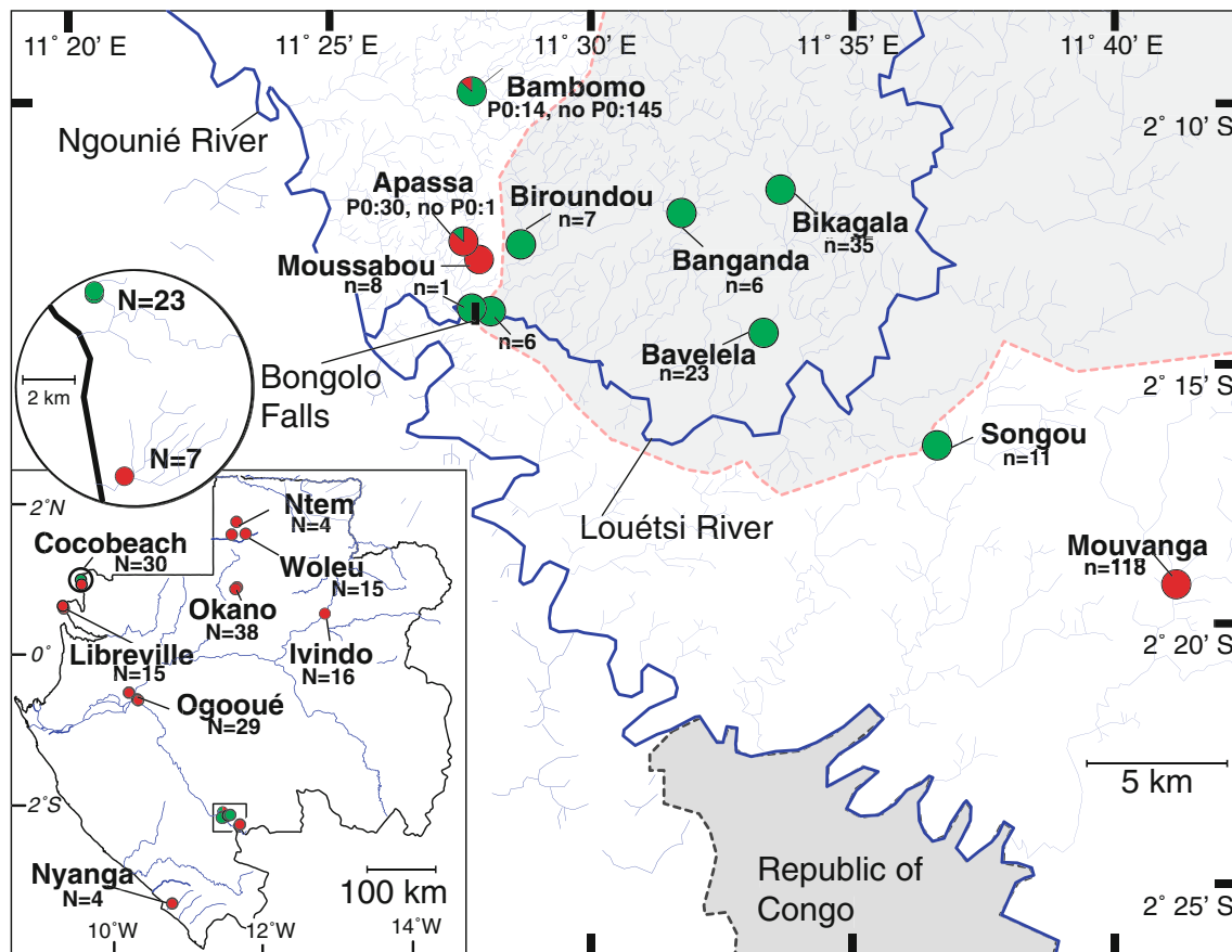
Fig. 6 Geographic distribution of P0 absent and P0 present P. kingsleyae collected 1998–2009. We indicate the distribution of P0 absent and P0 present individuals in Gabon at a variety of geographic scales. Each sampled locality is displayed as a pie chart proportional to signaling types collected. Pie charts are shaded based on signal type; red indicates proportion of P. kingsleyae that are P0-present; green indicate proportions of P. kingsleyae that are P0-absent. Sample sizes for each population are indicated. The map of Gabon (lower left) represents our sampling efforts across Gabon; the circular inset is a
