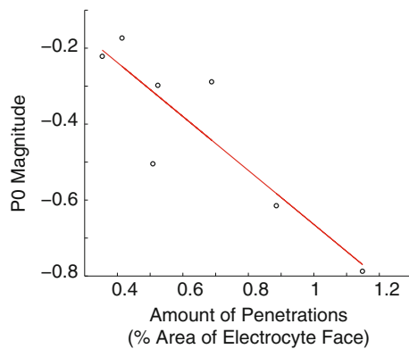
Fig. 9 Morphological correlates of signal variation in P. kingsleyae electrocytes. There is a linear relationship between the percent area of electrocyte face devoted to penetrations and magnitude of P0 for seven individually dissected electrocytes ( P = 0.008 ; R^2 = 0.78 )
