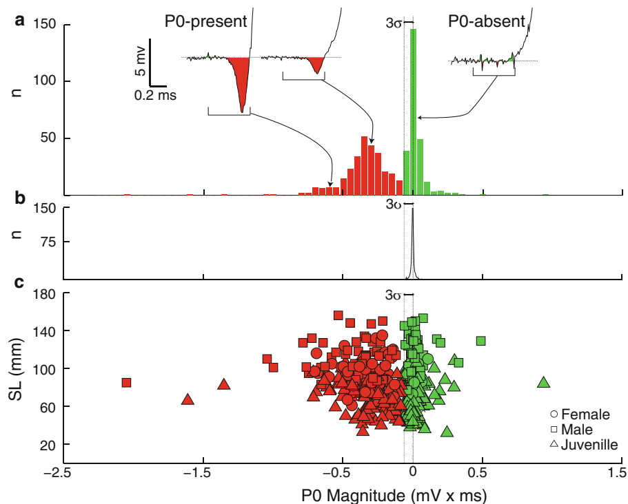
Fig. 5 Distribution of P0 magnitude among collected P. kingsleyae specimens. a Histogram of P0 areas ( n = 553 ) indicates a bimodal distribution of P0 areas corresponding to P0-present waveforms and P0-absent waveforms. Modal P0 magnitude of P0-present waveforms is -0.35 \text{ mV} \times \text{ms} , modal value for P0-absent waveforms is 0.00 \text{ mV} \times \text{ms} . Insets show representative EOD waveforms; far left inset is P0-present ( P0 = -0.79 \text{ mV} \times \text{ms} ), middle left is P0-present ( P0 = -0.17 \text{ mV} \times \text{ms} ), right inset is P0-absent ( P0 = 0.03 \text{ mV} \times \text{ms} ) b . Shown is a histogram of area measurements in the first 0.5 ms of each
