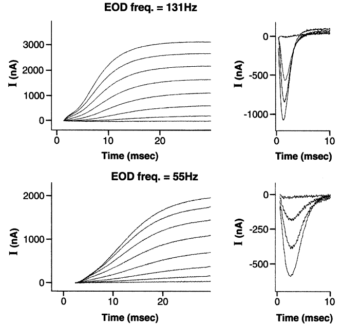
Fig. 8 Kinetics of Na^+ current inactivation and K^+ current activation vary with EOD frequency and sex in Sternopygus . Top traces are Na^+ and K^+ currents recorded under voltage clamp from the electrocytes of a fish with a high EOD frequency (female). Bottom traces are these currents recorded from a fish with a low EOD frequency (male). Note that the rates at which the Na^+ current inactivates and the K^+ current activates are faster in females than in males (McAnelly and Zakon 2000)
