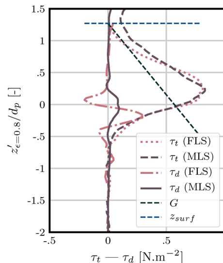
Fig. 16 Comparison of the dispersive and turbulent stresses obtained using either a fixed laser sheet (FLS) or the PIV–RIMS methodology. In contrast to using the FLS procedure, PIV–RIMS captures the variability of interactions in the transverse direction y . The resulting averaged profiles provide a better representation of the profiles at the mesoscopic scale
