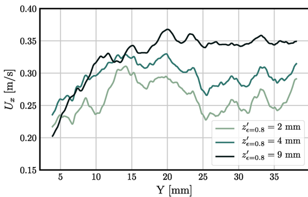
Fig. 11 Sidewall influence. The horizontal velocity profile has been averaged along the streamwise x -direction and plotted for different elevations z'_{\epsilon=0.8} = z - z_{\epsilon=0.8} as a function of their distance from the sidewall Y
