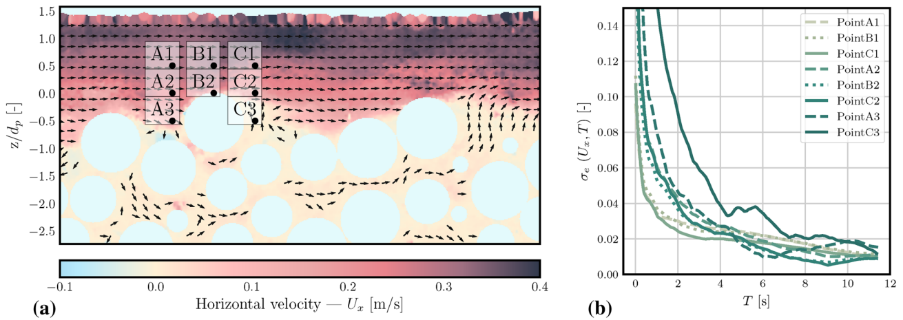
Fig. 8 a Turbulence in the fluid flows at eight points of interest surrounding a bead on top of the permeable bed were analysed statistically. (b) Evolution of the standard deviation of the empirical error
