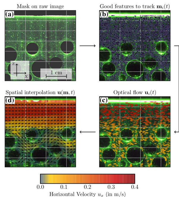
Fig. 17 Graphical overview of the workflow: from the raw image to the velocity field
