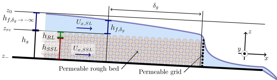
Fig. 14 Permeable outlet condition to ensure a subsurface flow. Measurements must be taken along a sufficiently long distance \delta_g to ensure that this condition’s boundary effect is negligible
