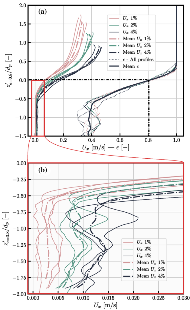
Fig. 13 Evaluation of reproducibility with different bed structures. a Velocity profiles (continuous and dash-dotted lines) and porosity profiles (dotted lines) for different slopes but using a constant flow discharge q_f = 0.30 \pm 0.015 \text{ m}^2/\text{s} . The modified coordinate is given by z'_{\epsilon=0.8} = z - z_{\epsilon=0.8} . b A zoom in on the roughness and subsurface velocities
