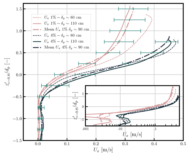
Fig. 15 Velocity profiles for various \delta_g values with which to evaluate the flow uniformity condition along the flume. The dashed-dotted lines represent the averaged velocity profiles at \delta_g = 90 \text{ cm} . The error bars show the deviations from the averaged profiles due to the modification of the bed structure. They represent the 95% confidence interval. \sigma_{U_x}(z) is the standard deviation at z calculated from the profiles shown in Fig. 13. The continuous lines are the profiles measured at \delta_g = 60 \text{ cm} , and the dashed lines were measured at \delta_g = 90 \text{ cm} . The bottom-right inset plots the same profiles using a logarithmic scale to emphasise the marked differences at low velocities
