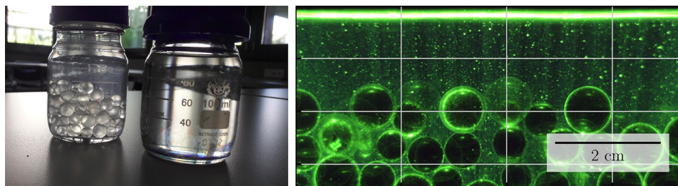
Fig. 2 Left: Two beakers containing equal quantities of borosilicate beads representing the porous bed. The left-hand beaker contains water and the refractive index mismatch means that the beads are visible; the right-hand beaker contains a fluid whose refractive index matches that of the beads, rendering them invisible, but the interstitial fluid can be probed using flow visualisation techniques. Right: Pho-
