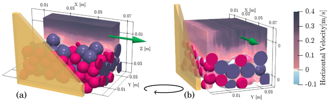
Fig. 10 Three-dimensional visualisation of the horizontal velocity. a Side view of a slab of the velocity field at FLS position Y_m = 25 mm (the same position as the FLS results above—see Fig. 7). b Frontal view of the flow, sliced along y . This view enables us to appreciate
