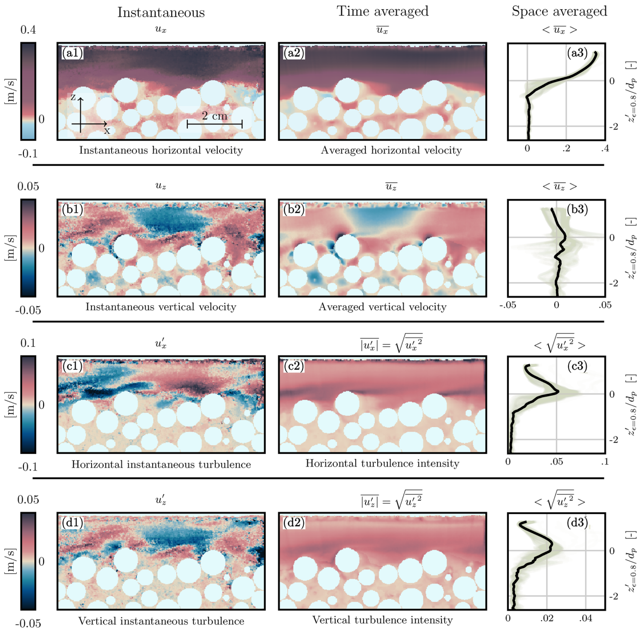
Fig. 6 From instantaneous to double-averaged quantities. In this configuration, the laser sheet was fixed at a position Y_m = 25 mm from the sidewall and it recorded the flow for 20 s. Instantaneous measurements were selected randomly, but each measurement is shown for
