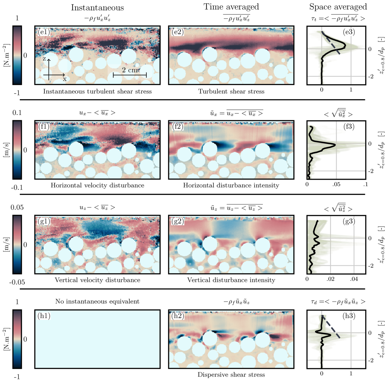
Fig. 7 From instantaneous to double-averaged quantities with conditions similar to Fig. 6. From the top to the bottom, the images show turbulent stresses, the horizontal and vertical disturbances and the
