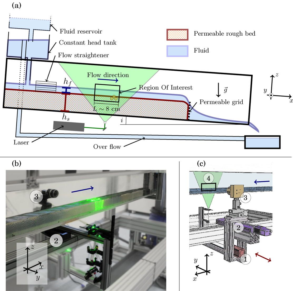
Fig. 3 a Sketch of the experimental set-up. b Photograph of the flume. c Three-dimensional visualisation sketch. ① laser; ② linear unit for displacement along the y-axis; ③ high-speed camera; ④ laser sheet
