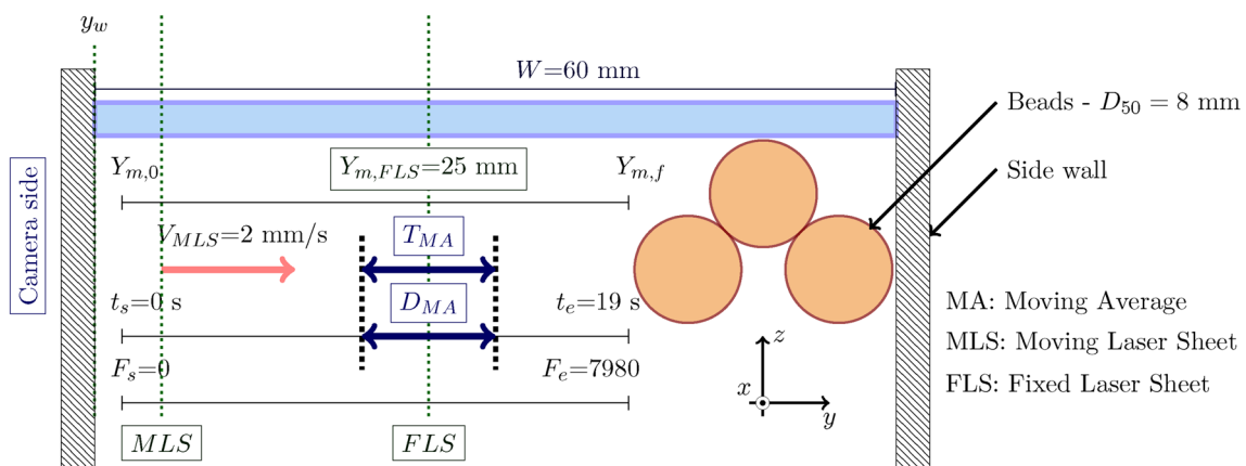
Fig. 5 Schema of the transverse scanning set-up and comparison with a fixed laser sheet (FLS) measurement. F_s and F_e are the start and end frame indexes, respectively
