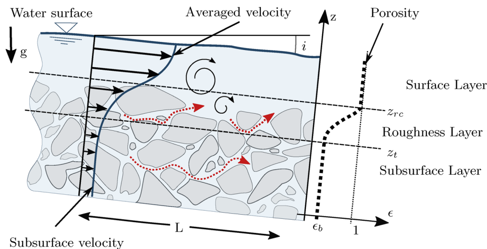
Fig. 1 Grain-scale processes of a turbulent flow over a rough permeable bed and double-averaged quantities. The porosity \epsilon and velocity profiles result from the double averaging procedure over a thin layer parallel to the mean bed surface over the length L . The flow is subdivided into three specific regions: the surface layer , the roughness layer and the subsurface layer . The roughness layer is bounded
