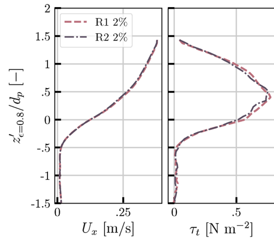
Fig. 12 Comparison between two consecutive runs using the PIV–RIMS procedure, with each run using identical bed structure and flow characteristics [left] Velocity profiles [right] turbulent stress profiles. Velocity profiles look very similar while a slight difference is observable in turbulent stress profiles
