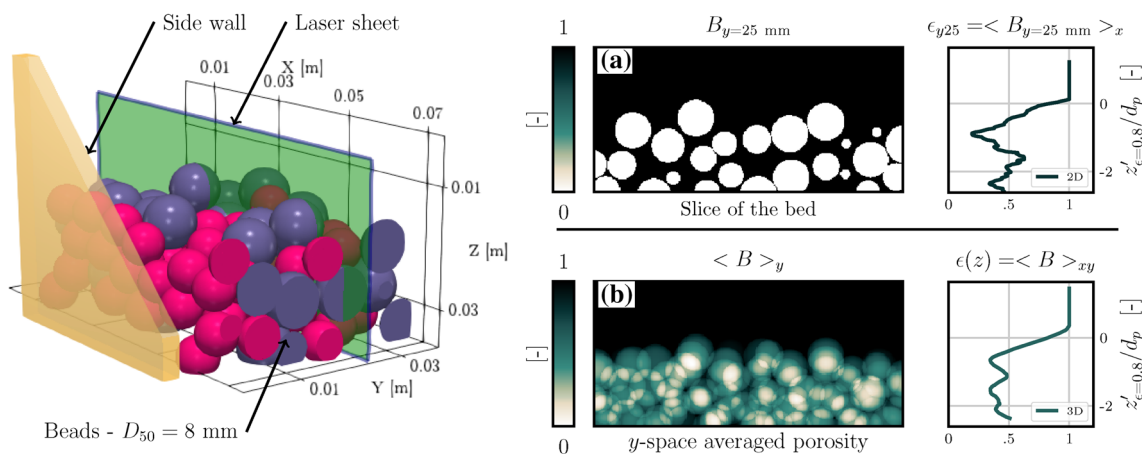
Fig. 4 Porosity measurement using RIMS: once the beads have been located, we define the porosity array B(x, y, z) . a The B field averaged in the x -direction in a slice located at Y_m = y - y_w = 25 mm from the wall position y_w . b Averaging B over x and y gives us a
