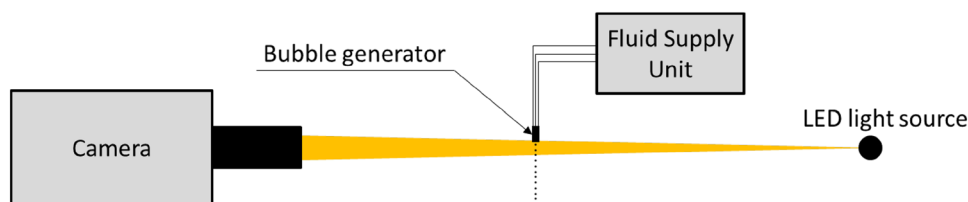
Fig. 2 Schematic illustration of the experimental setup for bubbles shadow visualization
