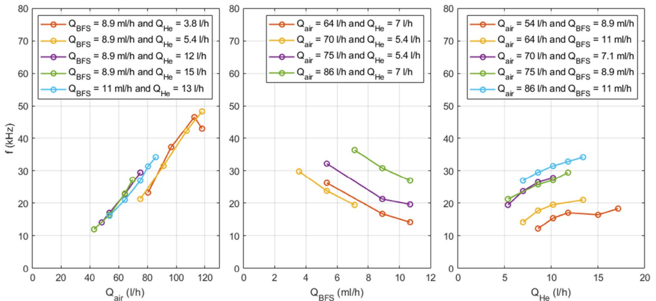
Fig. 13 Influence of air, helium and soap flow rates on the HFSB production rate
