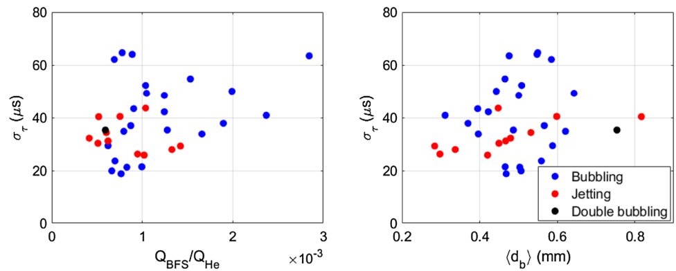
Fig. 11 Standard deviation of HFSB time response
