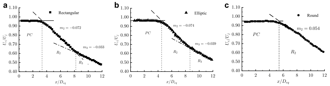
Fig. 6 Velocity distribution showing decay of mean streamwise velocity in the jet centerline for a rectangular b elliptic c round jets. The potential core region is denoted by PC. R_2 and R_3 denote two regions of centerline velocity decay
