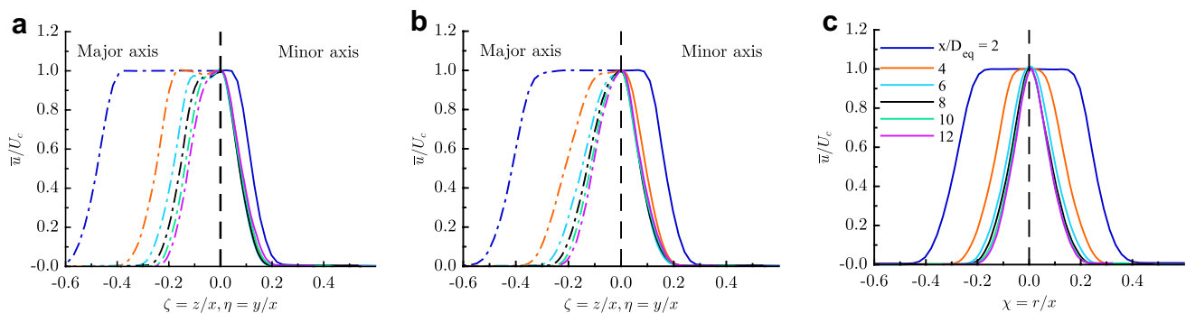
Fig. 5 Normalized mean streamwise velocity profiles at various axial locations for a rectangular b elliptic c round jets. For asymmetric jets, profiles in the major and minor axis planes are included in the same plot
