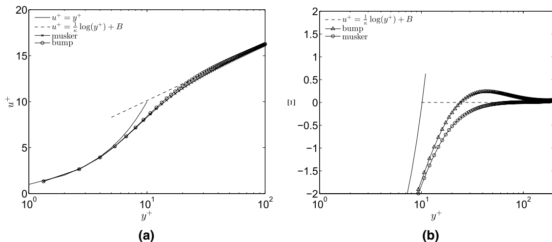
Fig. 1 Detail of mean velocity profile. a Detail on the buffer region for Musker (x) velocity profile, b \Xi = u^+ - \left[ \frac{1}{\kappa} \ln(y^+) + B \right] for bump ( \Delta ) and Musker (o) velocity profiles
