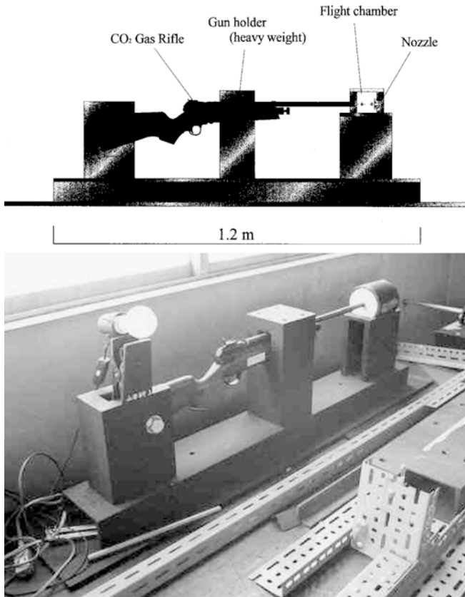
Fig. 1. a Schematic of the small high-speed liquid jet apparatus. b Photograph of the small high-speed liquid jet apparatus
