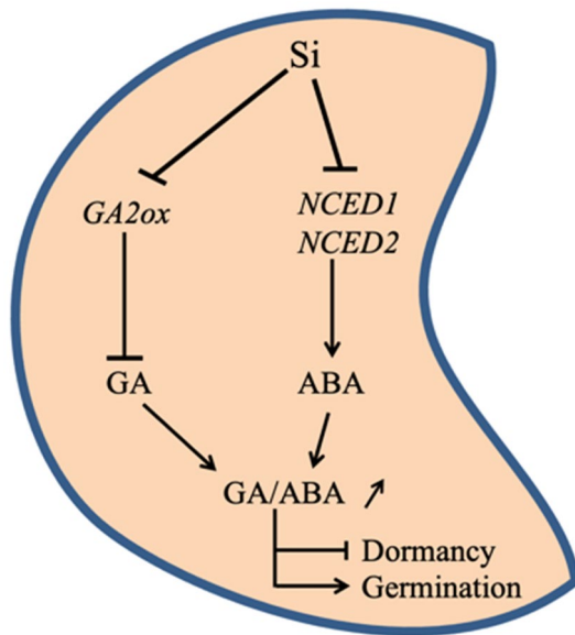
Fig. 3 Proposed effects of exogenous Si application on phytohormone balance during seed germination under abiotic stresses. NCED nine-cis-Epoxy-carotenoid dioxygenases, GA2ox Gibberellin 2-oxidases, GA gibberellic acid, ABA abscisic acid
