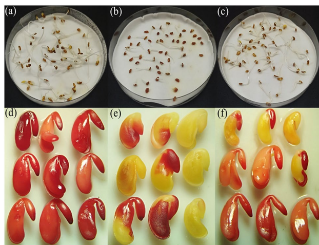
Fig.1 Germination (a–c) and embryo viability (d–f) of seeds of the Moroccan Medicago sativa L. Demnate 201 variety treated with water (a, d), with 200 mM NaCl (b, e), or with 200 mM NaCl and 3 mM silicon in the form of \text{CaSiO}_3 (c, f). The germination rates were a 100%, b 51%, and c 85% after seven days of treatment. Embryo viability was evaluated after 12 h of treatment using the 2, 3, 5 triphenyltetrazolium chloride (TTC) method in which viable embryos are stained red due to the reduction of TTC by respiratory activity of the cells. Images were taken under a binocular magnifying glass with \times 10 magnification
