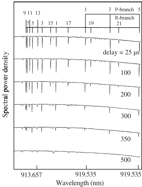
Fig. 24. Absorption spectra of \text{He}_2 molecules in an electric discharge plasma of He at 13 mbar, at various times after the termination of the discharge [189]
