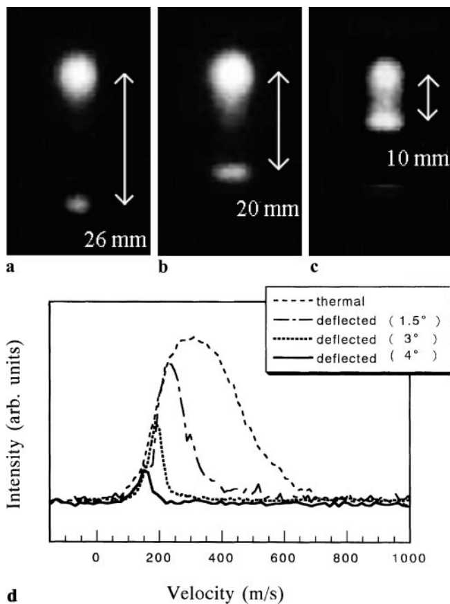
Fig. 1a–d. Typical CCD pictures in the probe region of the atomic beam after deflection with a deflection angle of a 4°, b 3°, and c 1.5°, respectively. d shows the velocity distributions of the deflected atoms in these cases
