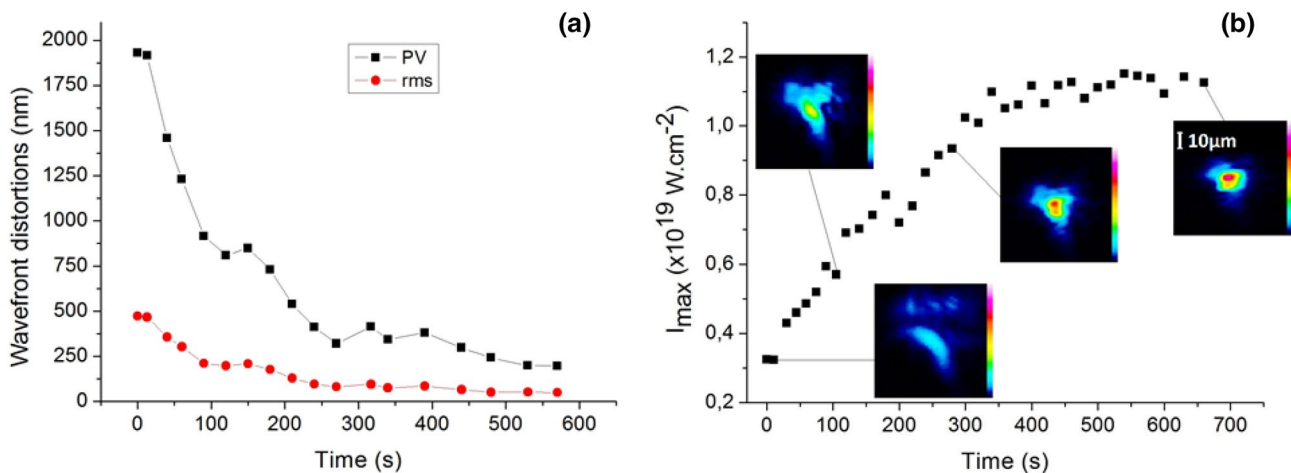
Fig. 7 a Evolution of the differential beam wavefront measured at high energy (320 mJ per pulse) as compared with the wavefront measured at low energy ( < 30 mJ per pulse) after pre-compensation of the thermally induced wavefront distortions. b Evolution of the peak intensity delivered on target as a function of time. Snapshots of the beam profile in the focal plane are displayed to show the cor-
