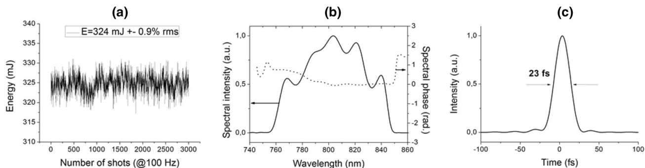
Fig. 2 a Evolution of the pulse energy before compression. The average energy is ~324 mJ per pulse with an energy stability of 0.9% rms. b Spectral intensity (solid lines) and phase (dot line) of the amplified
