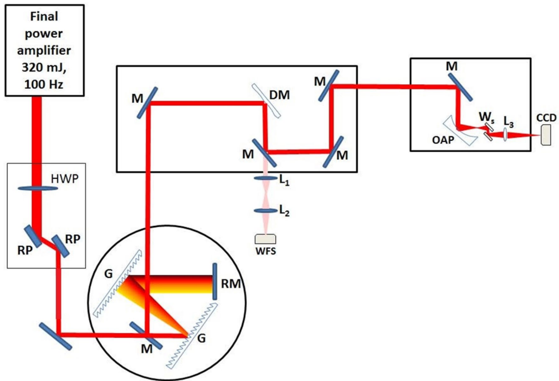
Fig. 4 Experimental set-up for high-intensity experiments. It is made of an energy attenuator, the compressor chamber, the adaptive optics chamber and the interaction chamber. The propagation of the laser beam is represented by the red line. HWP half-waveplate, RP Brewster cut reflective polarizer, G diffraction grating, RM roof mirror, M dielectric coating mirror R_{\max} in 750–850 nm spectral range, DM
