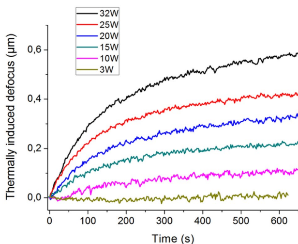
Fig. 6 Time-dependent thermally induced defocus for different average powers before the compressor. Note that the configuration studied includes the deformable mirror (whole laser chain)
