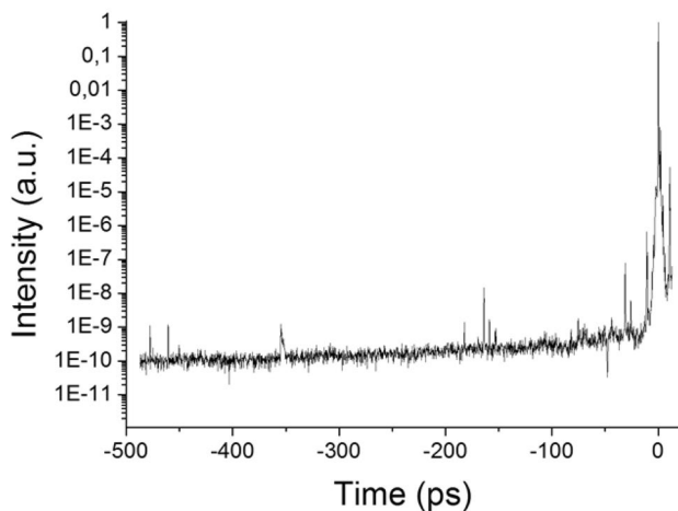
Fig. 3 Third order autocorrelation trace of the amplified pulse for delay up to 480 ps before the main pulse. The dip near -50 ps shows the actual noise level of this measurement
