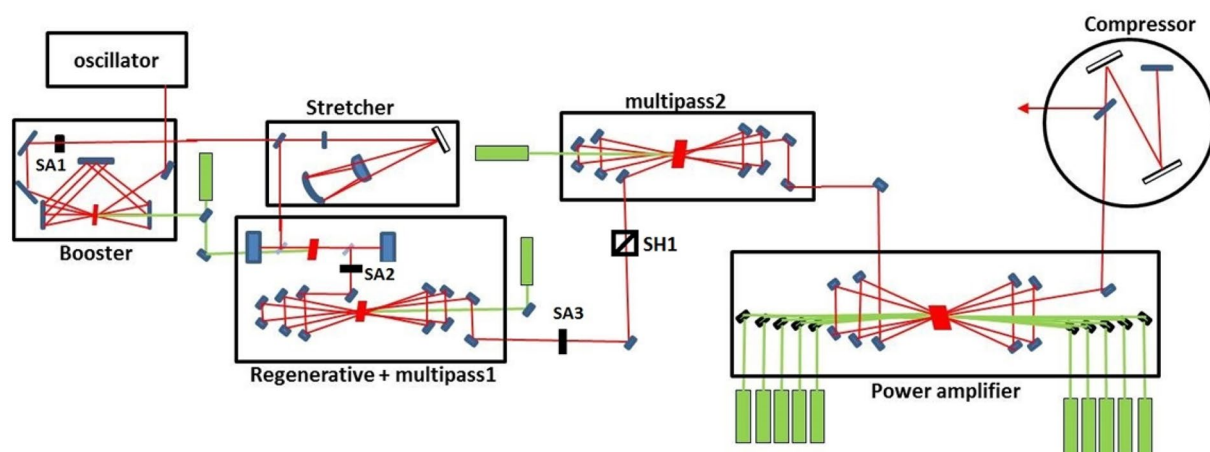
Fig. 1 The 100 Hz multi-TW laser set-up. SA1, SA2 and SA3 are saturable absorbers (RG-850 long pass filters, 2 mm thick for SA1, 1 mm thick for SA2 and SA3), SH1 is an electronic fast shutter (Newport, model 76992) whose aperture diameter is 6 mm, with an opening time < 1 ms. The pulse energy is measured at 10 \mu J after the
