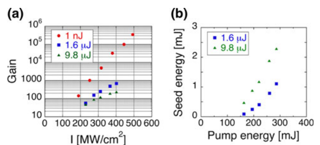
Fig. 4 a OPCPA energy gain as a function of pump intensity in two-stage BBO crystal layout. Solid-circles, rectangles, and triangles represent seed energies of 1 nJ in first stage, 1.6 \mu J in second stage, and 9.8 \mu J in second stage, respectively. b Output energy from the second-stage OPCPA as a function of input pump energy
