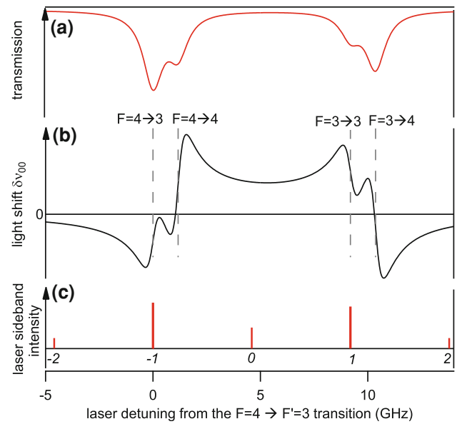
Fig. 2 Schematic view of light-shift in the case of CPT on the Cs D1 line. a Example of an optical transmission spectrum for a thermal Cs vapour, showing line broadening by a buffer-gas. b Frequency-dependence of the light-shift \delta v_{00} of the clock transition, for a monochromatic constant-intensity laser. The dashed vertical lines indicate the positions of the optical transitions. c Typical example of a multi-frequency laser spectrum, for CPT excitation by the positive and negative first-order sidebands. Italic numbers give the order j of each sideband. The resulting clock transition light-shift under polychromatic excitation is the product of spectra b with c , summed over all laser sidebands
