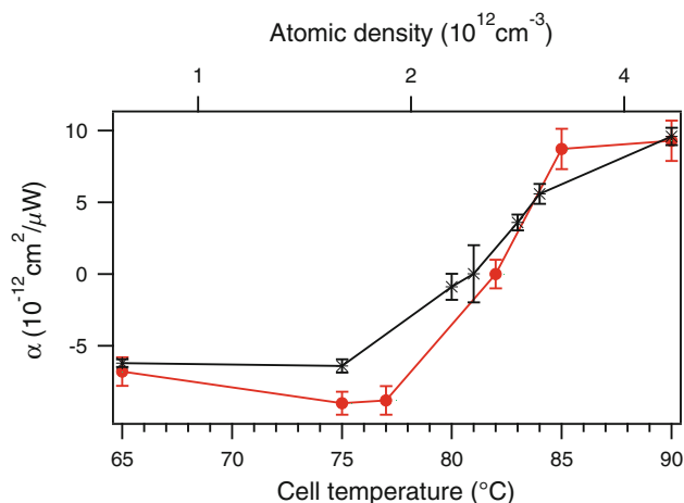
Fig. 7 Intensity light-shift coefficient \alpha as a function of the cell temperature (red circles). The measurement was repeated after 14 months (black stars). \alpha crosses the zero value level for a cell temperature of 81^\circ\text{C} . Coupling is via the F' = 3 excited state (laser locking point 1 in Fig. 4a)
