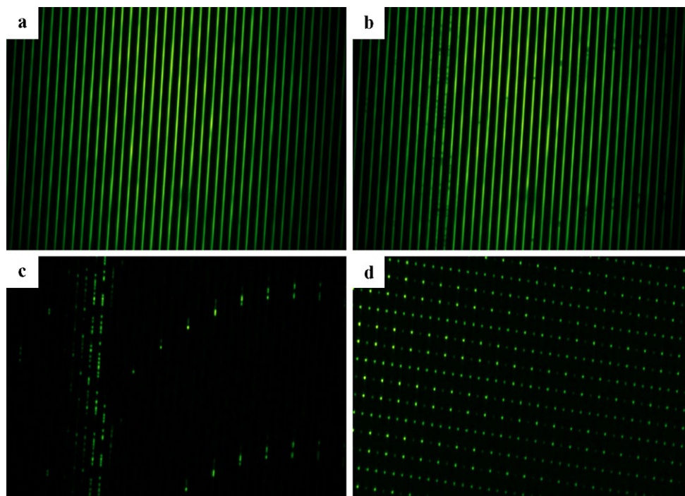
Fig. 3 Two-dimensional VIPA spectrometer images captured by CCD. (a) Dispersed source spectrum with no gas sample in the cell. (b) Methane absorption features imprinted on source spectrum. (c) Subtracted image (a) – (b) , to highlight the absorption spectrum pattern on the VIPA image. The VIPA's free spectral range is apparent in the vertical repetition of the absorption feature pattern at the top and bottom of image. (d) 10 GHz Ti:Sapph comb calibration grid, optical filter etalon causes variations in comb mode intensity
