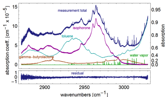
Fig. 7 Measured total absorption of the solvent mixture ( top ). The other spectra show the contributions of the constituents found by fitting the total spectrum with adjustable partial pressures. Absorption coefficient fit residuals are shown below the main graph and have a standard deviation of about 9 \times 10^{-7} \text{ cm}^{-1} , within a factor of four of the shot noise limited minimum absorption coefficient for a single frequency step
