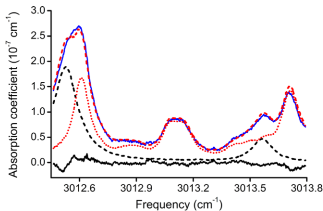
Fig. 10 Measurement of CO with purity 4.7 (solid blue line) and the corresponding fit (dashed red line) which is the sum of the absorption of 1.6 \mu\text{mol/mol} \text{H}_2\text{O} (dashed black line) and 12 nmol/mol \text{CH}_4 (dotted red line). The solid black line represents the residual of the measurement and the fit. Individual \text{H}_2\text{O} and \text{CH}_4 spectra were recorded in nitrogen. A small background absorption of 3 \times 10^{-8} \text{ cm}^{-1} was subtracted from the measurement data (due to the presence of a large absorbing molecule or far wing absorptions by CO)
