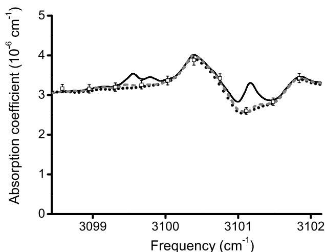
Fig. 7 Measurement of 1 \mu\text{mol/mol} benzene (black line) and after subtraction of water vapor interference (dashed grey line). Spectra from PNNL (black dots) and NIST (black squares including expanded uncertainty) database are also shown
