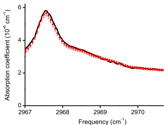
Fig. 9 Measurement of 200 nmol/mol propane (solid line) and the comparison with PNNL database (red dots including expanded uncertainty)
