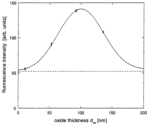
Fig. 8. Fluorescence intensity of a ghost stained with the dye DiIC 12 versus the thickness d_{\text{ox}} of silicon dioxide. The mean and \pm\sigma -values of the Gaussians are shown as obtained from the histograms of Fig. 7. The optical theory is fitted with a distance d_{\text{cleft}} = 12.1 nm (stochastic error \pm 0.4 nm) between membrane and oxide. The dotted line marks the background
