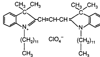
Fig. 2. Amphiphilic trimethin-indocarbocyanine dye DiIC 12 used to stain the erythrocyte membrane
