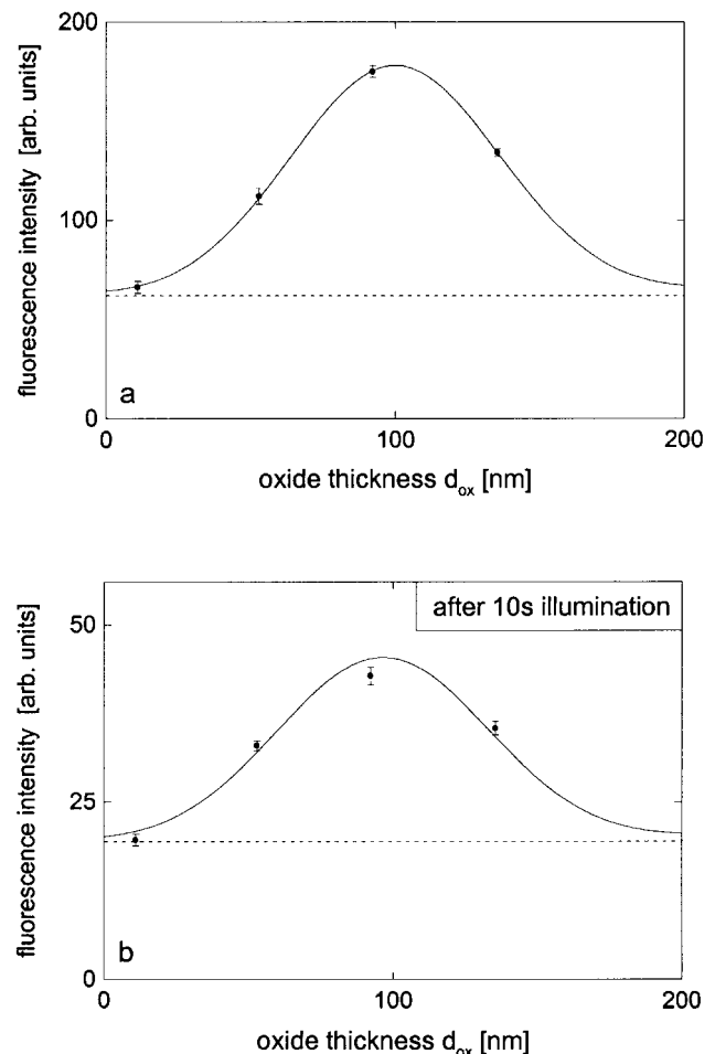
Fig. 9. Effect of photobleaching. Fluorescence intensity (mean and \pm\sigma -value) versus thickness d_{\text{ox}} of oxide without (upper figure) and with photobleaching (lower figure). The theory is fitted with a distance d_{\text{cleft}} = 12.2 nm (stochastic error \pm 0.3 nm) without bleaching and with d_{\text{cleft}} = 16.0 nm (stochastic error \pm 3.5 nm) after bleaching
