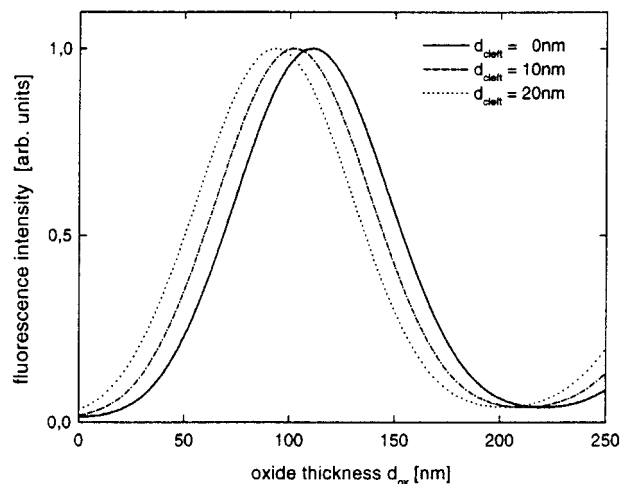
Fig. 5. Theory. Relative fluorescence intensity of the dye DiIC 12 in a cell membrane versus thickness d_{ox} of silicon dioxide for the distances d_{cleft} = 0, 10, 20 nm between membrane and silicon dioxide
