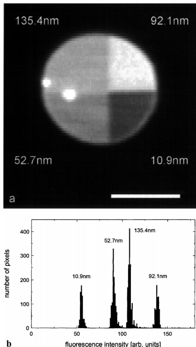
Fig. 7a,b. Fluorescence of a single ghost. a Image taken by a CCD-camera. The thickness of the four oxide layers is indicated. The scale bar is 5 \mu\text{m} . (The bright spots are dye crystals.) b Histogram of fluorescence intensity on the four regions. The number of pixels with a certain intensity is plotted versus the intensity in 8-bit resolution
