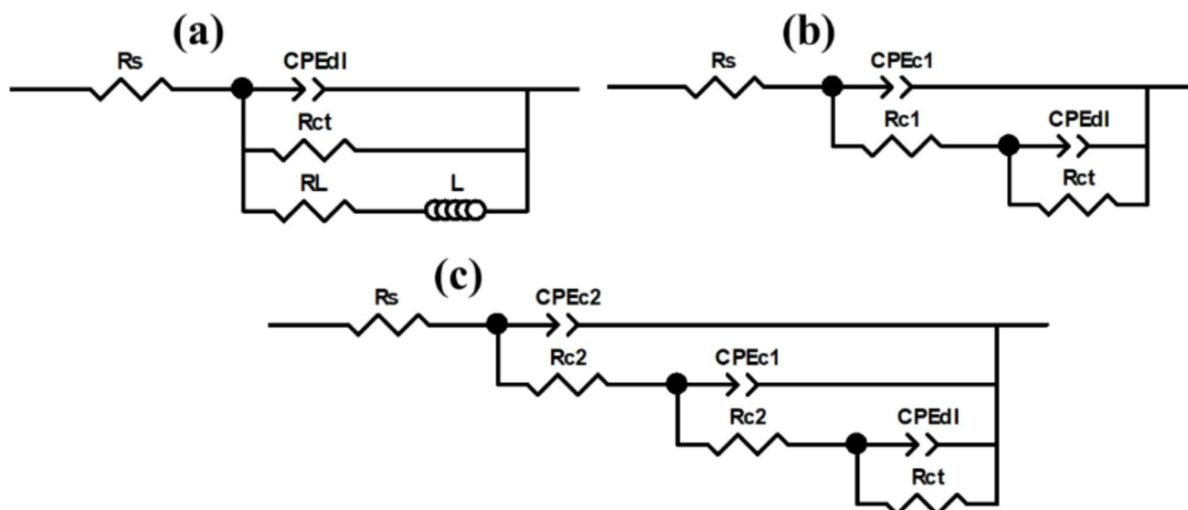
Fig. 5 Electrical equivalent circuits used to fit electrochemical impedance data of (a) the AZ91 alloy substrate, (b) the PEO-coated sample, and (c) the PEO/PDMS-nBG-coated sample
