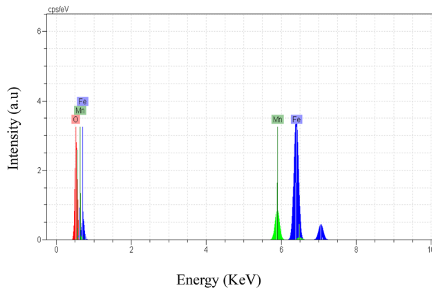
Fig. 5 EDX spectrum of \text{MnCe}_x\text{Fe}_{2-x}\text{O}_4 with x=0.0
