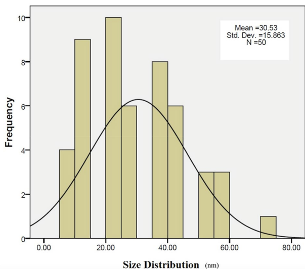
Fig. 3 Size distribution obtained from FESEM images of \text{Ce}_{1.4}\text{MnFe}_{0.6}\text{O}_4 nanoparticles
