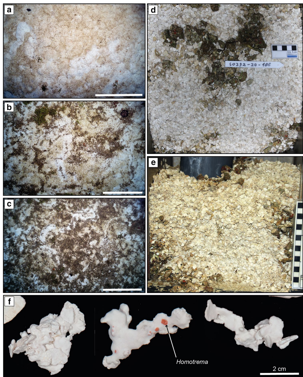
Fig. 5 Halimeda rudstone (OFOS station 09–1). A–C Surface variability in the amount of stained coated grains (mostly sponges and bryozoan) on the seafloor surface. Scale bar 1 m. D Close-up of the surface retrieved by a box corer on the Halimeda rudstone (SO292_20-1BC). Darker material is encrustations of sponges and bryozoans. E Sediment retrieved by box corer on the Halimeda rudstone. F Colonial foraminifera Homotrema encrustations on Halimeda segments
