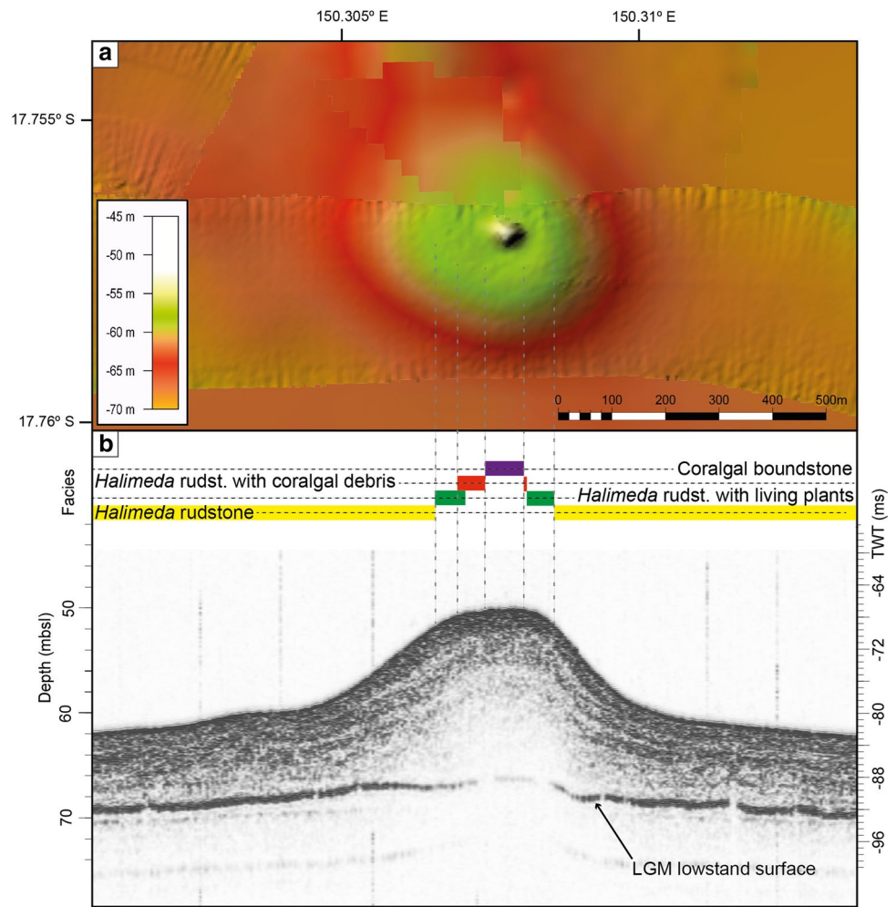
Fig. 4 Profile Bioherm East (OFOS station 09–1). A Multibeam bathymetry map. B Parasound profile with surface facies distribution. LGM, last glacial maximum
