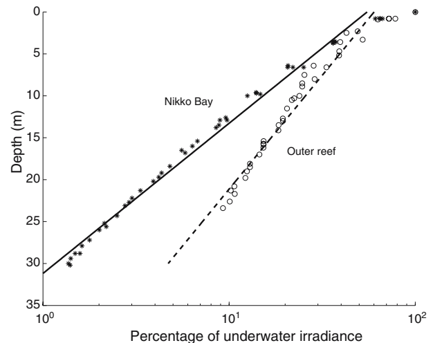
Fig. 4 Attenuation of scalar irradiance at two habitats, Nikko Bay Site 1B and (2) Outer Eastern Reef Site 3E, Palau, using a Photosynthetic Active Radiation sensor, Biospherical Instrument Inc., Model number, QSP-170; data were taken on 22 February 2005 during cloud free conditions. Regressions of the form E_o(Z) = E_o(0)e^{-K_o Z} were fitted to the data at each site, where K_o is the vertical attenuation coefficient for scalar irradiance, and E_o(Z) and E_o(0) are the scalar irradiance at Z meters depth and just below the surface respectively. K_o for Nikko Bay was 0.129 and for the Outer Eastern Reef Site 0.085
