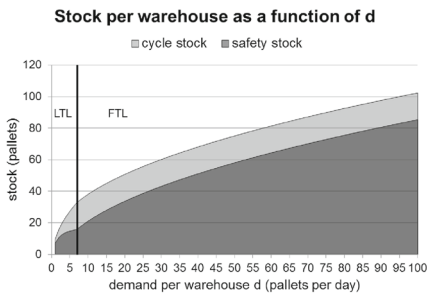
Fig. 4 Safety stock and cycle stock for continuous review and gamma distributed demand. Common data: Q = 34 [pallets], L = 2, t_{max} = 5 [days]
