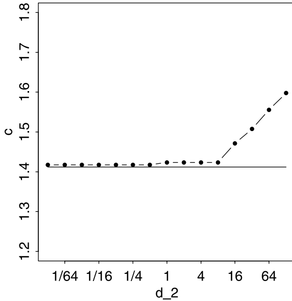
Fig. 1. Numerical calculation of spreading speed for Lotka-Volterra competition model. Parameter values are a_1 = 2/3 , a_2=4/3 , r_1 = r_2 = 1 and d_1 = 1 . The parameter d_2 varies on a log scale. The solid line shows \bar{c} = \sqrt{2} and dots show numerically calculated values for c^* . The numerical solution method uses the method of lines and Gear’s method with 4000 spatial grid points.
