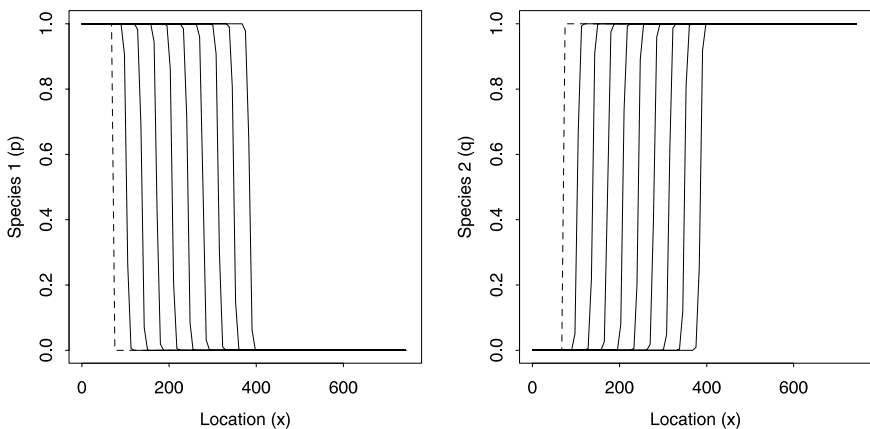
Fig. 2. Numerical simulation of Lotka-Volterra competition model. Parameter values are a_1 = 2/3 , a_2=4/3 , r_1 = r_2 = 1 and d_1 = d_2 = 1 . Dashed lines show initial conditions. Solutions are given every 25 time units, and are denoted by the solid curves.
