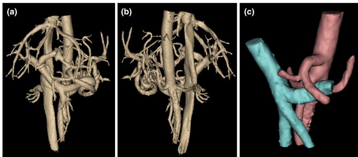
Fig. 1 Phase contrast (PC) angiograms of the mesenteric vasculature created from 4D flow MRI complex difference data. Anterior (a) and posterior (b) views of the segmented angiogram for a healthy (61-year-old, male) control subject. Note the high vascular detail.
