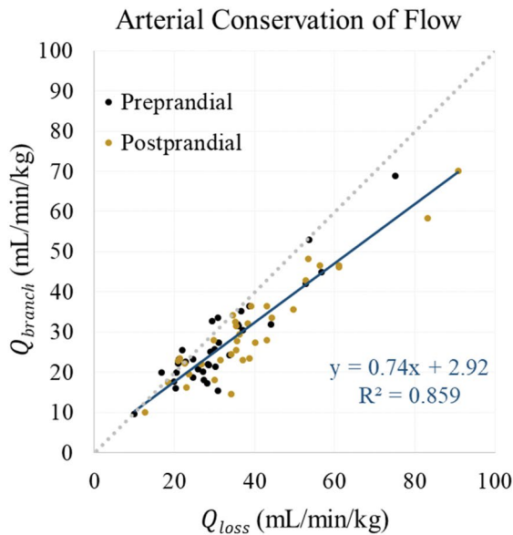
Fig. 4 Correlation analysis of venous and arterial flow measurements. (Left) Difference in blood flow between SCAo and IRAo measurements ( \bar{Q}_{loss} ) plotted against the sum of flow from all branching arteries between the measured SCAo and IRAo segments ( \bar{Q}_{branch} ).
