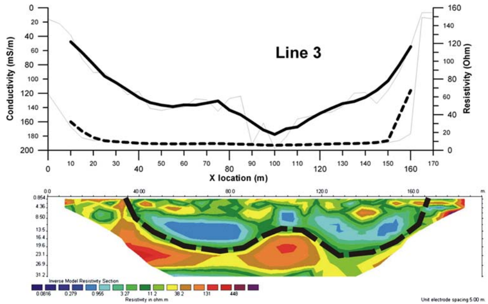
Fig. 6 Surface geophysical data for EM-3 ( upper figure ) and ERT-3 ( down figure ) profiles in Fodele landfill. Black solid line and dashed line represent the variation of inductive terrain conductivity and resistivity, respectively, along the profile and the dashed thick black line shows the boundary between the deposited wastes in the landfill and the bedrock. Thin line indicates the raw measured data and the thick solid line shows the filtered/smoothed model
