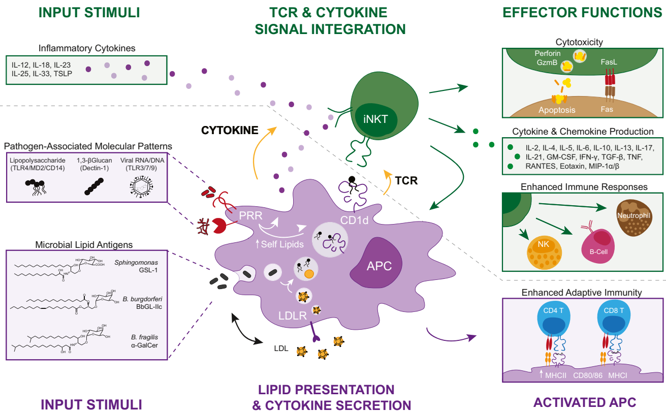
Fig. 1 Mechanisms of iNKT cell activation
