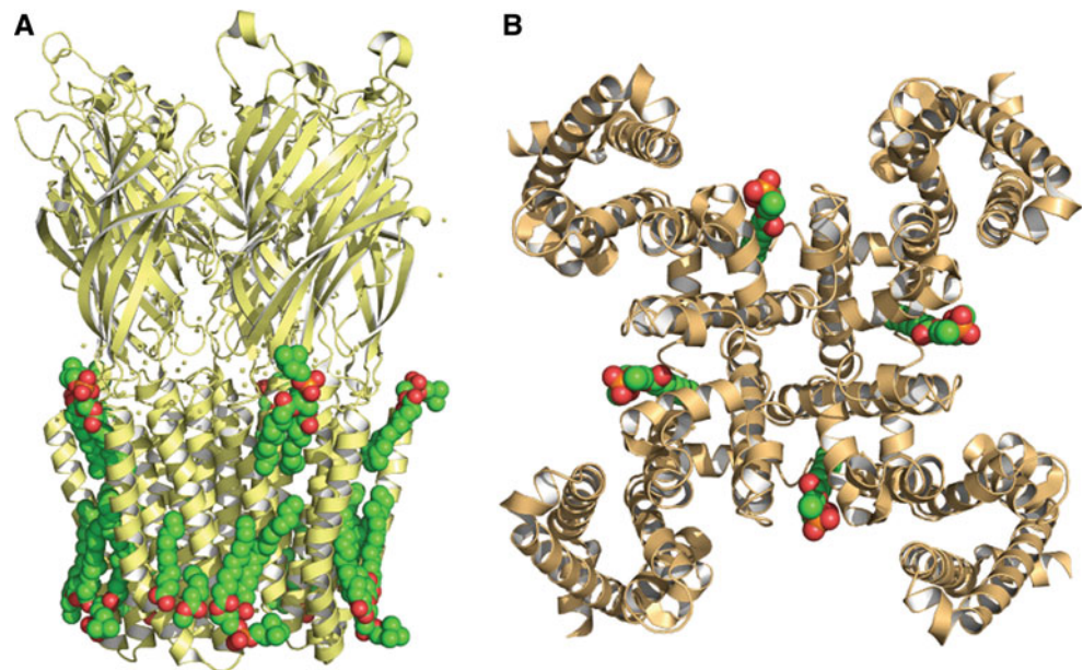
Fig. 10 Native-like bound lipids and detergents in the crystal lattice shown with space-filling atoms . a In the ligand-gated ion channel (PDB: 3EAM) a large number of diacyl lipids diffract in an annulus around the protein. b For the voltage-gated Na + channel (3RVY) one monoacyl detergent is bound per monomer in a crevice at the monomer junctions, thought to be a lipid binding site
