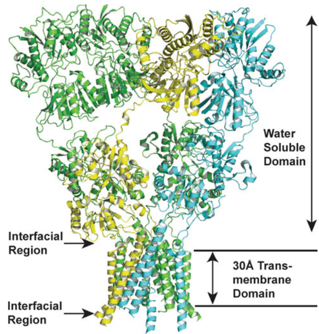
Fig. 1 Membrane proteins may have significant extramembranous portions that behave much like soluble proteins, and can receive signals from the extracellular environment and transmit them to the intracellular side through a membrane-embedded, close-packed \alpha -helical domain, as with an ionotropic glutamate receptor (PDB: 3KG2) (Sobolevsky et al. 2009). This review focuses on the native-like structure of the transmembrane domain of helical membrane proteins
