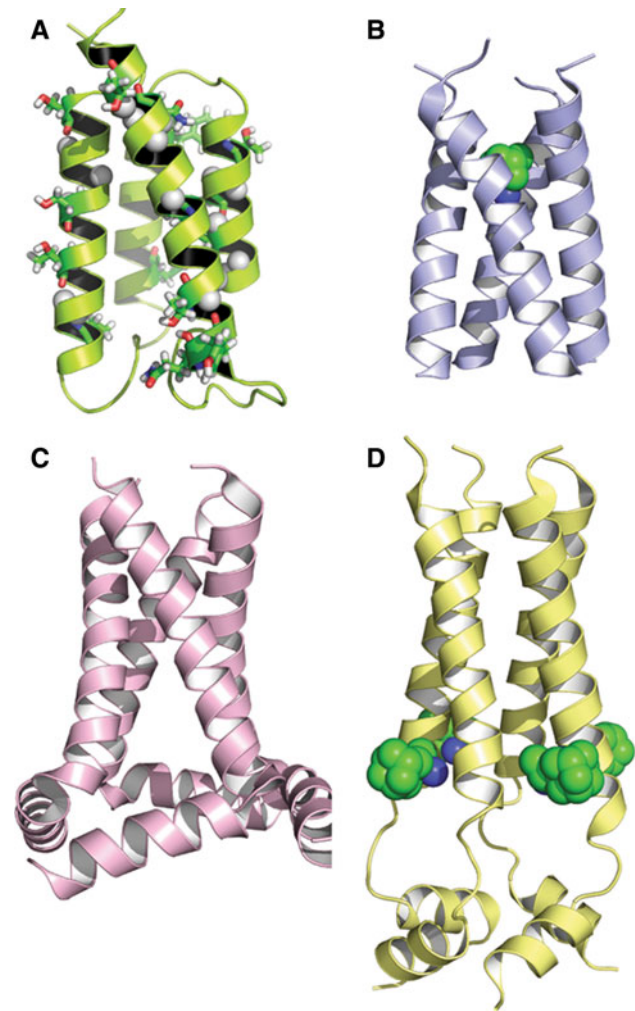
Fig. 9 Hydrophobic match of the membrane environment with the protein TM domain. a The histidine kinase receptor KdpD (2KSF) displays a short helix as well as numerous hydrophilic residues on the external surface of the helical bundle, leading to considerable H/D exchange ( white space-filling amide protons indicate sites that H/D exchange). b–d Influenza A M2 protein structures. b The TM domain characterized in lipid bilayers with amantadine bound in the pore (2KQT), displaying helical lengths that span the hydrophobic region of the membrane. c The conductance domain of M2 (residues 22–62; 2L0J), displaying very similar helical tilt angles to that of 2KQT. d The M2 conductance domain in DHPC micelles (2RLF), displaying helices with a small tilt angle and drug ( green space-filling ) on the external surface of the protein
