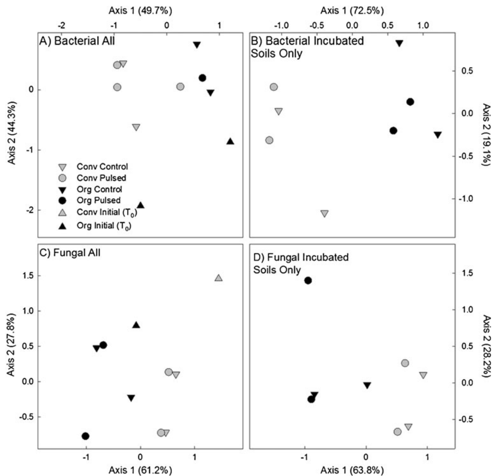
Fig. 1 Bacterial and fungal NMS ordination plots. The x - and y -axes represent the two axes that best summarize the community composition based on TRF relative abundance, and numbers in parentheses by the axes are the amount variation in community structure represented by the respective axis. a, b patterns of bacterial community TRFs and c, d patterns of fungal community TRFs. b, d Bacterial and fungal NMS run without the T_0 sample in the analysis. In all panels, management significantly differentiated communities (PerMANOVA, p < 0.05 ), but carbon treatment did not. a, c T_0 samples were also different from incubated samples within managements (PerMANOVA p < 0.05 )
