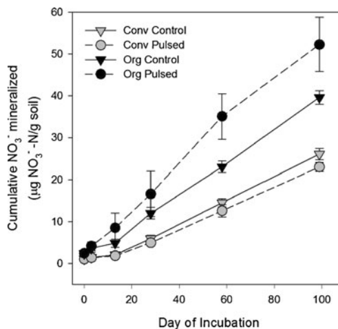
Fig. 5 Cumulative soil mineralization (only nitrate detectable). Black symbols indicate organic and grey symbols conventional management; triangles are deionized water controls, circles are pulsed ^{13}\text{C} glucose incubations. Organically managed soils produced more \text{NO}_3^- than conventional ( p<0.05 ), and organically managed soils with pulsed substrate addition mineralized more N than controls ( p<0.05 )
