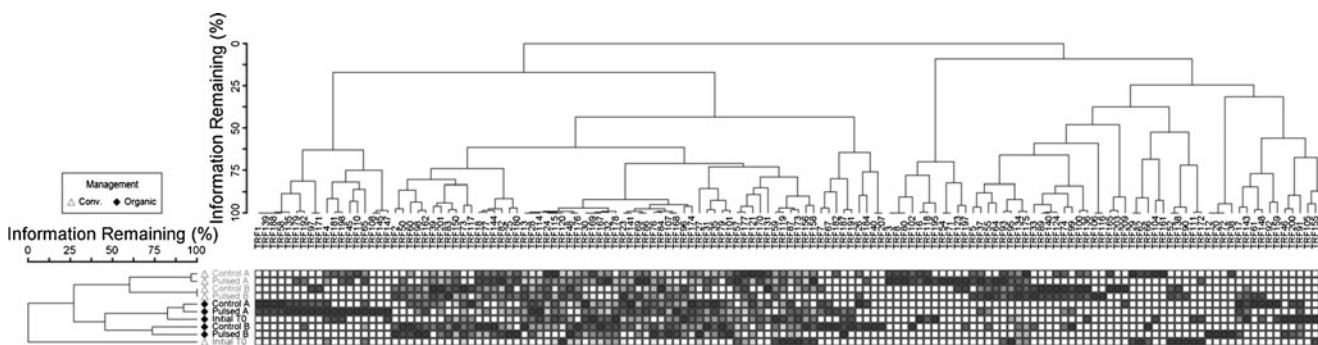
Fig. 3 Two-way cluster analysis of fungal community TRFs. Shading of cells indicates relative abundance of each TRF in each plot, management, and treatment with white indicating absence and darker colors indicating increasing relative abundance. TRFs that cluster
