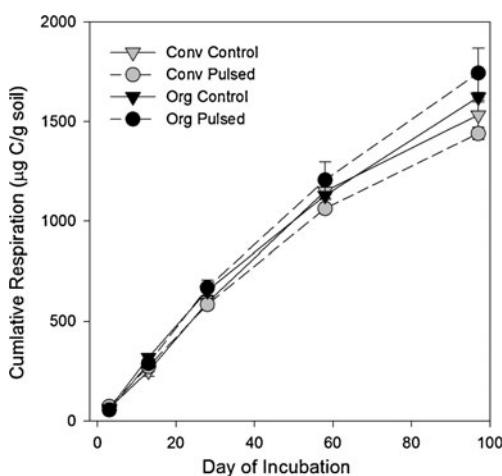
Fig. 4 Cumulative soil respiration during incubation. Black symbols indicate organic and grey symbols conventional management; triangles are deionized water controls, circles are pulsed ^{13}\text{C} glucose incubations
