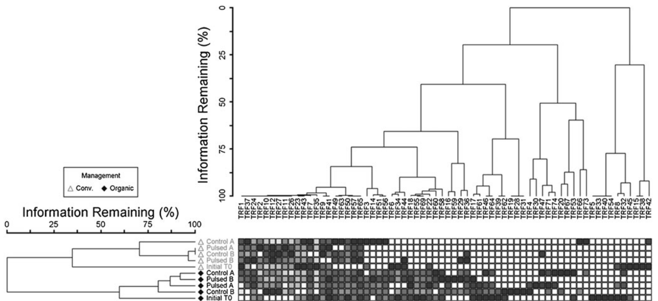
Fig. 2 Two way cluster analysis of bacterial community TRF relative abundance. Shading of cells indicates relative abundance of each TRF in each plot, management, and treatment with white indicating absence and darker colors indicating increasing relative abundance. TRFs that
