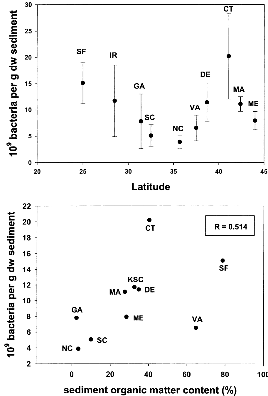
Figure 2. Distribution of the abundance of sediment bacteria by latitude (top) and by the percentage of organic matter present in the sediments (bottom).
