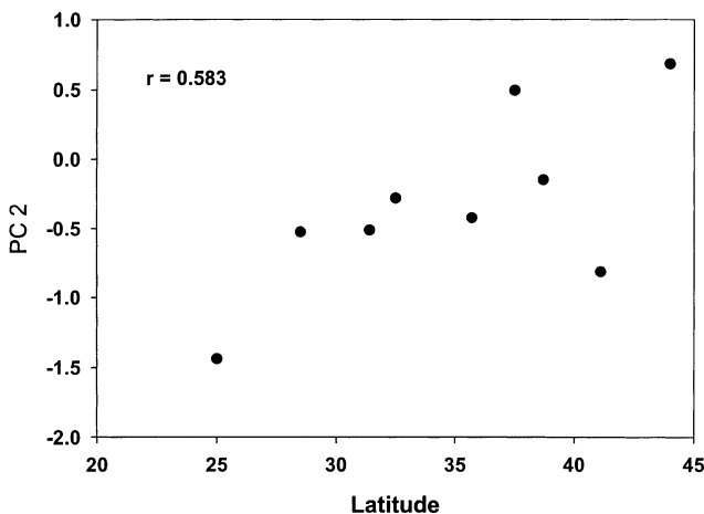
Figure 4. Distribution of PC2 values for bacterial sediment community composition (from Fig. 3) with latitude to display latitudinal gradient in community composition of the sediment. The correlation between the variables was r = 0.583 .
