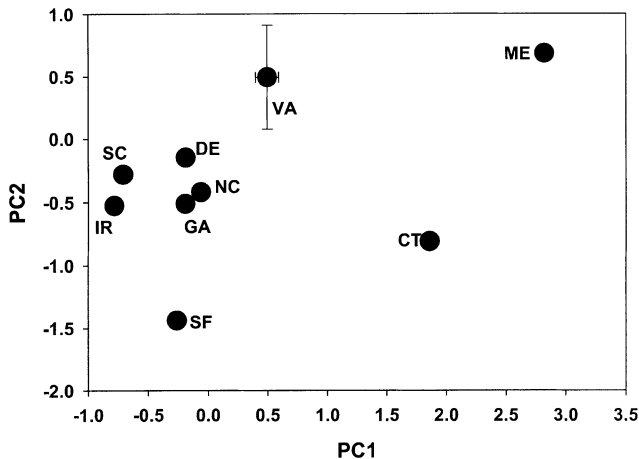
Figure 3. Principal components analysis plot of sediment-bacteria community composition patterns obtained from TRFLP analysis of whole-community DNA extracts amplified with the primer set 27f_6FAM:1492r.
