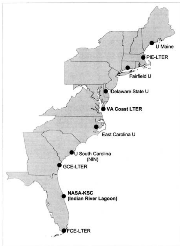
Figure 1. Location of participating sites. Dominant high-marsh plants (standing dead) and sediments were collected from each of the sites in late fall–winter of 2000–2001.
