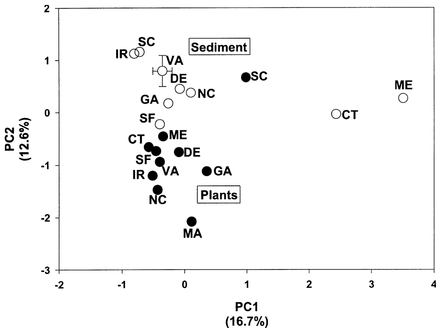
Figure 7. Comparison of plant-associated and sediment-associated bacterial communities showing the distinct differences between the two habitats. Open circles are sediment data; closed circles are plant data.
