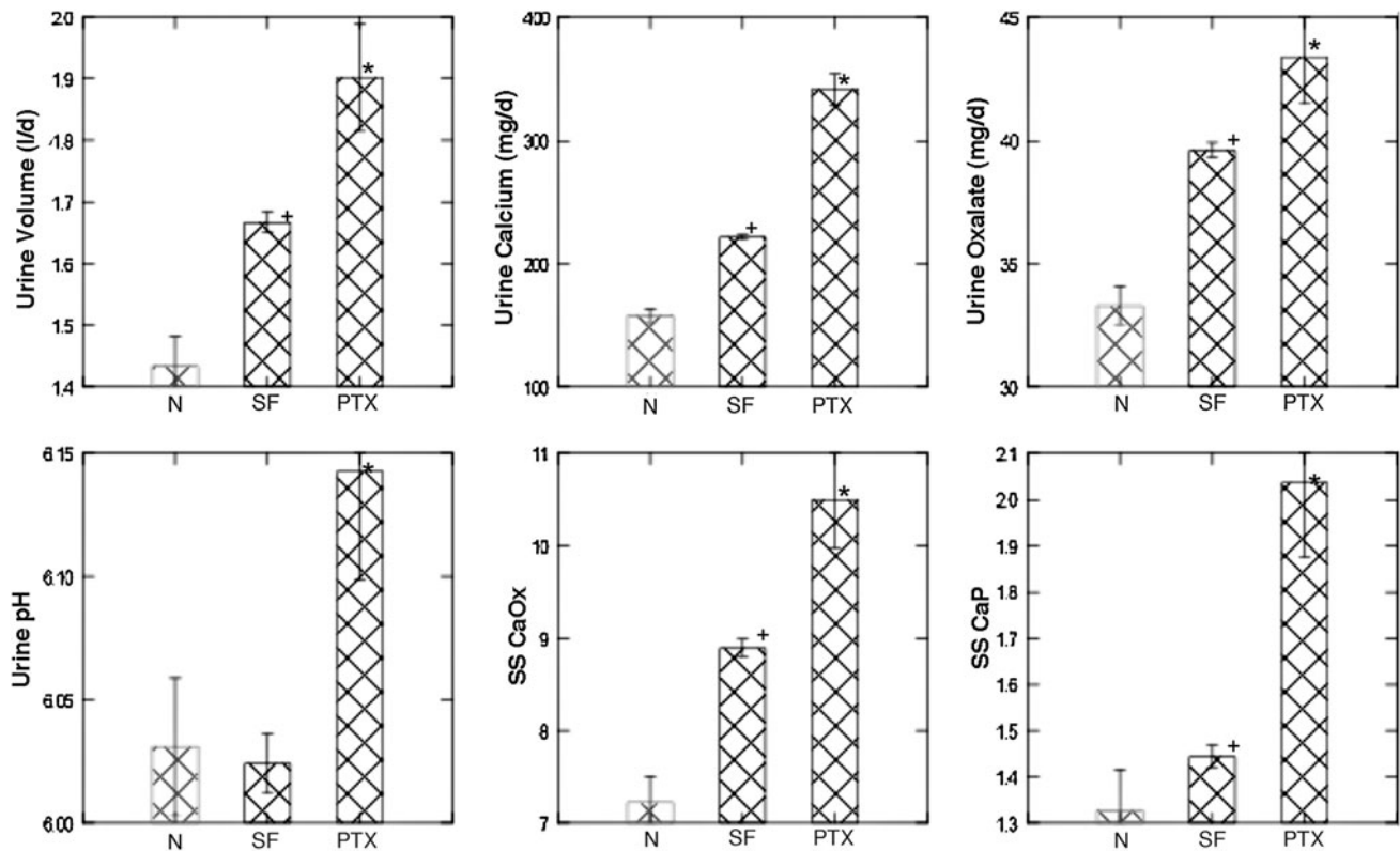
Fig. 12 Urine abnormalities in primary hyperparathyroid stone formers (PTX). Compared to ICSF and normals (SF and N on X axes of all panels) PTX showed higher urine volume, calcium and oxalate excretion, and especially urine pH and SS CaP. This was true
