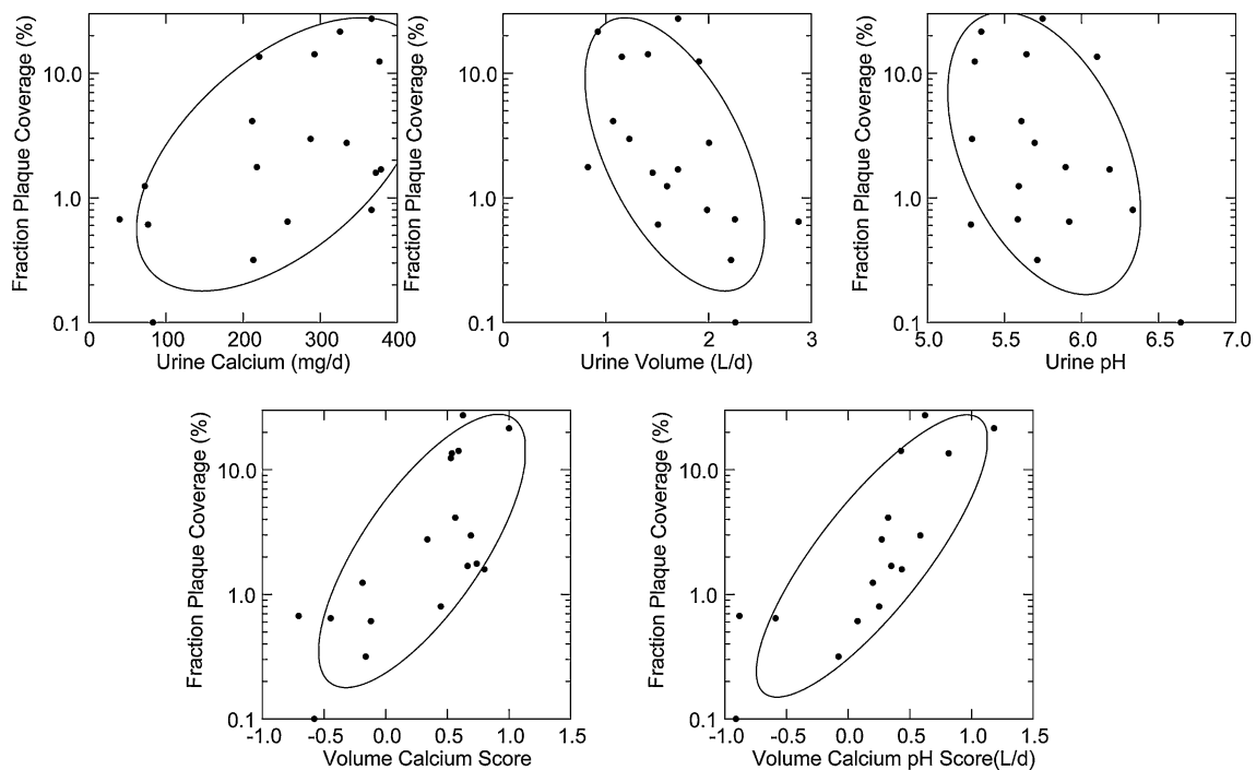
Fig. 5 Relationship between plaque abundance (y-axes of each panel) and urine measurements. Plaque area is proportional to urine calcium excretion and inverse to volume and pH ( upper panels );
