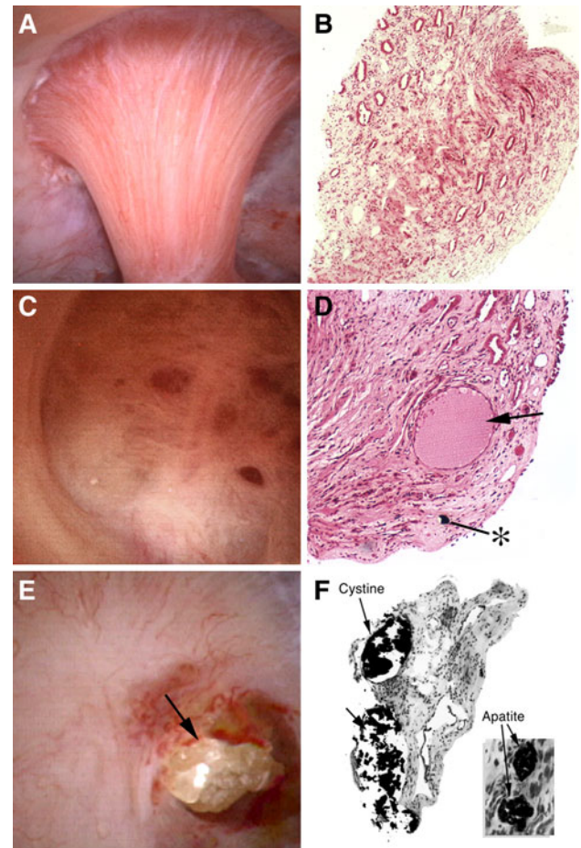
Fig. 14 Endoscopic and histologic observations of stone formers with cystinuria. Papillary morphology varied in these patients with some appearing normal ( a ) to distorted with flattening and greatly dilated opening of ducts of Bellini ( c ). Protruding plugs of cystine were noted in some dilated ducts (arrow, e ). Histopathology confirmed the observations seen by endoscopy, in that, tissues from papillary biopsies appeared normal ( b ) to abnormal characterized by extensive inner medullary plugging with ( f ) and without mineral deposits ( d ). An occasional mineral plug was noted in loops of Henle (asterisk, d ). Intraluminal plugs of the ducts of Bellini were primarily cystine in nature while deposits in inner medullary and loops of Henle were always apatite ( f )
