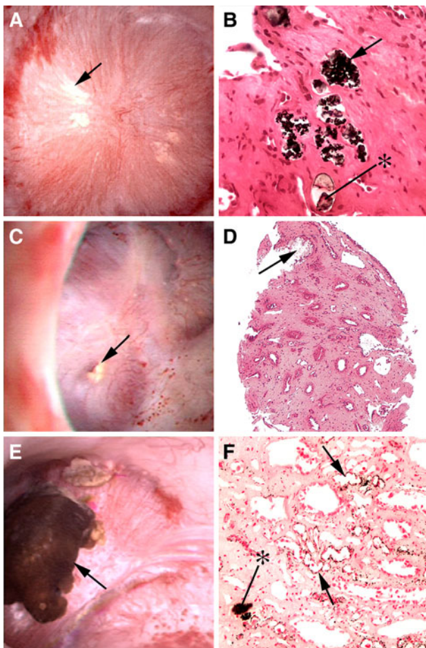
Fig. 15 Endoscopic and histologic observations of ileostomy patients with stones. Papillary morphology as observed by endoscopy varied from a normal conical shape (a) to flattened and retracted (c). Papilla show areas of white plaque (arrow, a) and plugs in opening of ducts of Bellini (arrow, c) and attached stones (arrow, e). Histopathology revealed intraluminal plugs of apatite in dilated inner medullary collecting ducts (arrows, b, f), those with a mixture of apatite and sodium acid urate/ammonium acid urate (asterisk, b) while others had only sodium acid urate/ammonium acid urate (arrow, d). Some biopsy sections contained large amounts of interstitial plaque (arrows, f)
