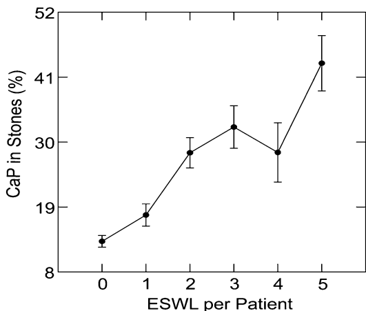
Fig. 10 Stone CaP percent versus extra-corporeal shock wave lithotripsies (ESWL). Stone CaP% rose with numbers of ESWL procedures after correcting for sex, age, number of stones, and years of stone disease
