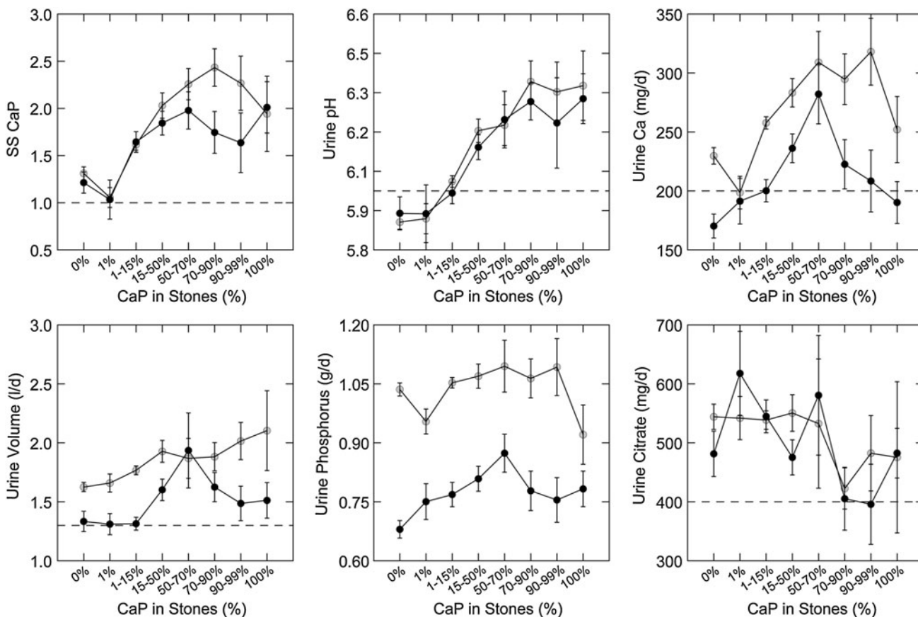
Fig. 9 Urine measurements in ICSF with increasing stone calcium phosphate (CaP) percent (men, gray circles; women, black circles). With increasing percent of CaP in analyzed stones (x-axes of all panels) SS CaP and urine pH (upper left and middle panels) rose
