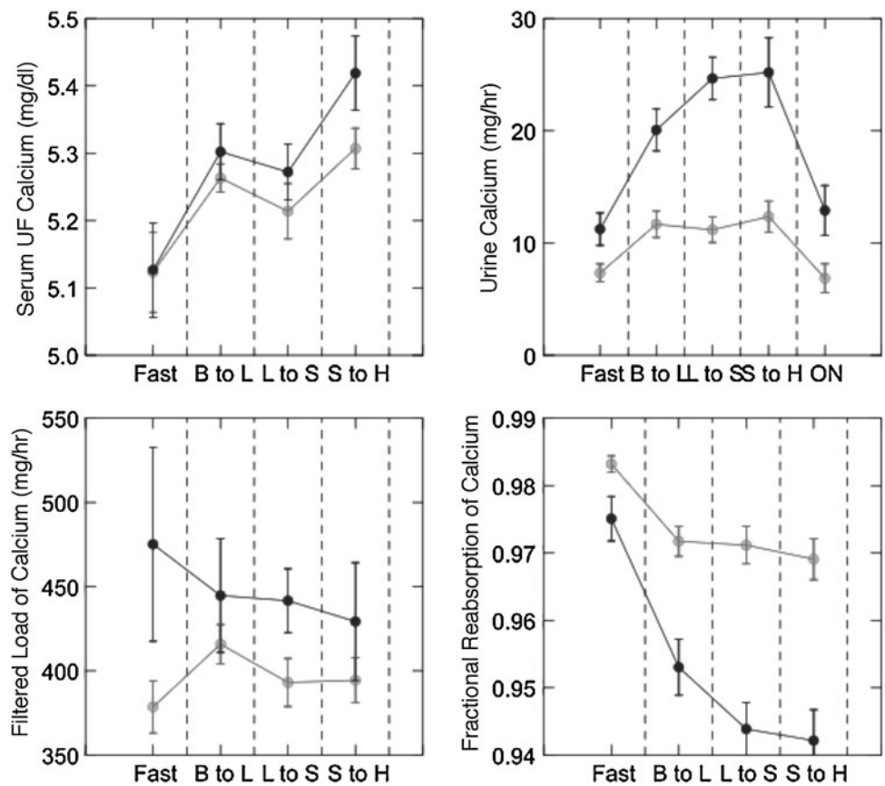
Fig. 6 Evidence for reduced tubule calcium reabsorption in ICSF. In a GCRC controlled diet three meal day, serum Ultrafiltrate calcium ( upper left panel ) rose modestly and equally in ICSF ( black circles ) and normals ( gray circles ) after breakfast (B to L) and remained high after lunch (L) and supper (S), but urine calcium rose ( upper right panel ) above normal throughout the day and overnight (ON) and tubule calcium reabsorption ( lower right panel ) fell far more in ICSF; filtered loads of calcium ( lower left panel ) did not change in either group
