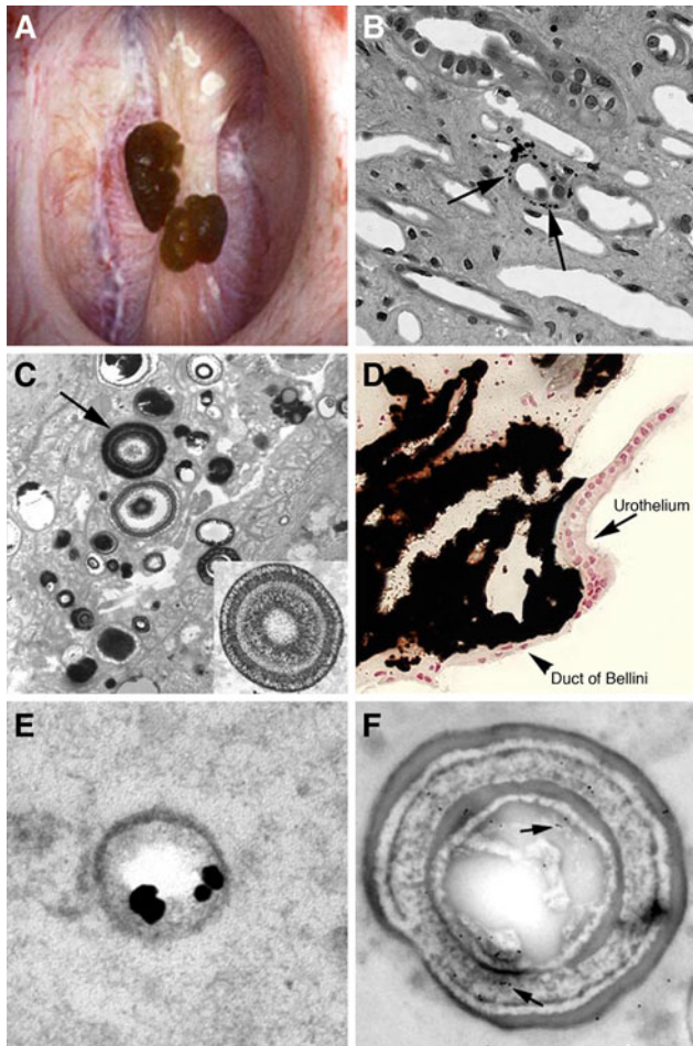
Fig. 1 Endoscopic and histologic images of Randall's plaque in ICSF patients. a Two CaOx stones attached to the papilla tip at sites of Randall's plaque as seen by endoscopy at the time of stone removal. On biopsy ( b ), tissue sections stained by the Yasue method reveals black, small, spherically shaped deposits (arrows) in the basement membrane of the thin loops of Henle, which appears to be the initiating site of plaque formation. By TEM ( c ), these deposits appear as multi-layered spheres with alternating light (crystal) and dark (matrix) bands. The smallest deposits were about 50 nm in diameter. Rather dense regions of interstitial plaque located near the papilla tip were commonly noted in ICSF patient ( d ) and at such sites crystal accumulated beneath the urothelium and around the distal ends of ducts of Bellini. Immunoelectron microscopic studies localized osteopontin immunogold particles (dark dots, e ) at the crystal-matrix boundary whereas the third heavy chain of the inter-alpha trypsin molecule (arrows f ) was detected in the matrix layer
