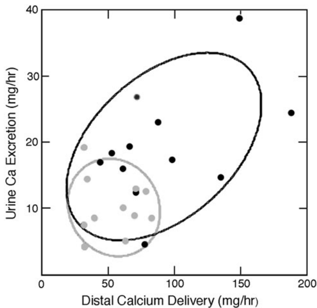
Fig. 7 Relationship between delivery out of proximal tubule and urine calcium excretion. Distal calcium delivery from proximal tubule estimated by endogenous lithium clearance was higher in ICSF ( black circles ) versus normals ( gray circles ) and highest urine calcium excretions corresponded with highest delivery. Each point is a complete study in a single individual
