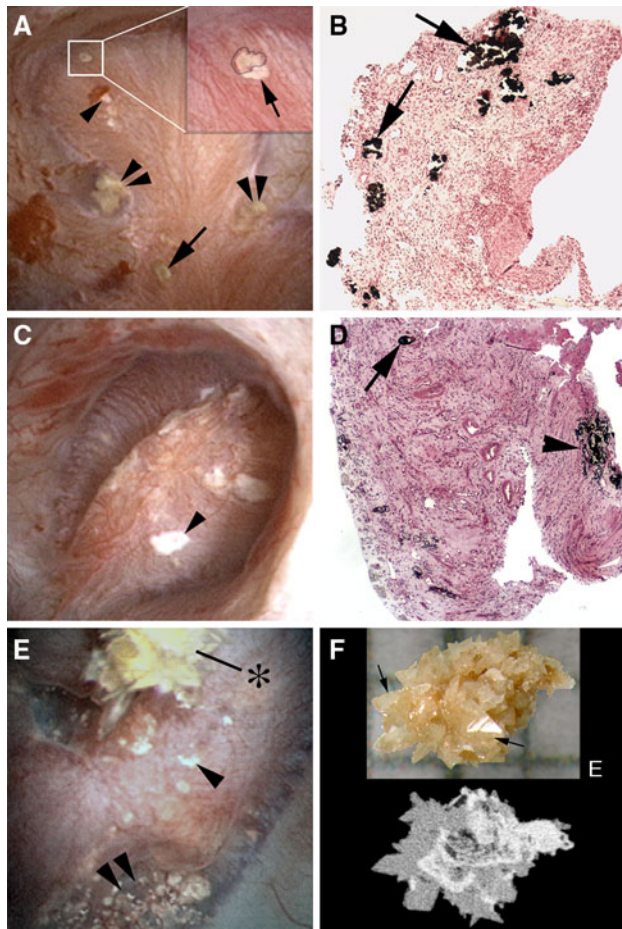
Fig. 11 Endoscopic and histologic observations of stone formers with primary hyperparathyroidism. Endoscopic evaluation of papilla from stone formers with primary hyperparathyroidism shows the coexistence of attached stones (a, within white box; e) and plugging of ducts of Bellini (a, lower single arrow) on the same papilla. In additions, regions of white plaque (arrowhead, a, c, e) and yellow plaque double arrowheads, a, e) were also seen on the same papilla. Histopathology of the papillary biopsies showed extensive regions of intratubular plugging of inner medullary collecting ducts and ducts of Bellini (arrows, b, d) with areas of interstitial plaque (arrowhead, d). Extensive interstitial fibrosis surrounded the plugged tubular segments. e An attached calcium oxalate stone (*) before while f (upper panel) shows it after detachment. Micro-CT analysis of this same stone (f, lower panel) reveals a mixture of apatite (white regions) and calcium oxalate dihydrate (gray regions)
