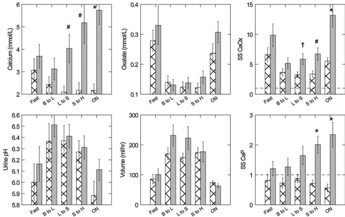
Fig. 4 Urine measurements in idiopathic calcium stone formers ICSF. Urine molarity of calcium ( upper left panel ) among ICSF ( gray solid bars ) exceed normals ( crosshatch ) in the intervals from lunch to supper (L to S), supper to home (S to H) and overnight (ON). Oxalate molarity ( upper middle panel ), urine pH ( lower left panel ),
