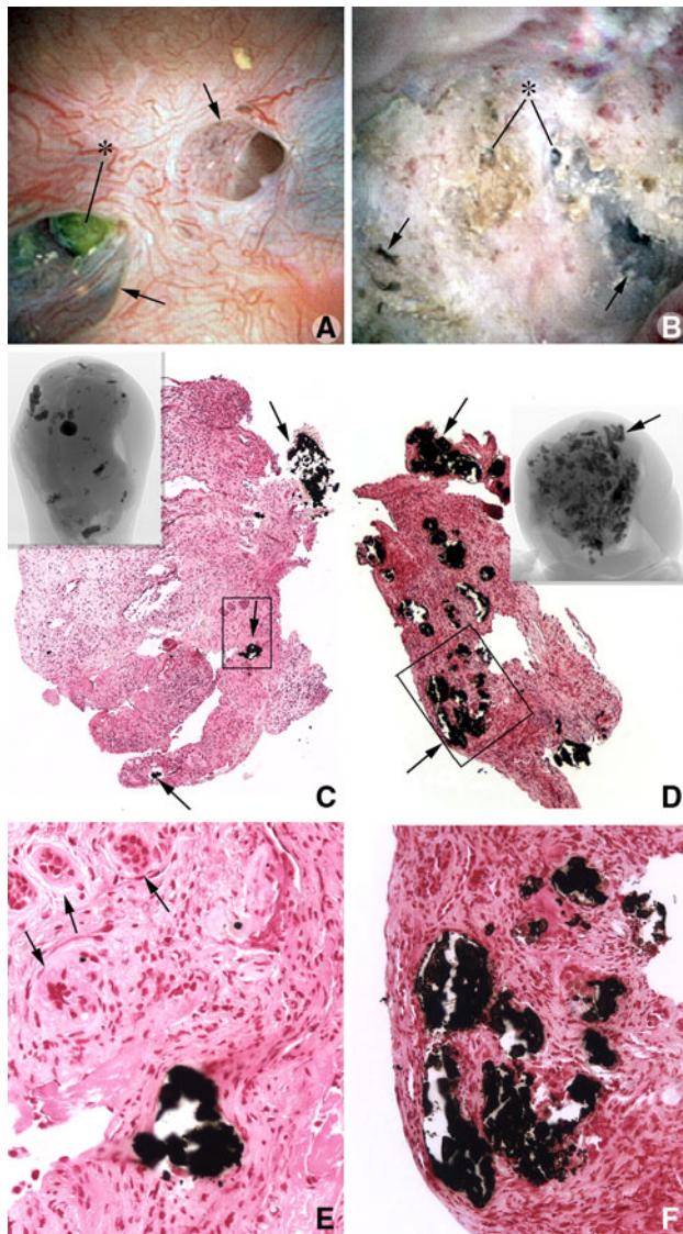
Fig. 13 Endoscopic and histologic observations of stone formers with renal tubular acidosis. Appearance of papillae varied from normal papilla apart from an occasional dilated duct of Bellini (arrows, a ) to severely flattened and fibrotic with pitted appearance (arrow, b ). These papilla possess multiple dilated ducts of Bellini, some with protruding mineral plugs (asterisk, a , b ). Histopathology and micro-CT imagery shows a range of abnormalities. Plugging of inner medullary collecting ducts varied from minimal in number of tubules involved and size of deposits (arrows, c ) with some interstitial fibrosis (arrows, e ), to extensive plugging (arrows, d ), loss of tubular cells and dense cuffs of fibrotic tissue ( f )
