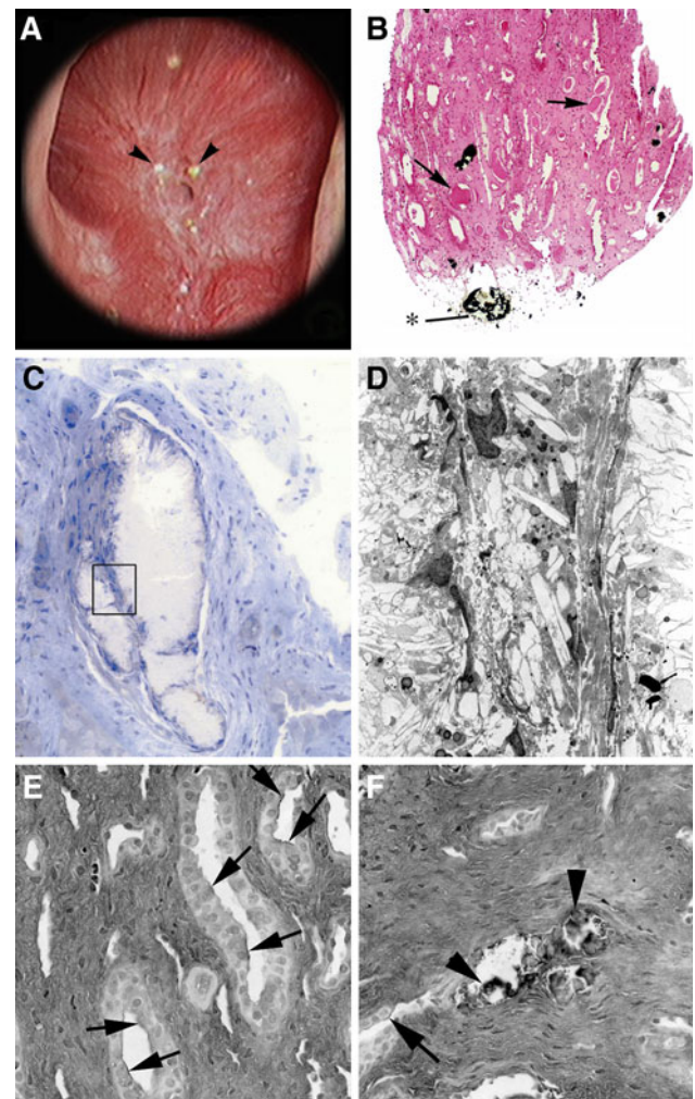
Fig. 16 Endoscopic and histologic observations of stone patients with bypass surgery for obesity. Endoscopic observations revealed normal appearing papilla except for an occasional dilated opening of a duct of Bellini with adjacent nodular-appearing structures (arrowheads, a). Histopathology shows an occasional intraluminal deposit in an inner medullary collecting duct and plugs in the ducts of Bellini (asterisk, b). A few dilated inner medullary collecting ducts possessed cast material and regions of fibrosis (arrows, b). At a higher magnification (c), a site of intraluminal plugging reveals a loss of tubular lining cells and cuffs of interstitial fibrosis. A region within c (see rectangle) is further magnified in d with transmission electron microscopy. There is a complete loss of cellular detail. Biopsy sections from stone patients with bypass surgery for obesity were also stained for hyaluronan to detect sites of cellular injury. A number of inner medullary collecting ducts with (arrowheads, f) and without mineral deposits showed focal regions of hyaluronan staining of their apical cell membranes (arrows, e, f)
