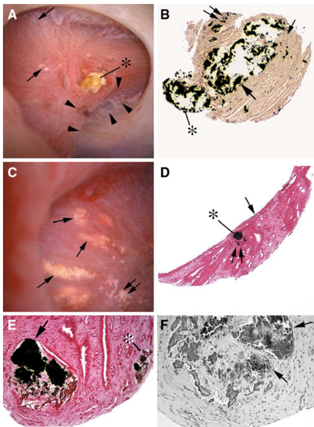
Fig. 8 Endoscopic and histologic observations of brushite stone formers. Brushite stone formers have unique papillary characteristics in that they possess white and yellow plaque as well as protruding plugs from ducts of Bellini. Although the papilla from brushite stone formers have sites of white plaque ( arrows in a and double arrow in c ), the most prominent features are mineral plugs protruding from dilated ducts of Bellini ( asterisks in a, b ) and radially oriented sites of yellow plaque ( single arrows in c ) shown to be localized to inner medullary collecting ducts ( asterisk, d ) just beneath the urothelium ( arrow, d ). Many of the papilla of brushite stone formers are deformed as noted by flattening, large dilated opening to ducts of Bellini ( a ) and large pits ( arrowheads in a ). Histopathology detected grossly dilated inner medullary collecting ducts and ducts of Bellini filled with mineral deposits ( arrows in b ) shown to be apatite. These dilated tubules were surrounded by interstitial fibrosis. Regions of interstitial plaque were easily found ( double arrows, b, d ). Using light microscopy of 1 \mu m thick plastic sections of decalcified papillary biopsies, extensive regions of cellular damage with mineralization were seen in inner medullary collecting ducts ( arrows, e, f ) and loops of Henle ( asterisk, e ) adjacent to normal appearing tubular segments ( e ). Extensive interstitial fibrosis is noted around these sites of tubular injury
