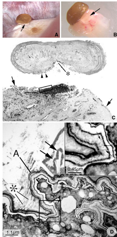
Fig. 2 Histologic examination of attached human kidney stone. During percutaneous nephrolithotomy for stone removal in a ICSF patient, two attached stones were noted on a single papillum ( a ), a clear region of Randall's plaque (arrow) is noted at the base of the larger of the two stones. b The same stone and the underlying renal tissue with interposing region of Randall's plaque (arrow) after biopsy removal of this entire complex. The entire biopsy specimen was subsequently decalcified and sectioned first for light microscopy ( c ). During the sectioning process, the stone detached from its underpinning so the two images have been approximated in this figure. A large base of interstitial plaque, stained black here by the Yasue method, and framed in part by the rectangle was in continuity with the base of the stone that also reveals a small darkly stained region (*). This region of plaque is completely devoid of its normal urothelial lining cells. Several attached epithelial cells (arrowheads) were seen at the periphery of the stone while arrows mark the site on the tissue where intact epithelial cells are seen again. The region in c marked by the rectangle was prepared and sectioned for transmission electron microscopy ( d ). In this image, the region of interstitial plaque is at the lower right and the stone in the upper left. Between these two regions is a multilayered ribbon structure (labeled A) that forms a sharp boundary. This ribbon is formed by alternating layers of five thin black organic lamina and four, white crystalline lamina (see square and its enlarge in the insert at upper right of d ). Small arrows in insert show perpendicularly oriented crystals in the white lamina. Various sized crystals (marked by asterisk and large arrows) are seen embedded in the outer matrix layer of the ribbon-like structure
