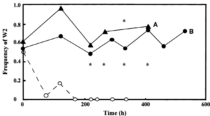
Fig. 2. Competition between the W2 and A1 genes. Each of the plasmid containing W2 gene or A1 gene of the same concentration was used to transform fresh host cells independently. The total resultant transformants from each transformation were mixed and an aliquot was used as inoculant for the chemostat run as described under Materials and Methods. Frequency of W2 was determined as follows: An aliquot of the chemostat culture was sampled at the indicated time and plated on 2xTY agar plate (12) containing 50 \mu\text{g/ml} ampicillin. The plasmids from randomly picked 26 clones per sampling were analyzed by double restriction endonuclease digestion. W2 has only the Pst I site, while A1
