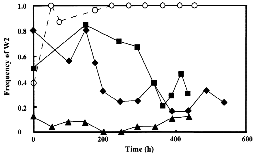
Fig. 3. Competition of the W2 gene with members of the final population of the third chemostat run. The once extinct W2 gene was mixed with the pooled genes isolated from the final population of the third chemostat run (see Fig. 1A). Frequency of the W2 gene was adjusted to 0.8 (◆), 0.5 (■), and 0.1 (▲) before mixing with the pooled genes. The three gene mixtures were introduced independently to fresh host cells and each of total resultant transformants were cultivated in three chemostat runs (◆, ■, and ▲) initiated with corresponding initial frequency of the W2 gene. Open circle (○) represents competition experiment conducted in the same manner as described above, with W2 gene frequency adjusted to 0.5 and glutamate concentration in the feeding medium reduced from 0.1 M to 10 \mu M. Frequency of W2 in the culture was determined as in Fig. 2.
