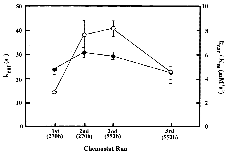
Fig. 4. Average values of the kinetic constants over the population at indicated time of the three chemostat runs. The average values were calculated from the data shown in Fig. 1B and Table 1.
