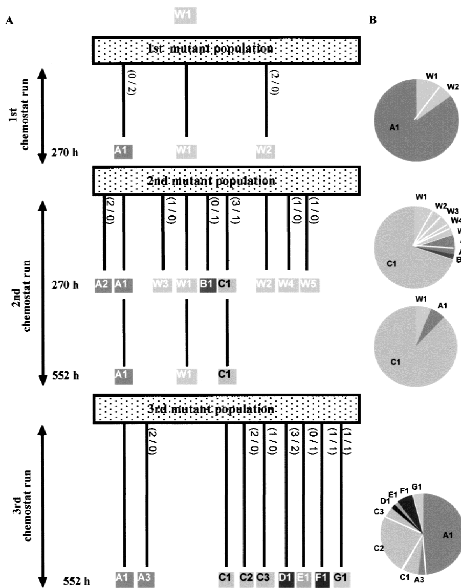
Fig. 1. Molecular evolution of glutamate synthetase. (A) Phylogenetic tree of glutamine synthetase gene. W1 denotes the wild-type gene. Paired capital letter and numerical number represents the type of mutant gene. Each letter denotes a different deduced amino acid sequence. Genes with the same letter but different number are synonymous mutants. The number of synonymous/non-synonymous mutations appears in parentheses. Double-headed vertical arrows represent the time span of cultivation. (B) Population structures at the indicated time of each chemostat run.
