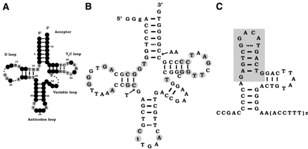
Fig. 2. A General cloverleaf structure for tRNAs (Gauss et al. 1979; Lowe and Eddy 1997). Gray circles represent conserved and semiconserved nucleotides, whereas dots represent variable sequence regions. B Predicted cloverleaf structure of tRNA-related Sauria SINE consensus sequence (tRNAscan-SE program [Lowe and Eddy 1997]). All conserved and semiconserved nucleotides
