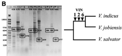
Fig. 7. A Alignment of three Sauria SINE loci and their flanking sequences in monitor lizards. The absence of these three SINE loci in the genome of Varanus salvator (VSA) and the presence of SINE sequences at orthologous genome locations in Varanus indicus (VIN) and Varanus jobiensis (VJO) support a monophyletic origin of the latter two species. A and B boxes of the tRNA-related sequence regions are shown and the clearly recognizable flanking
