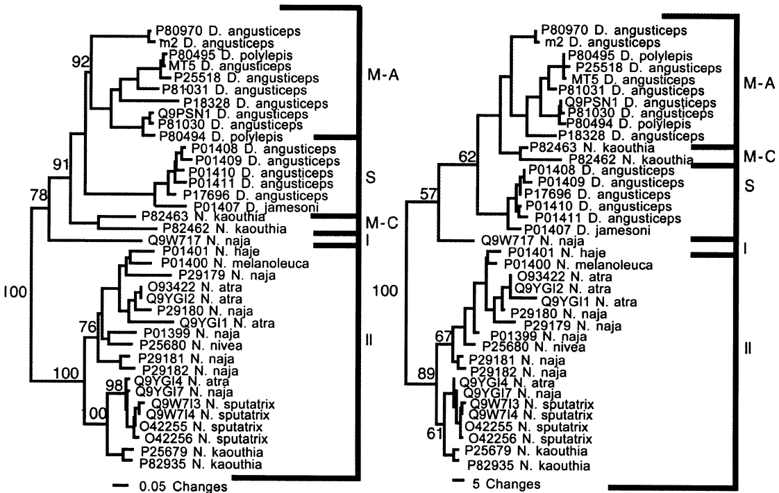
Fig. 8. Results of (A) NJ and (B) MP analysis of Type A muscarinic toxins (M-A), synergistic toxins (S), Type C muscarinic toxins (M-C), and orphan groups I and II. Only bootstrap values 50% or greater are shown. Outgroup sequences (Q14210 and P35459) were removed from the final tree image, although they were included in the analysis to root the phylogeny.
