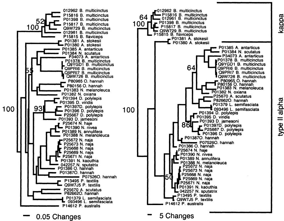
Fig. 7. Results of (A) NJ and (B) MP analysis of Type II \alpha -neurotoxins and \kappa -neurotoxins. Only bootstrap values 50% or greater are shown. Outgroup sequences (Q14210 and P35459) were removed from the final tree image, although they were included in the analysis to root the phylogeny.
