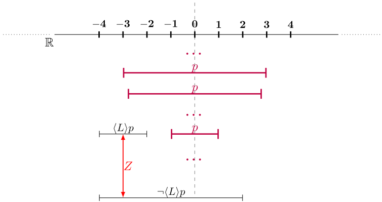
Fig. 3 \overline{\text{OBEO}} -bisimulation that violates \langle L \rangle , relative to \text{Den}
