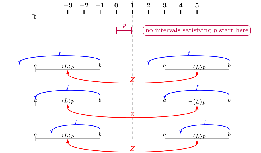
Fig. 2 \overline{\text{BEAED}} -bisimulation that violates \langle L \rangle , relative to \text{Den}
