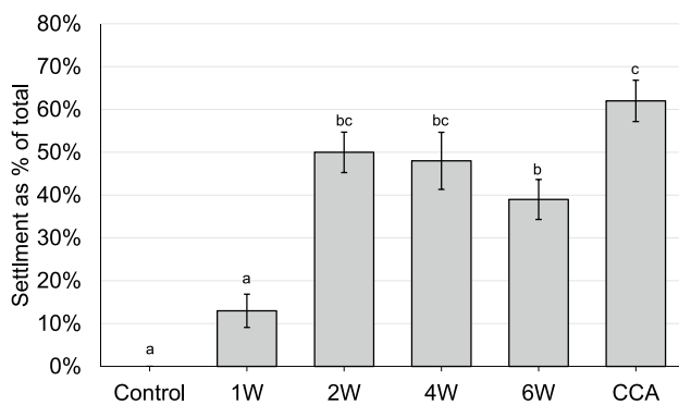
Fig. 2 Settlement of Diadema antillarum larvae exposed to a biofilm of one, two, four and six W (week(s)) old, CCA and a control with no cues, expressed as mean percentage of total \pm SE (each treatment had n=10 petri dish replicates, each containing 10 competent larvae). Treatments sharing the same letter do not differ significantly ( P>0.05 )
