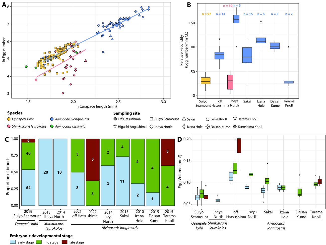
Fig. 4 Comparison of reproductive features between alvinocaridid species from hydrothermal vents fields off Japan. n : number of individuals for each condition. A Variation of \log_e -transformed minimum realized fecundity with \log_e -transformed carapace length. B Fecun-
