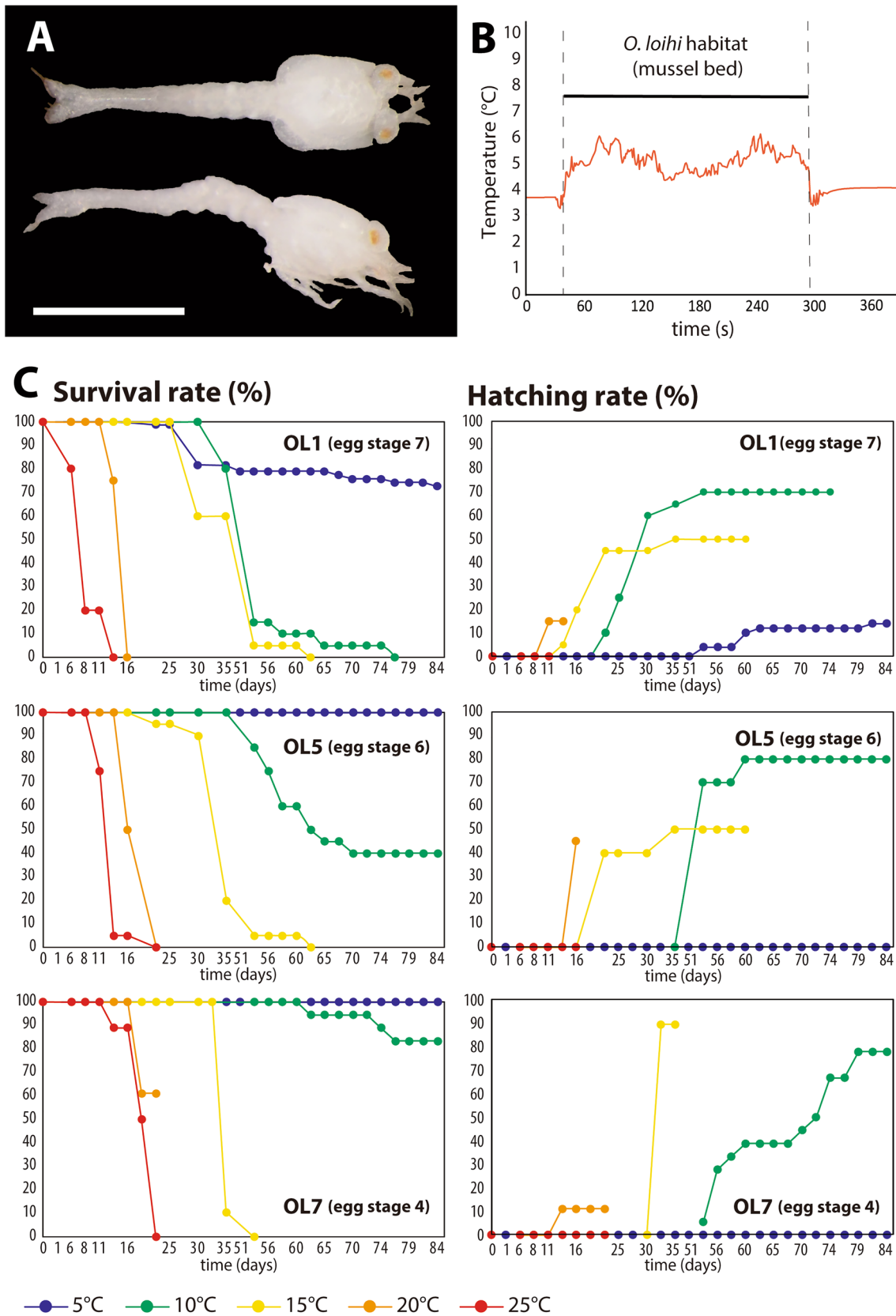
Fig. 5 Culture experiment of Opaepale loihi egg broods under different temperature conditions. A Hatched larva of O. loihi in dorsal and sagittal view. B Temperature measurement within the habitat of O.
