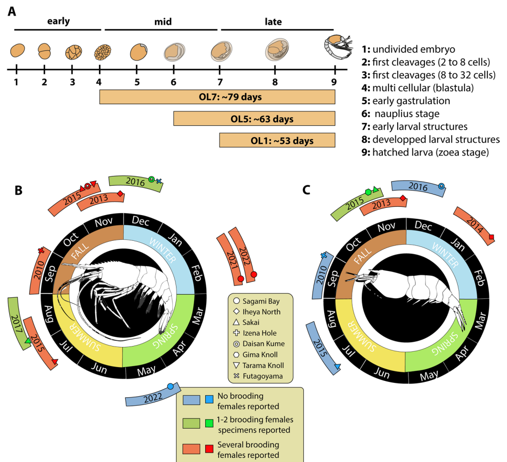
Fig. 6 Perspectives on the reproductive periods and the brooding duration of alvinocaridid shrimps inhabiting chemosynthetic ecosystems around Japan A. Duration of the embryonic development estimated by rearing experiments at 10 °C B. Diagram summarizing the occurrence of reproductive stages of Alvinocaris longirostris according to the year period C. Diagram summarizing the occurrence of reproductive stages of Shinkaicaris leurokolos according to the year period
