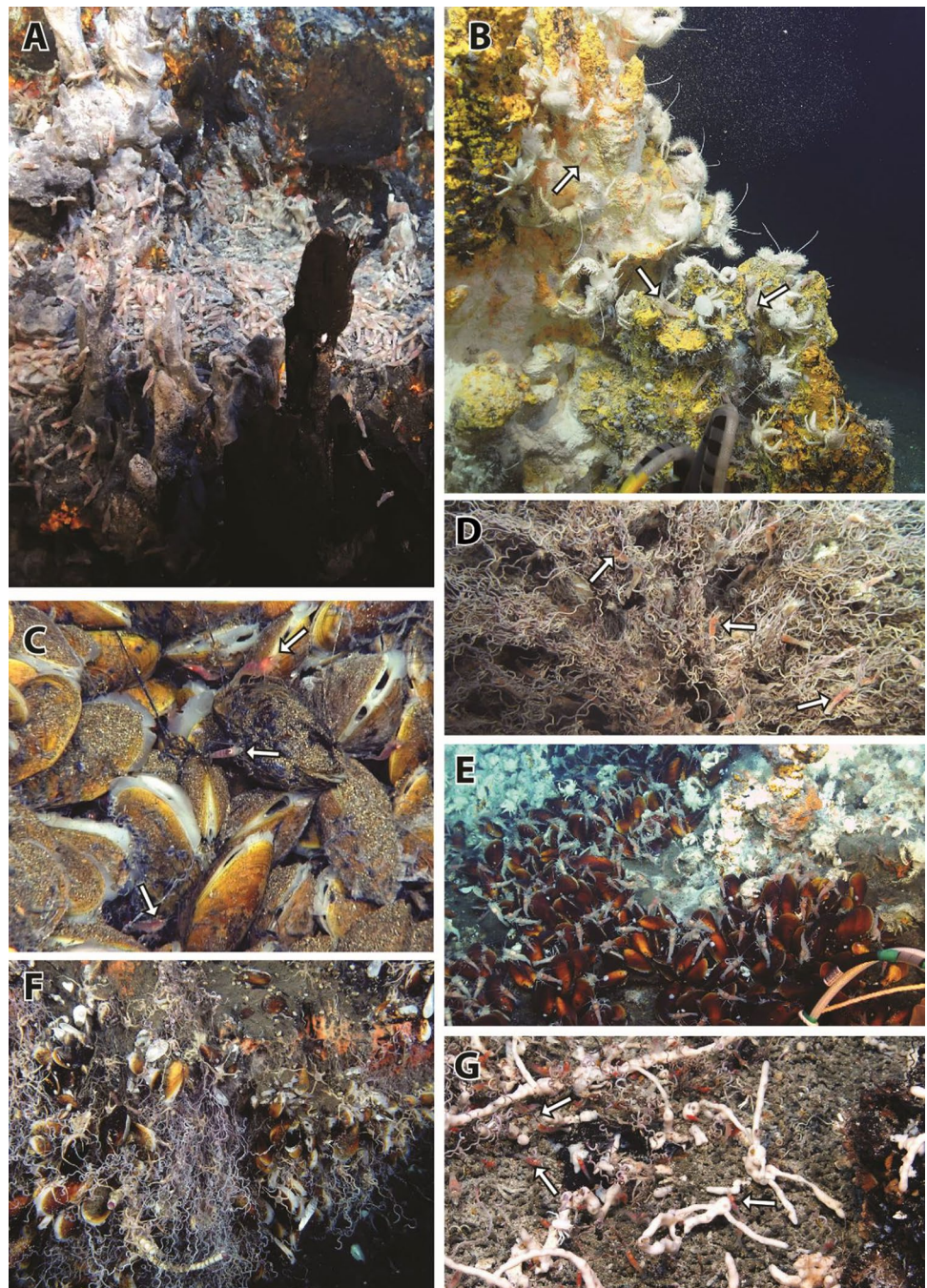
Fig. 3 Overview of the different assemblages from hydrothermal vent fields and seeps off Japan where alvinocaridid shrimps could be collected. A Aggregation of Shinkaicaris leurokolos near vent fluid exits at the Yokosuka site, Okinawa Trough. B Alvinocaris longirostris on chimney rocks in close vicinity with Shinkaia crosnieri squat lobsters at the Daisan Kume Knoll, Okinawa Trough. C Opaepele loihi within a Bathymodiolus septemdiarum mussel bed at Suiyo Seamount, Izu-Ogasawara Arc. D Alvinocaris spp. on a tubeworm bush at Sakai field, Okinawa Trough. E Alvinocaris longirostris on a mussel bed at Futagoyama field, Okinawa Trough. F Alvinocaris longirostris hidden in a tubeworm bush at the Off Hatsushima seep, Sagami Bay. G Alvinocaris longirostris within a branching sponge colony at Tarama Knoll, Okinawa Trough
