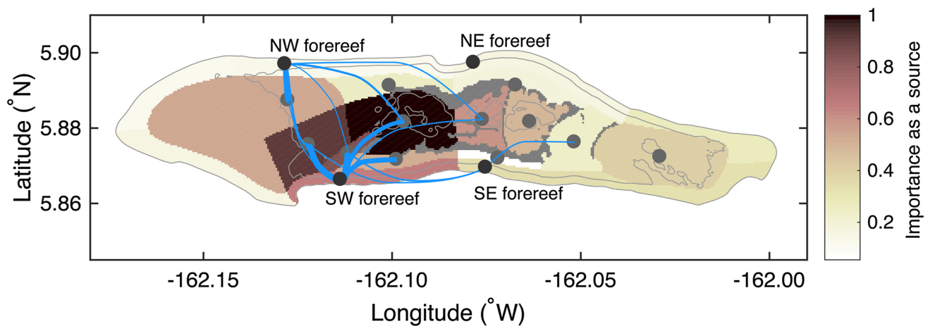
Fig. 3 Major hydrodynamic connectivity pathways between Palmyra's shallow reef terrace (< 10 m depth) and interior lagoon habitats and our four fore reef study sites. Connectivity was evaluated using a previously published wave and hydrodynamic model (ROMS/SWAN), using passive Lagrangian tracer particles and averaged over many model runs with different flow conditions (Rogers et al. 2017). Width of blue arrows indicates strength of connectivity; showing only
