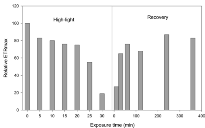
Fig. 3. Relative \text{ETR}_{\text{max}} derived from a series of RLCs during 30-min exposure of a single Pocillopora damicornis polyp to 500 \mu\text{mol photons m}^{-2} \text{s}^{-1} . RLCs were performed at 5, 10, 15, 20, 25 and 30 min exposure. After exposure, recovery (under an irradiance of 50 \mu\text{mol photons m}^{-2} \text{s}^{-1} ) was monitored, with RLCs performed at 10, 30 min, 1, 2, 4 and 6 hr. Relative \text{ETR}_{\text{max}} was plotted against recovery time. Units of relative ETR are \mu\text{mol electrons m}^{-2} \text{s}^{-1} and units of irradiance are \mu\text{mol photons m}^{-2} \text{s}^{-1}
