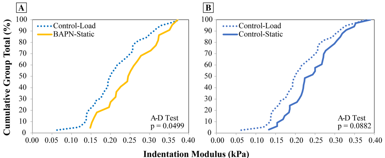
Fig. 5 Cumulative distribution function representation of indentation modulus data. There is a clear shift towards a (a) higher indentation modulus in the BAPN-static group relative to the control-load group
